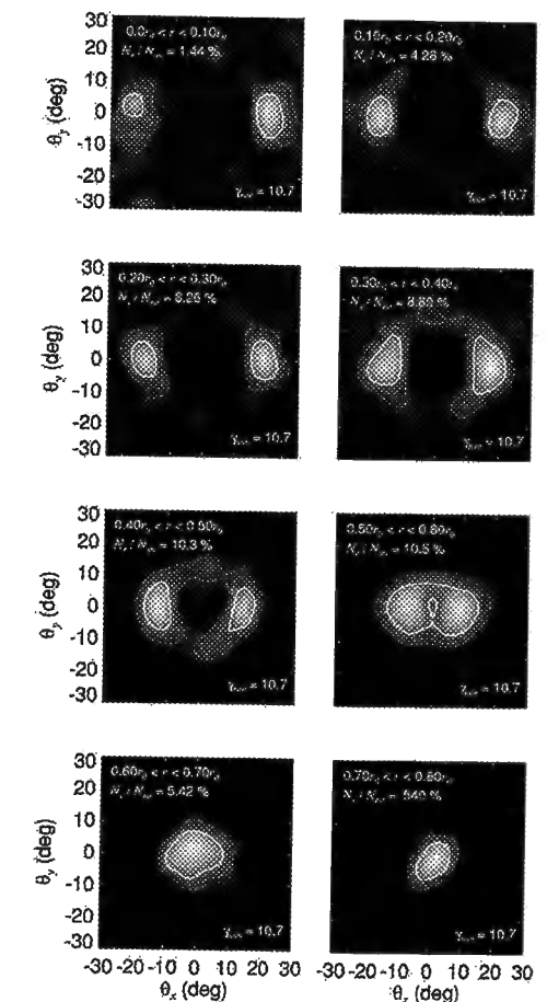
FIG. 15. Each frame shows the angular profile of electrons with final \gamma > \gamma_{\text{min}} = 10.7 emerging from an annulus indicated in the upper left corner. The percentage of the electrons involved is also given. The contour plots are linear and the heavy white contour denotes the 50% level.
