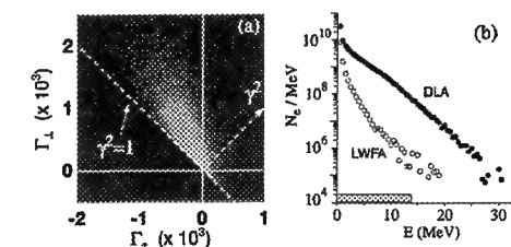
FIG. 6. Breakdown of electron spectrum with respect to the major acceleration mechanism. (a) Distribution of the accelerated electrons in the (\Gamma_z, \Gamma_\perp) space. The shaded histogram is in logarithmic scale. (b) The filled circles represent the DLA spectrum of electrons while the empty circles mark the LWFA spectrum. The bar at the energy axis marks the range of the electron detector used in the experiment (see text for details).
