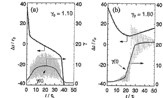
FIG. 11. Variation of the electron-laser pulse distance \Delta z and of the dimensionless electron energy \gamma with time. In the case of energy, the light gray curve is the \gamma(t) variation while the solid line is the same averaged over few bounce oscillations (a) for \gamma_0=1.10 and (b) for \gamma_0=1.80 . The rest of the parameters are as in Fig. 9.
