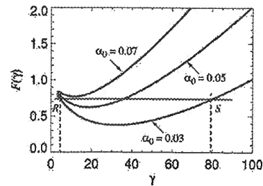
FIG. 5. Variation of F(\gamma) as a function of \gamma for \omega_{b0}/\omega=0.2 , \eta=0.98 and the indicated values of \alpha_0 = v_A^2/(2c^2) .
