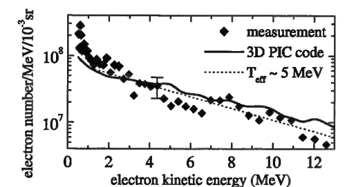
FIG. 1. Typical electron spectrum measured in laser beam direction (diamonds) and exponential fit (dotted line). The prediction of the 3D PIC simulations is also shown (solid line).
