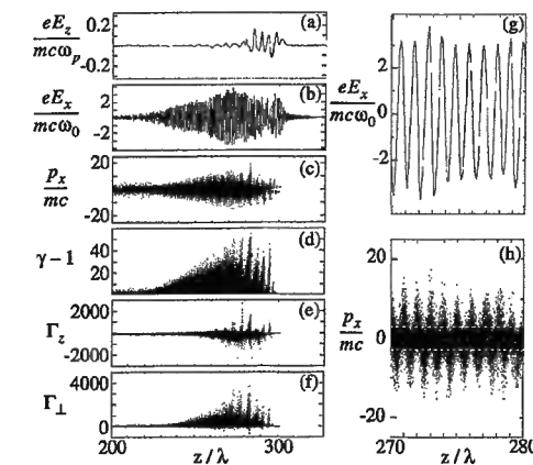
FIG. 5. 3D PIC simulations. The frames show the following: (a) the wake field eE_z/mc\omega_p ; (b) the laser field eE_x/mc\omega_0 , where \omega_0 is the laser frequency; (c) the transverse momentum p_x/mc ; (d) the electron energy distribution \gamma - 1 ; (e) the gain \Gamma_z ; (f) the transverse gain \Gamma_\perp ; all along the laser propagation axis z . Zoom at 270 < z/\lambda < 280 of (g) eE_x/mc\omega_0 and (h) p_x/mc with the dashed line indicating |p_x/mc| = 3 .
