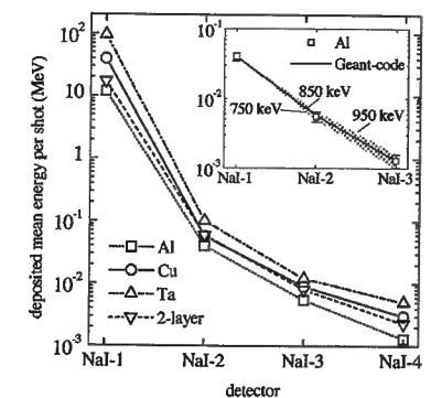
FIG. 3. Mean energy per shot deposited in the four detectors for various Z targets (low-energy threshold 30 keV). Inset: Comparison of the detector response with the prediction of the GEANT code. The shaded area gives an estimate of the temperature determination accuracy corresponding to the statistical error bars of the measurement. All lines shown are to guide the eye.
