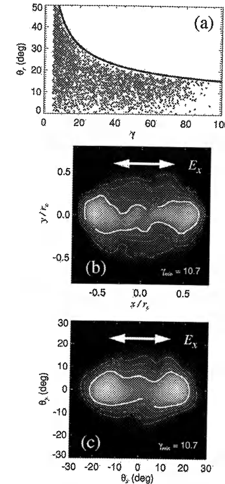
FIG. 14. (a) Distribution of all accelerated electrons to \gamma > 5.0 having initial temperature T_{e0} = 50.0 \text{ keV} in the \theta_r - \gamma space. The maximum angle of emergence for a given final energy is reproduced by the analytical expression for the constant of motion in Eq. (54) (solid line). (b) Spatial distribution of electrons having final \gamma > \gamma_{\text{min}} = 10.7 in the x - y plane after the interaction with the laser pulse is over and (c) the corresponding angular profile of the electron beam. The contour plots are linear and the heavy white contour denotes the 50% level. The double arrow indicates the polarization direction.
