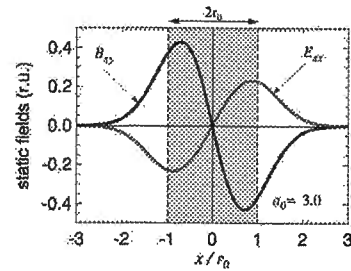
FIG. 1. Static electric and magnetic field profiles; Variation of E_x and B_y with x at y=0 .
