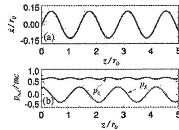
FIG. 2. (a) Trajectory of an electron originating at x=0 , y=0 , z=0 with \vec{p}/(mc)=(0.5,0,0.5) . (b) The variation of p_x/(mc) and p_z/(mc) of the same electron as a function of z/r_0 . The parameters are B_{0\phi}=mc\omega/e=134.0 MG and r_0=2\lambda=1.6 \mu\text{m} .
