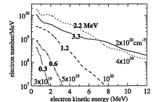
FIG. 2. Experimentally determined electron-spectrum dependence on different electron densities (labeled by normal letters). Bold letters give the effective temperatures of the (not shown) exponential fits.
