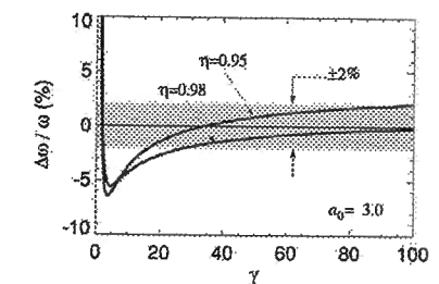
FIG. 12. Dependence of the normalized frequency mismatch on \gamma for \eta=0.95 and \eta=0.98 [see Eq. (25)]. The rest of the parameters are a_0=3 , \omega_c=\omega , and r_0=2\lambda . The shaded region indicates the range of \Delta\omega/\omega for which resonance is attained.
