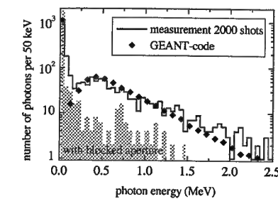
FIG. 2. Pulse-height spectrum for a tantalum target as measured by the second detector NaI-2 (solid line). The shaded area shows the contribution of the scattered radiation. The points depict the prediction of the Monte Carlo code analysis for electrons with 0.9 MeV temperature.
