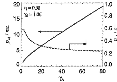
FIG. 4. Dimensionless transverse momentum, p_{xA}/mc (solid line), and velocity, v_{xA}/c (dashed line), of an electron on channel axis ( x=0 ) as a function of dimensionless energy \gamma_A for p_{0x}=0 , \gamma_0=1.06 , and \eta=0.98 .
