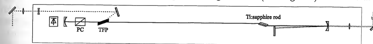
Figure 3.7: Schematic illustration of the regenerative amplifier for initial experiments. The pump light (solid gray line) from the Nd:YLF-laser is focused slightly behind the Ti:sapphire rod. The seed pulses (dotted line) coming from the stretcher are switched in by a Pockels cell (PC) working in combination with a thin film polarizer (TFP). The solid black line shows the beam path of the wave oscillating inside the amplifier cavity. The light leaking through the high-reflective mirrors of the resonator generates an electric signal in a photodiode (PD) positioned behind one of these mirrors. This way, the pulse train oscillating in the cavity is monitored by an oscilloscope (Tektronix TDS2465A, 350 MHz).
