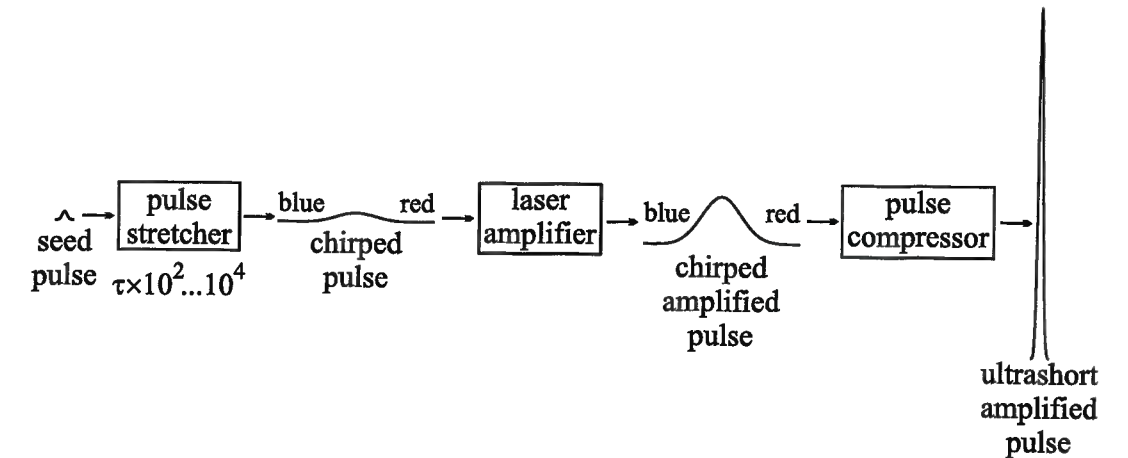
Figure 3.3: Principle of chirped pulse amplification.
