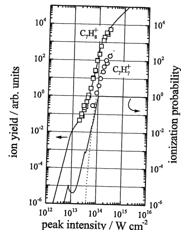
Figure 4.10: Ion yields as a function of peak intensity for 800-nm, 80-fs, linearly polarized laser pulses irradiating gaseous toluene. Squares, parent ion, \text{C}_7\text{H}_8^+ ; circles, fragment ion, \text{C}_7\text{H}_7^+ . The solid line passing through the parent ion data (left ordinate axis) is obtained by volume-integrating the ionization probability that results from the combined action of 6-, 7-, 8-, 9-, 10-, and 11-photon processes (lower solid curve, right ordinate axis). The jumps in the ionization probability curve are the result of channel closing (cf. Fig. 4.9). The dotted line shows the expected effective \text{C}_7\text{H}_7^+ fragment ion yield on the assumption that the internal energy of the toluene cation equals the ponderomotive energy of the electron.
