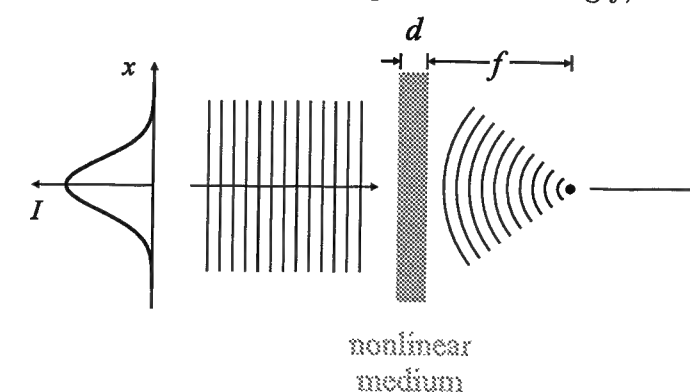
Figure 3.2: Principle of self-focusing. A nonlinear medium exhibiting the Kerr effect of the thickness d behaves as a lens (for paraxial rays) whose focal length f depends on the intensity I of the incident laser beam.
