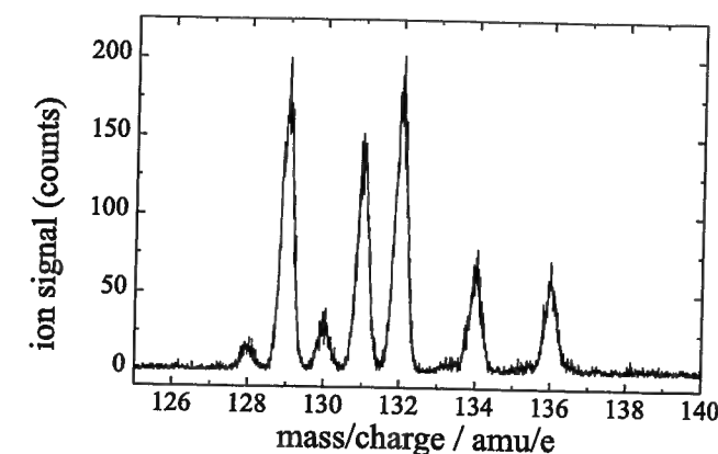
Figure 4.2: Mass spectrum of Xe taken at a pump wavelength \lambda_{\text{pu}} = 266 nm, a probe wavelength \lambda_{\text{pr}} = 800 nm, and I_{\text{pu}} = 8.5 \times 10^8 \text{ W cm}^{-2} , I_{\text{pr}} = 4.3 \times 10^{12} \text{ W cm}^{-2} , for a sample pressure of p = 2 \times 10^{-7} mbar.
