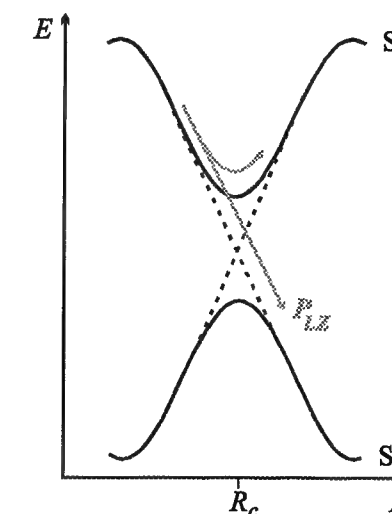
Figure 2.5: Adiabatic picture of two potential energy curves S_0 and S_1 exhibiting an avoided crossing at the critical internuclear distance R_c .
