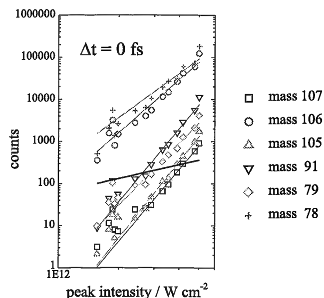
Figure 4.24: Comparison of slopes of ion yields as a function of probe intensity. The data points and the thin solid lines correspond to Fig. 4.20. The thick solid line results from calculating the order of the probe process according to Eq. 4.3 from the fitted width of the response function (see Fig. 4.23 and Tab. 4.5). Obviously, the slope thus calculated does not agree with the experimental data.
