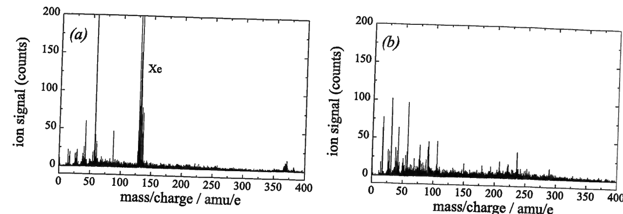
Figure 4.29: Mass spectra of 7-dehydrocholesterol taken under different experimental conditions, (a), \lambda_{pu} = 266 nm, \lambda_{pr} = 800 nm, \tau_{pu} = 99 fs, \tau_{pr} = 93 fs, I_{pu} = 8.5 \times 10^8 W cm -2 , I_{pr} = 4.3 \times 10^{12} W cm -2 , p \approx 1 \times 10^{-7} mbar; (b), \lambda_{pu} = 266 nm, \lambda_{pr} = 400 nm, \tau_{pu} = 99 fs, \tau_{pr} = 86 fs, I_{pu} = 2.0 \times 10^9 W cm -2 , I_{pr} = 6.6 \times 10^{11} W cm -2 , p \approx 1 \times 10^{-7} mbar. In case (a), Xe ( p_{Xe} \approx 2 \times 10^{-7} mbar) is added for calibration. Both spectra are averaged over 150000 sweeps.
