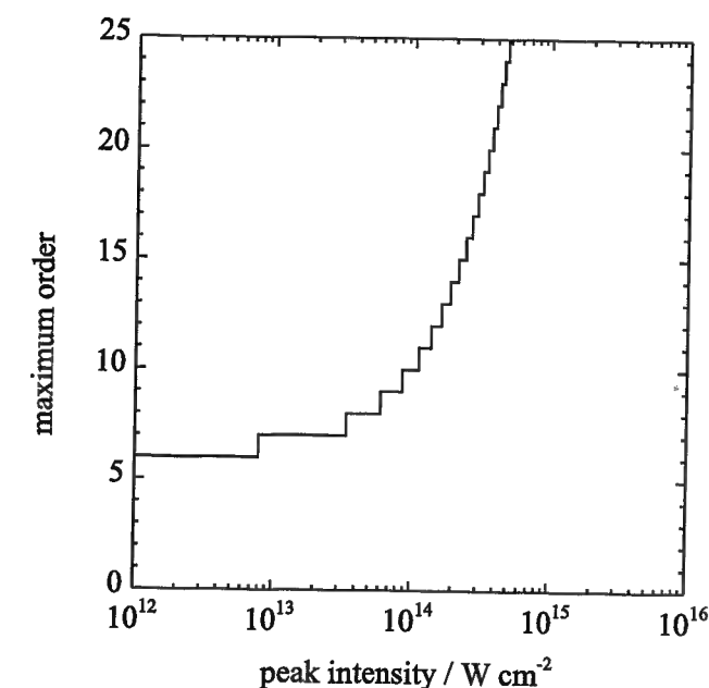
Figure 4.8: Channel closing: highest order expected for an MPI process as a function of peak intensity for gaseous toluene and 800-nm radiation.
