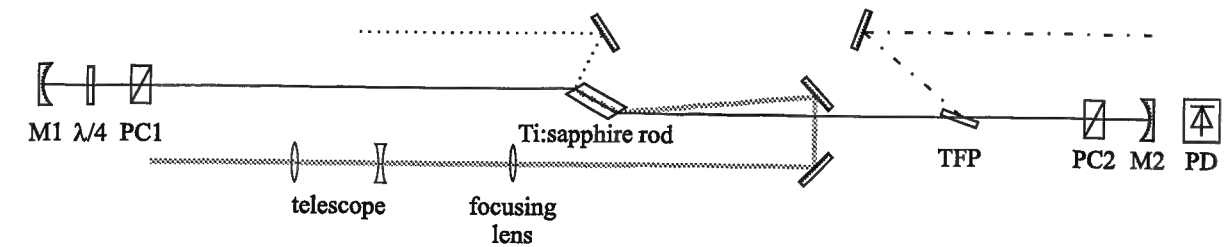
Figure 3.10: Setup of the regenerative amplifier (Spectra-Physics Super-Spitfire). The concave mirrors M1 and M2 form the resonator. The pump beam (solid gray line) collimated by a telescope is focused by a lens slightly behind the Ti:sapphire rod. The seed pulses (dotted line) are vertically polarized and therefore reflected into the cavity by the Ti:sapphire rod cut in the Brewster angle and switched in by the Pockels cell PC1 working in combination with a \lambda/4 -plate. The amplified pulses are switched out by a second Pockels cell (PC2) working in combination with a thin film polarizer (TFP) and then travel to the double-pass amplifier (dash-dotted line). By means of the photodiode (PD) behind M2 connected with an oscilloscope (Tektronix TDS220), the pulse train oscillating in the cavity is visualized.
