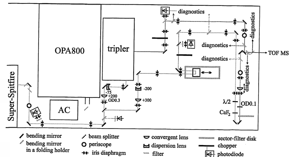
Figure 3.15: Optical setup for pump-probe measurements.
