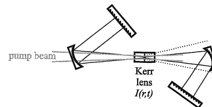
Figure 3.1: Generation of ultrashort pulses in a solid-state laser medium. The optical Kerr effect leads to an intensity-dependent lens in the Ti:sapphire crystal, where only the shortest, i.e. most intense, pulses are allowed to travel inside the cavity (solid lines). Only high intense pulses generate the Kerr lens providing minimized losses, which is the condition for mode-locking to take place.
