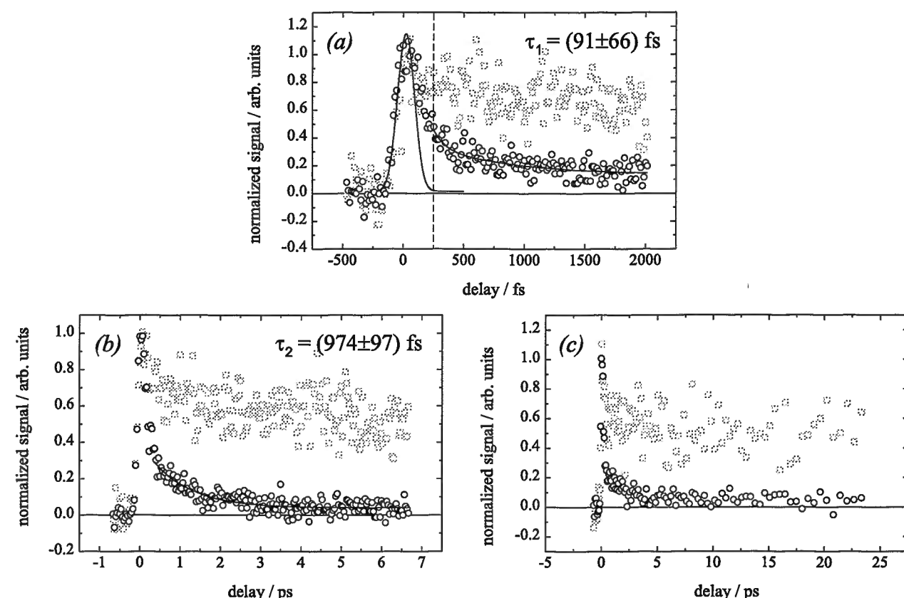
Figure 4.31: Transient ion signals of 7-dehydrocholesterol (gray squares, mass 384; black circles, mass 369) recorded under the same experimental conditions as given in the caption of Fig. 4.29 (a) with different time resolutions in different pump-probe delay ranges ((a), resolution, 13 fs, delay from \sim -0.5 ps to 2 ps; (b), resolution, 33 fs, delay from \sim -0.7 ps to \sim 7 ps; (c), resolution varying from 67 fs to 667 fs, delay from \sim -0.7 ps to \sim 23 ps). In (a) the solid lines represent a Gauss fit and a double-exponential fit, the starting point of which is marked by the dashed line. The solid line in (b) is a single-exponential fit to the data points. Every data point is averaged over 8000 laser pulses.
