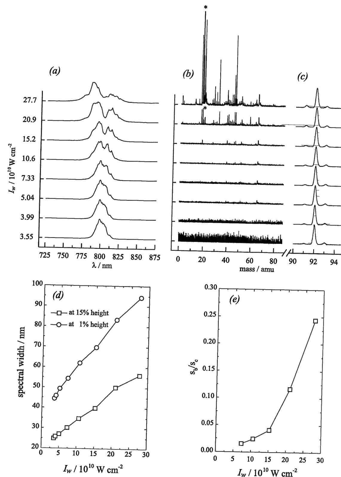
Figure 4.14: Mass spectra of gaseous toluene and corresponding wavelength spectra of the used laser light recorded at different intensities in the \text{CaF}_2 entrance window I_w . (a), recorded wavelength spectra dependent on I_w ; (b) and (c), mass spectra of toluene taken at the same I_w as the power spectra, the \text{H}_2\text{O}^+ peak marked with an asterisk is cut. The part where smaller fragments are expected ( \leq 88 amu/e, panel (b)) is enlarged against the part in panel (c) by a factor of 50. (d), spectral broadening as a function of I_w ; (e), ratio of integrated fragment peaks (from panel (b)) to integrated peaks (from panel (c)) occurring also with Fourier-limited pulses as a function of I_w .
