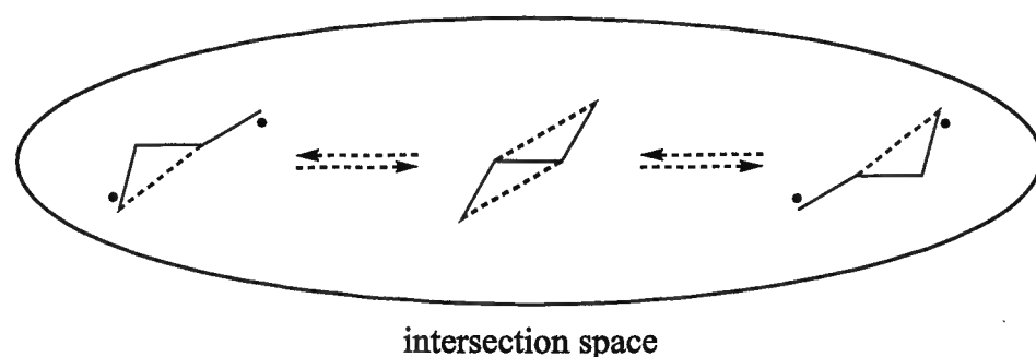
Figure 2.8: Typical geometrical properties of molecular substructures conical intersections playing an essential role in polyene photochemistry [53–55].
