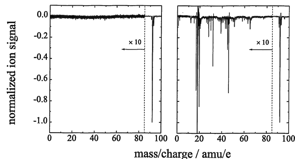
Figure 4.15: Comparison of two mass spectra of the toluene molecule. Although the left spectrum is recorded at an even higher intensity at focus ( 1 \times 10^{14} \text{ W cm}^{-2} ) than the right one ( 6 \times 10^{13} \text{ W cm}^{-2} ), strong fragmentation is only observed in the latter. Obviously, this is a result of the different peak intensities to which the \text{CaF}_2 entrance window is exposed (left spectrum, I_w = 7 \times 10^{10} \text{ W cm}^{-2} ; right spectrum, I_w = 3 \times 10^{11} \text{ W cm}^{-2} ).
