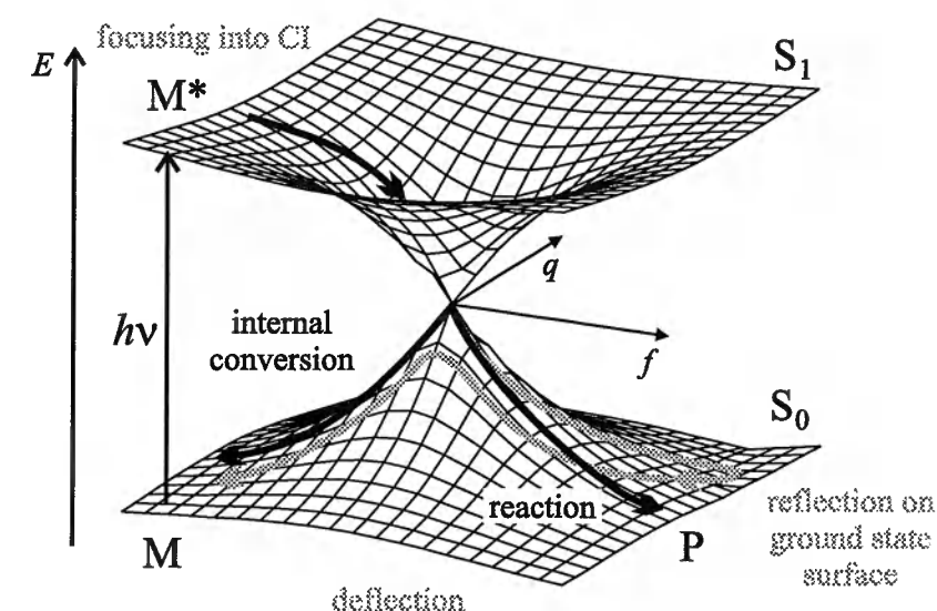
Figure 2.12: Fundamental processes occurring at a conical intersection. The two promoting modes correspond to the coordinates f and q extending the branching space. During the unimolecular photochemical reaction, the molecule M reaches the excited state S_1 from the ground state S_0 by absorption of light and forms the excited molecule M^* . In the vicinity of a conical intersection, the wavepacket is focused into the funnel of the conical intersection. After passing it, the wavepacket contains a lot of vibrational energy from the upper state, causing a reflection on a rising area of the ground state surface sooner or later. This can be prevented by including a third mode for energy dissipation. This way, the molecule can form the product(s) P (reaction), or relax to the ground state as M once more (internal conversion).
