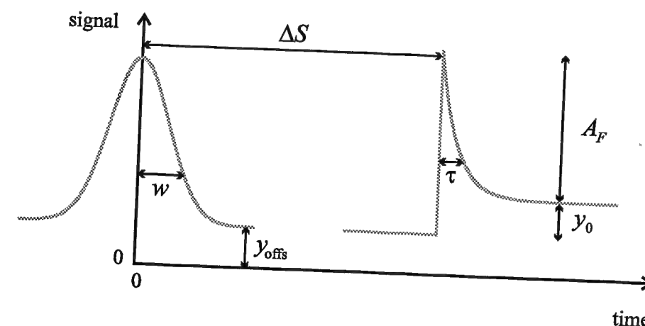
Figure 4.3: Illustration of the components of the fit function (Eq. 4.1) used for the evaluation of time-dependent data (left curve, response function; right curve, exponential decay).
