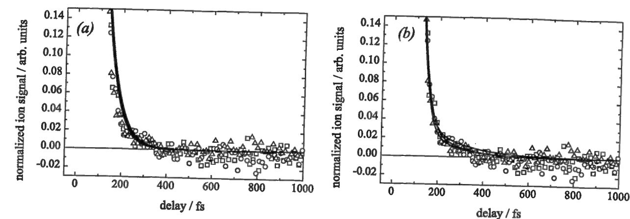
Figure 4.23: Expanded view of time-dependent signals of the 1,3,5-cyclooctatriene parent ion. The three data sets are identical in both panels. Each solid line represents a fit to one of these data sets (squares, circles and triangles) applying the same fit function given in Eq. 4.1 to all, but different numbers of free parameters. In (a) the width of the response function determined before is inserted as a fixed parameter. In (b), however, this width is treated as an additional free parameter in the fitting procedure.
