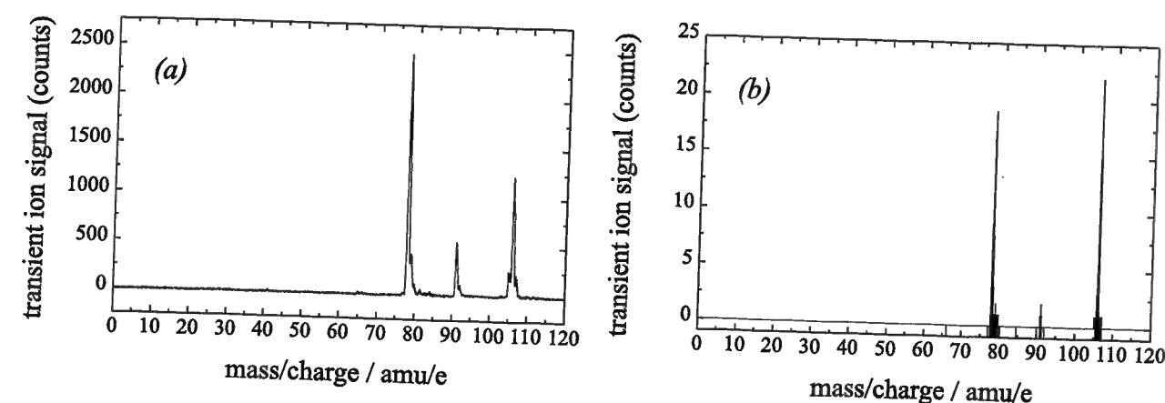
Figure 4.26: Comparison of transient mass spectra of 1,3,5-cyclooctatriene taken at different probe wavelengths ((a), NIR; (b), UV) under the experimental conditions described in the caption of Fig. 4.25.
