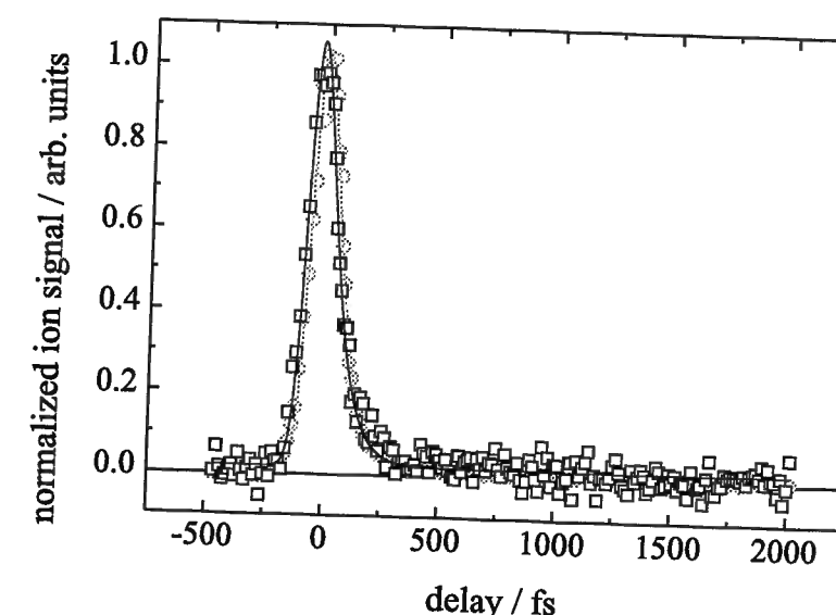
Figure 4.25: Comparison of transient signals of the 1,3,5-cyclooctatriene fragment with mass 78, exemplarily illustrated. Black squares, \lambda_{pu} = 265 nm, \lambda_{pr} = 401 nm, \tau_{pu} = 88 fs, \tau_{pr} = 80 fs, I_{pu} = 3.9 \times 10^8 W cm ^{-2} , I_{pr} = 2.2 \times 10^{11} W cm ^{-2} , p = 1.0 \times 10^{-7} mbar; gray circles, \lambda_{pu} = 265 nm, \lambda_{pr} = 802 nm, \tau_{pu} = 93 fs, \tau_{pr} = 104 fs, I_{pu} = 1.7 \times 10^8 W cm ^{-2} , I_{pr} = 2.9 \times 10^{12} W cm ^{-2} , p = 7.2 \times 10^{-8} mbar. The solid lines representing fits to the data are described in the text.
