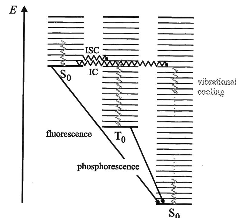
Figure 2.14: Fundamental processes of interstate relaxation. The abbreviation ISC stands for intersystem crossing, and IC for internal conversion. The wavy lines correspond conventionally to non-radiative processes.
