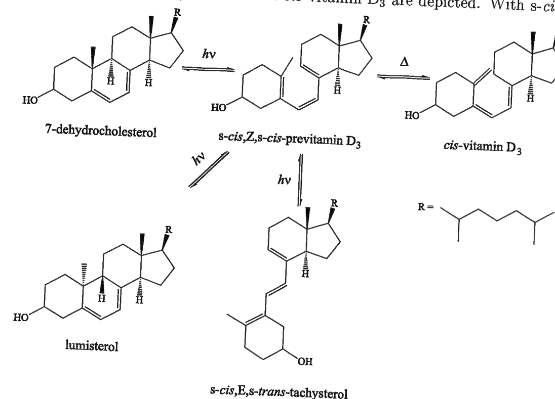
Figure 4.32: Reaction scheme of vitamin D 3 synthesis with side reactions induced by UV light. previtamin D as the reactant, the following photoreactions can take place: ring closure leading to 7-dehydrocholesterol or lumisterol and double bond (Hula twist) cis-trans isomerization (see Sec. 2.1.2) to form s-cis,E,s-trans -tachysterol.
