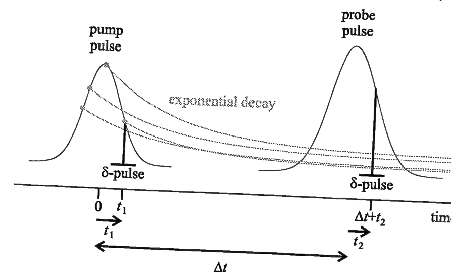
Figure A.1: Illustration of the time variables used for the derivation of the fit function of Eq. 4.1. each \delta -pulse contributes to the excitation probability P_{pu} (to the order of 1) and induces the photochemical reaction and the concomitant (exponential) decay of the signal at every point in time within the pump pulse. This leads to a smearing out of the begin of the reaction in the measurable signal. The time-dependent excitation function f(t) can be expressed as:
