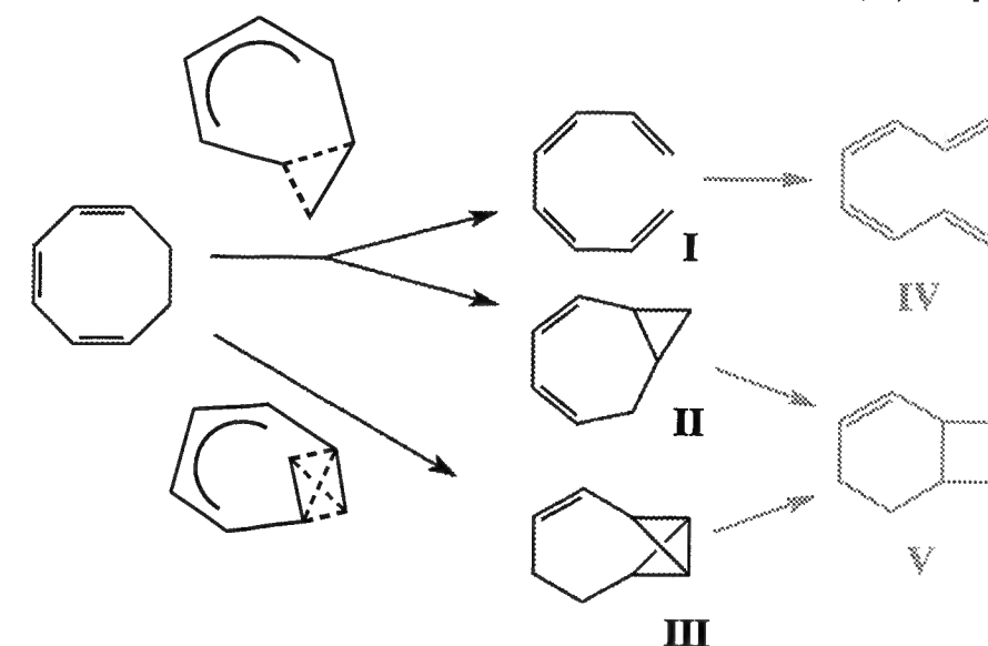
Figure 2.15: Photoinduced electrocyclic ring opening of 1,3,5-cyclooctatriene proceeding via conical intersections.
