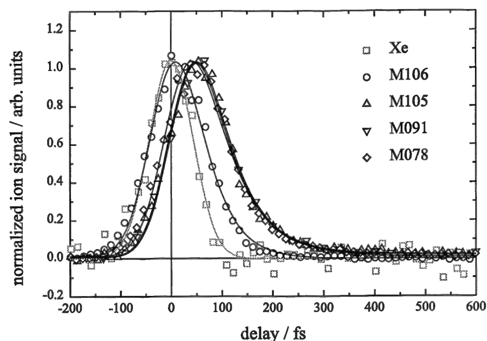
Figure 4.22: Normalized transient signals of the parent ion and all measurable fragment masses of 1,3,5-cyclooctatriene as a function of the pump-probe delay, taken at \lambda_{pu} = 265 nm, \lambda_{pr} = 802 nm, \tau_{pu} = 93 fs, \tau_{pr} = 104 fs, I_{pu} = 1.7 \times 10^8 W cm ^{-2} , I_{pr} = 2.9 \times 10^{12} W cm ^{-2} , p = 7.2 \times 10^{-8} mbar. The Xe signal indicates \Delta t = 0 fs. The solid lines are fits using Eq. 4.1.
