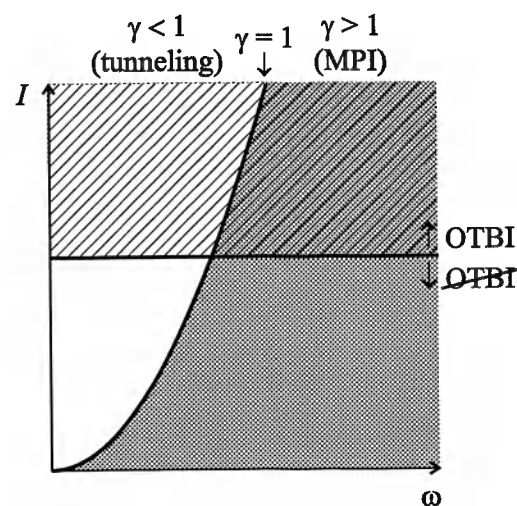
Figure 2.23: Different ionization regimes as a function of laser intensity and laser frequency. The Keldysh adiabaticity parameter divides the plot into MPI and tunneling ionization regimes. The onset of OTBI depends only on laser intensity, independent of frequency (cf. [101,102]).
