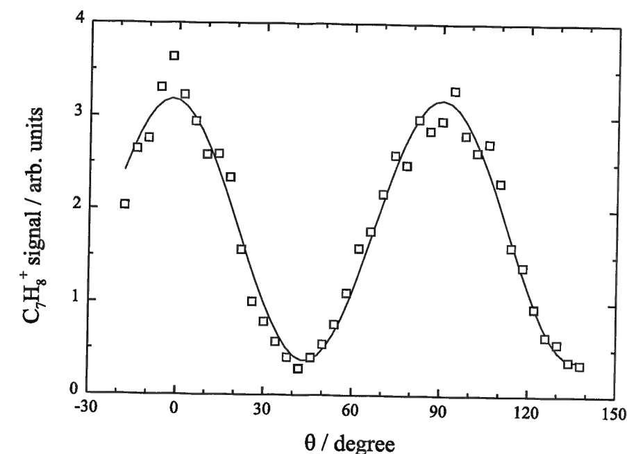
Figure 4.13: Parent ion yield as a function of the ellipticity for 800-nm, 80-fs, laser pulses irradiating gaseous toluene, for a fixed peak intensity of 8.5 \times 10^{13} \text{ W cm}^{-2} , measured by varying the angle \theta between the fast axis of the quarter-wave plate and the polarization direction of incoming linearly polarized light (see text).
