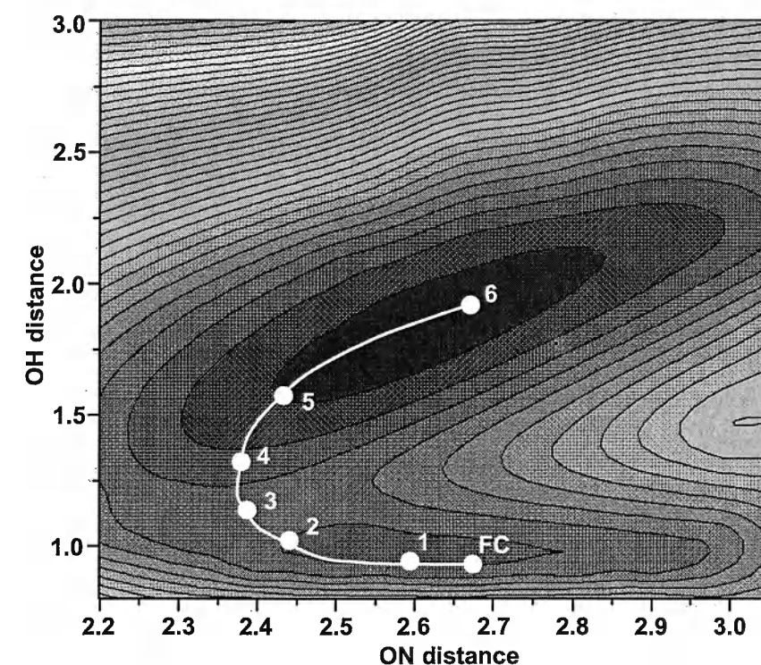
Figure 2.3: The 2-D S_1 reaction surface predicted for the ESIPT of HBT [9]. Ab initio calculations proved the ON and OH-distance (in Å) to be the relevant coordinates for describing the H-transfer. The reaction path (white line) connects the FC-region to the K^* configuration close to structure "6", passing the transition state "3". NMA results for the points FC, 1, 3, 5, and 6 follow in Chapter 2.3.
