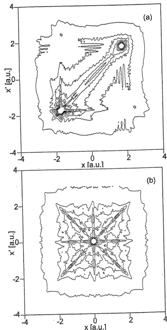
Figure 4.2: Contour plots of two kernel matrices A in the double well system. Comparable features can be observed for the Morse potential also. Panel (a) shows configuration H and panel (b) configuration T. The numerical values for the matrix entries range from \sim 10^3 on the diagonal to \sim 10^{-8} on the boundaries. The contour levels correspond to: 1 (outer line), 31, 61, \dots , 211.
