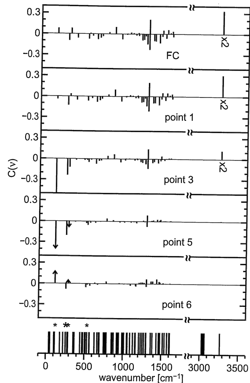
Figure 2.5: NMA with solution coefficients C(\nu) along the reaction path with respect to the K^* equilibrium structure. The computed normal mode frequencies are given in the bottom row for comparison. Stars point out modes that are close to the experimentally observed frequencies. In the keto modes system these are (\nu_{\text{ex.}}, \nu_{\text{theo.}}) : (118 \text{ cm}^{-1}, 114 \text{ cm}^{-1}) , (289 \text{ cm}^{-1}, 288 \text{ cm}^{-1}) , (529 \text{ cm}^{-1}, 533 \text{ cm}^{-1}) , and the experimentally strongest signal at (254 \text{ cm}^{-1}, 258 \text{ cm}^{-1}) , marked by a larger star. Compare to Fig. 2.4 and the text for details.
