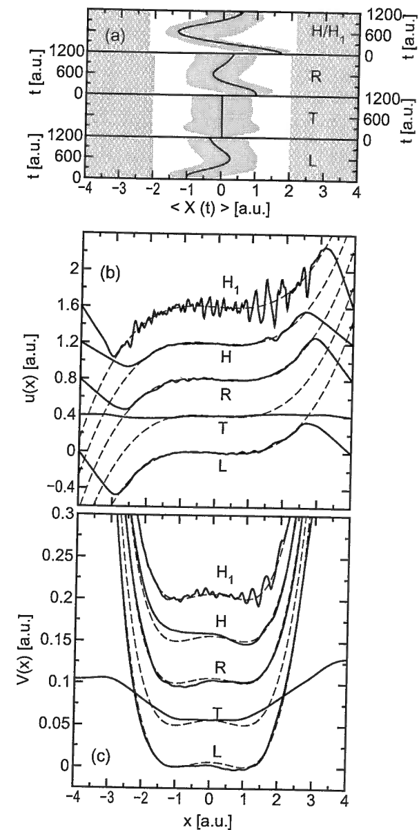
Figure 5.3: Extractions of the potential under the conditions given in table 5.1. Panel (a): The time evolution of the position average \langle x(t) \rangle accompanied by the left- and righthand normalized variances (i.e., the shaded areas determined by Eqs.(5.7) and (5.8)) to indicate the regions predominantly covered by the probability densities. The grey domains on the extreme left and right mark classically forbidden areas (cf. table 4.1). Panel(b): The reconstructed gradient u(x) and the corresponding potential V(x) in panel (c). For comparison the exact solutions are included as dashed lines. The individual curves have been offset for graphical reasons and the presentation of V(x) is restricted to |x| \lesssim 2.5 since the boundary regions will not be extracted correctly due to the lack of data sampling there.
