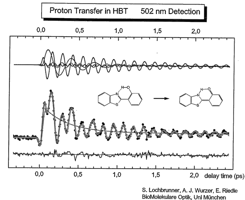
Figure 2.1: Time resolved transmission change (dots, center) for a 20 fs probe pulse at 502 nm induced by ESIPT after an excitation at 347 nm. In combination with the exponential decay (magenta) the remaining signal can be perfectly reproduced (grey line, center) with four low frequency modes 118\text{ cm}^{-1} , 289\text{ cm}^{-1} , 529\text{ cm}^{-1} , and a dominant contribution at frequency 254\text{ cm}^{-1} (top part). Only a negligible residuum remains (lowest curve).
