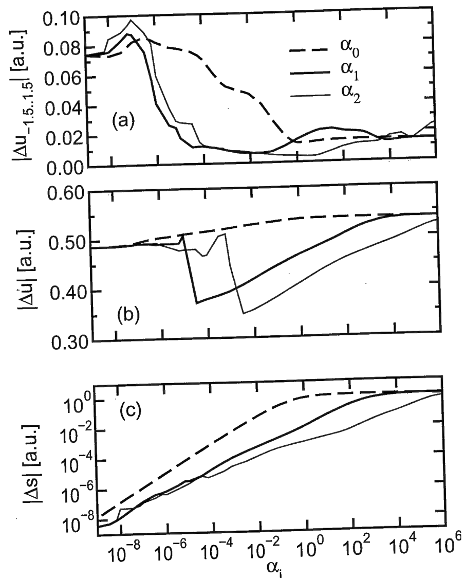
Figure 5.2: \alpha_i parameter scan performed with malonaldehyde configuration L. The two top panels display |\Delta u| with respect to the inversion range -1.5 \leq x \leq 1.5 in (a) and -4 \leq x \leq 4 in (b). Panel (c) explores the system defect |\Delta s| .
