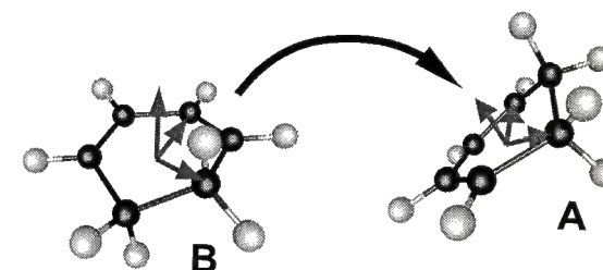
Figure B.1: CHD subject to translation and rotation apart from internal degrees of freedom.
