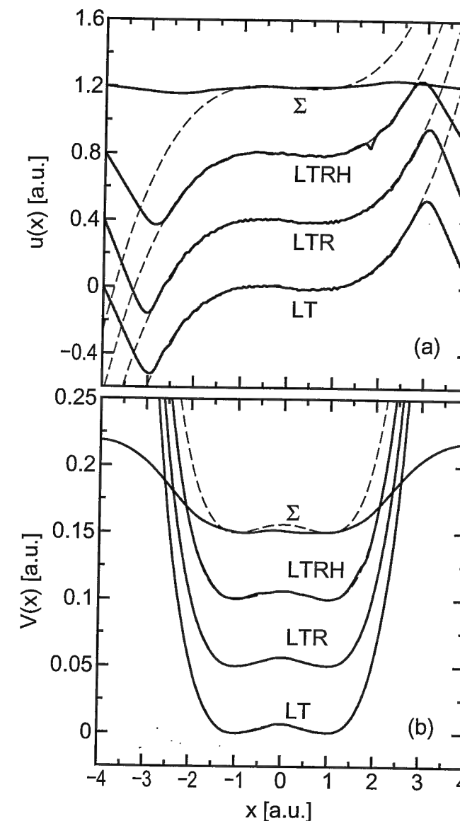
Figure 6.1: Extraction of PES for optimally combined (LT, LTR, and LTRH) as well as \rho -combined data ( \Sigma ). See the text and table 5.1 for further details. The curves for the potential's derivative u(x) in (a) and the PES in (b) have been offset for graphical clarity and exact solutions (dashed lines) added for comparison. For several optimal combinations of the data the original and reconstructed PES are almost indistinguishable.
