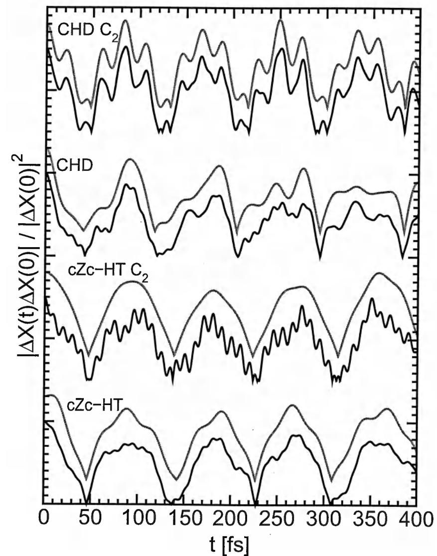
Figure 1.11: Similar to Fig. 1.10 but this time \Delta X(t) is compared to the initial excursion \Delta X(0) . Colored lines again represent vibrations dictated by the few fingerprint modes selected in the tables 1.1a and 1.1b.
