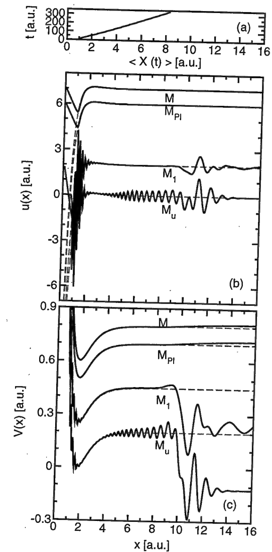
Figure 5.5: Extractions of the Morse potential with \alpha_1 regularization (see table 5.2). (a) area covered by the wavepacket motion 1 \lesssim x \lesssim 8 illustrated by the time evolution of the average position \langle x(t) \rangle . (b) reconstructed u(x) and the corresponding potential V(x) in (c). The individual curves have been offset for graphical clarity and exact solutions (colored dashed lines) were added for comparison. An additive constant was suitably chosen for V(x) to make exact and reconstructed curves coincide. M : optimal \alpha_1 -parameter chosen according to Fig. 5.4a; M_{PI} : employing partial integration for b(x) (cf. Appendix D.1); M_1 : \alpha_1 -parameter chosen for the too large inversion domain in Fig. 5.4b; M_u : unregularized inversion.
