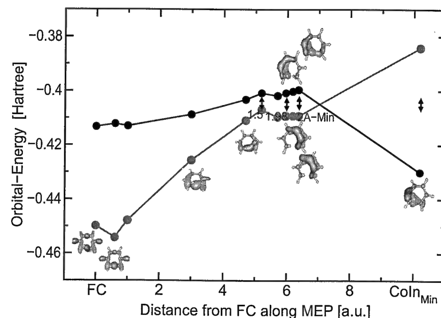
Figure 1.6: MOs 20 and 21 along the full minimum energy paths connecting the FC region on the S_2 -surface with CoIn_{Min} on the S_1 -surface (cf. [37]). Distances on the abscissa refer to this full MEP. Arrows point to structures selected for NMA and the corresponding labels refers to those employed in the text and in subsequent figures. All orbitals were evaluated with a 6-31G* basis set with GAUSSIAN94 [23]. See the text for further details.
