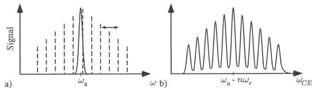
Figure 2.6: Linear (single photon) spectroscopy with a comb. Panel a) shows the response of the atom to a single frequency (solid) and the comb spectrum (dashed) that can be shifted by tuning the offset frequency. Panel b) gives the atomic response as a function of the carrier envelope frequency. For a linear response of the atom this spectrum is just the convolution of atom response and comb spectrum.
