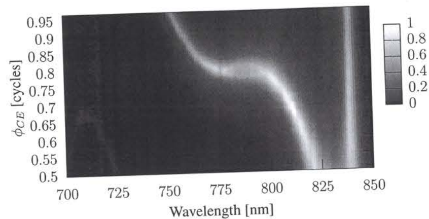
Figure 4.12: Spectrally resolved transmission of the resonator through one of the high reflecting mirrors as a function of the driving lasers pulse to pulse phase shift \phi_{CE} . The transmission data was normalized by the driving laser spectrum to improve the visual display. This normalization is not necessary for analysis.
