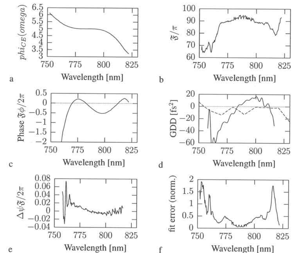
Figure 4.14: Results from fitting the transmission data with model (4.6). (a) The center of the fringe \phi_{CE}(\omega) , (b) The resonator finesse (divided by \pi ) as calculated from the fitted round trip gain r using (3.34), (c) The effective round trip phase \psi(\omega) from expression (3.75), where the unknown constants \phi'_{CE} and \psi(\omega_{fix}) were chosen such that the spectrum in figure 4.10 would be the result. (d) Second derivative of \psi(\omega) obtained like this. To get a nice plot the data phase data was low pass filtered with a cutoff frequency of about 1.5 THz, corresponding to a resolution of about 3 nm. (e) The phase rejects of the smoothing low pass filter. As this is small compared to the relevant scale for this resonator, no important information is removed by the filter. (f) square sum of the residuals of the fit normalized to the fitted model integral. The fit become less accurate in the wings of the spectral range covered.
