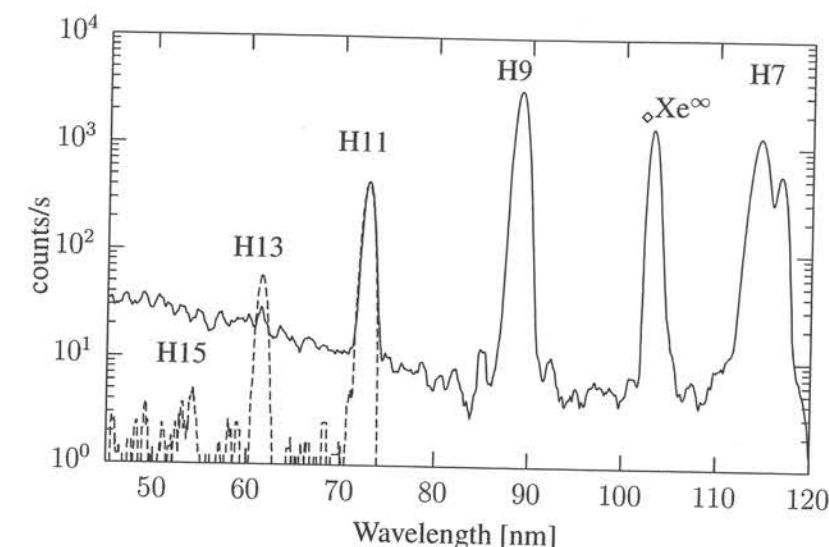
Figure 4.19: Typical harmonic spectrum observed. In solid is the signal observed, when looking directly into the output beam, while the dashed curve is taken with a 1000 Å thick aluminum foil with an absorption edge just below 90 nm in the beam path. This filters away the strongest components in order to reduce the stray light that would otherwise bury the weaker peaks. The dashed signal has been rescaled to have the same magnitude at the 11 th harmonic. The harmonics are labeled Hx, and the ionization limit is marked by a point labelled Xe ∞ .
