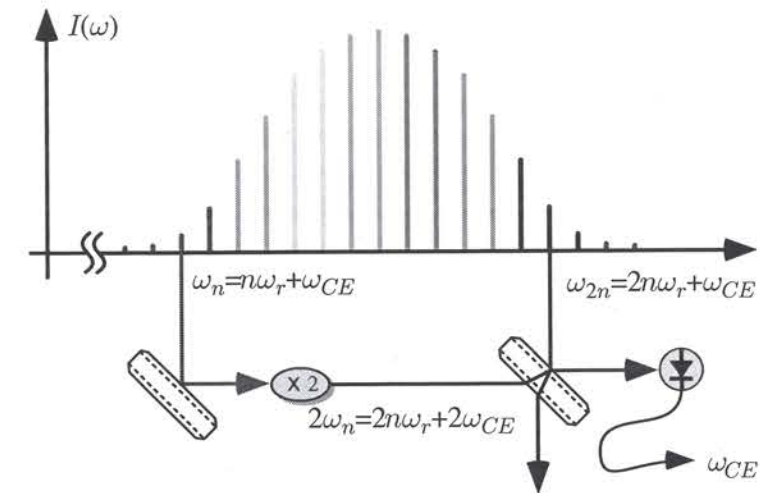
Figure 2.3: Self-referencing technique. A mode from the low frequency side of the comb is frequency doubled and compared to a mode from the high frequency end. Like this the absolute frequency of the low frequency mode, and therefore all modes can be determined via two radio frequencies \omega_r and \omega_{CE} and a large integer n .
