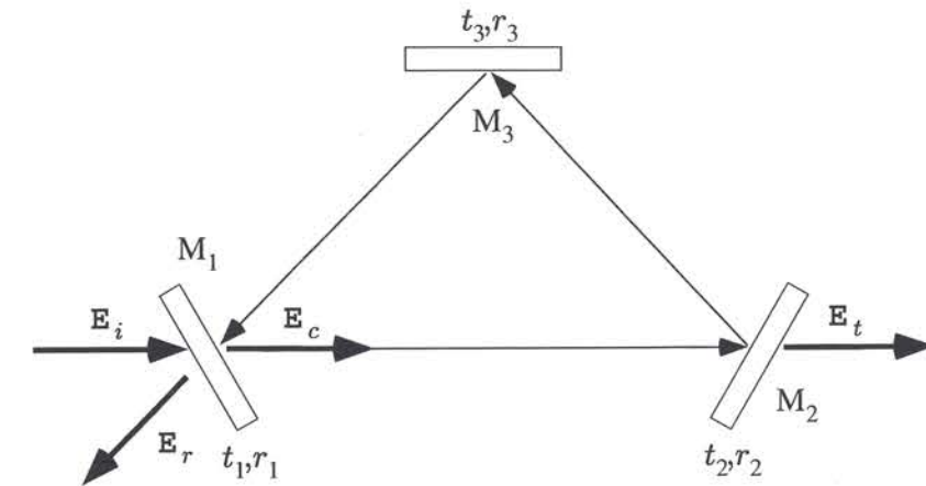
Figure 3.6: Sketch of a typical optical resonator. The incident electric field E_i is coupled to the resonator through a input coupler M1 with complex transmission amplitude t_1(\omega) and reflection amplitude r_1(\omega) . Circulating field E_c , reflected field E_r and transmitted field result from the driving incident field.
