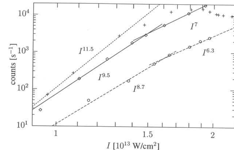
Figure 4.20: Power scalings of different features in the spectrum. Diamonds indicate values for H9, circles correspond to H11 and crosses to Xe ^{\infty} . Lines are power law fits to H9 (solid) data with exponents 9.5 and 7, H11 (dashed) with exponents 8.7 and 6.3, and to Xe ^{\infty} (dash dot) with exponent 11.5. Saturation of the Xe ^{\infty} feature is observed for high intensities.
