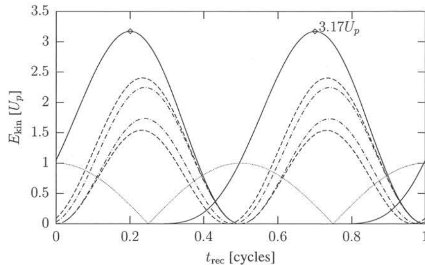
Figure 3.4: Kinetic energy of the returning electron as a function of return time for trajectories shorter than an optical cycle (solid), between one and two (dashed), and between two and three optical cycles (dash-dotted). This shows the instantaneous spectral distribution of the generated field (for a finite time window). The strongest contribution comes from the trajectories shorter than an optical cycle. The dotted line is proportional to the electric field at the time of recombination.
