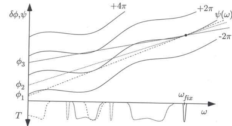
Figure 3.14: Illustration of the meaning of equation (3.75). On the positive vertical axis the left hand side (i.e. \psi(\omega) - 2j\pi ) of (3.75) is plotted in black and the right hand side is shown for different values of the intercept \delta\phi = k\phi_{CE} - \phi'_{CE} is shown in grey, dotted and dash-dotted respectively. On the negative vertical axis a sketch of the corresponding relative transmission T of the resonator is shown with corresponding line styles. Maxima in T are observed where the right and left hand side coincide.
