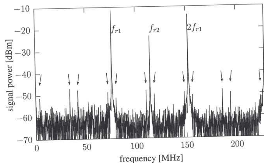
Figure 4.23: RF spectrum of the signal from the photomultiplier tube. f_{r1} marks the repetition rate of the Nd:YVO 4 laser (76 MHz), f_{r2} the repetition rate of the HHG system (114 MHz) and arrows mark the beat signals between the two frequency combs with respective repetition rates.
