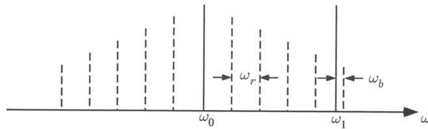
Figure 2.1: Determining the frequency gap between a carrier with frequency \omega_0 and a second signal at \omega_1 . The dashed lines depict the sidebands, which arise from periodically modulating the carrier at \omega_0 with a period T = 2\pi/\omega_r . An interference between the modulated carrier and the signal at \omega_1 will now exhibit beat signals with all of these sidebands, the smallest being \omega_b . The gap is then given by (2.5).
