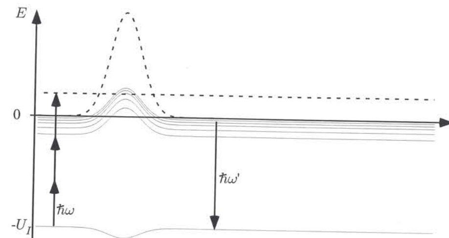
Figure 4.25: Process leading to the \text{Xe}^\infty feature at 103 nm. The high-lying Rydberg states are resonantly excited during the pulse (dashed peak) by a multi photon (3 photons in this sketch, in xenon this would be 8 in our case) process that is shifted into resonance by the AC-Stark effect. The excited dipole radiates for a long time so that most of the emission is at the unperturbed frequency.
