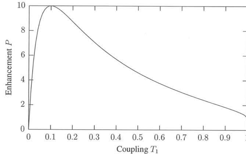
Figure 3.8: Enhancement factor in a resonator with a loss of 10% per round trip, i.e. a value of r_r^2 = 0.9 .
