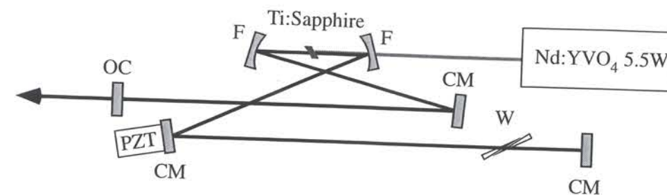
Figure 4.2: Schematic of the laser system. Nd:YVO 4 : frequency doubled pump laser 5.5 W at 532 nm, Ti:Sapphire: laser gain medium, F: focusing mirrors 25 mm focal length, CM: chirped plane mirrors, OC: output coupler, PZT: piezoelectric transducer for controlling resonator length, W: fused silica wedges to control the carrier envelope offset frequency.
