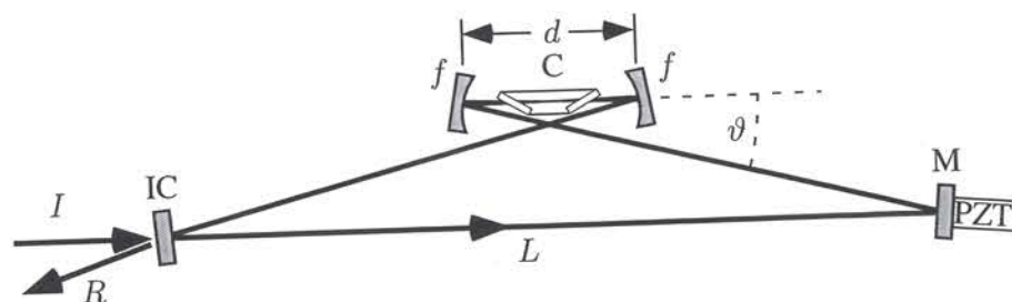
Figure 4.4: Sketch of the bowtie resonator design. A ring resonator with a long "collimated" arm of length L (starting from the left focusing mirror f through mirror M and IC to the right focusing mirror) and a "focused" arm of length d between the two focusing mirrors with focal length f . The folding angle between the focused and collimated arm is \vartheta . IC is the input coupler through which the driving field is coupled to the resonator. M is a piezo (PZT) mounted mirror to control the resonator length electronically. Note that there is also a reflected beam R from IC in addition to the driving beam I , which is used to create an error signal for the electronic feedback. The target is placed in the focused arm. Frequently this is a nonlinear medium for second or third harmonic generation. In our case it is a vacuum chamber that contains the nonlinear medium and is sealed by Brewster windows.
