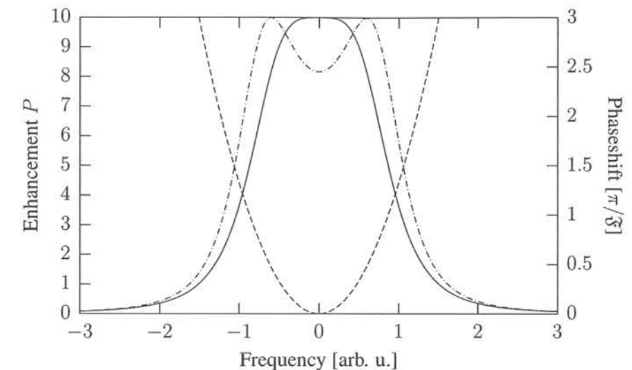
Figure 3.9: Enhancement (solid) of a tuned comb in a resonator with r = 0.9 , effective round trip phase shift (dashed) and enhancement for a slightly shifted phase (dash-dotted) so that the enhanced range is broader. This illustrates that setting \delta\omega_r = \delta\omega_{CE} = 0 may be not the only sensible choice.
