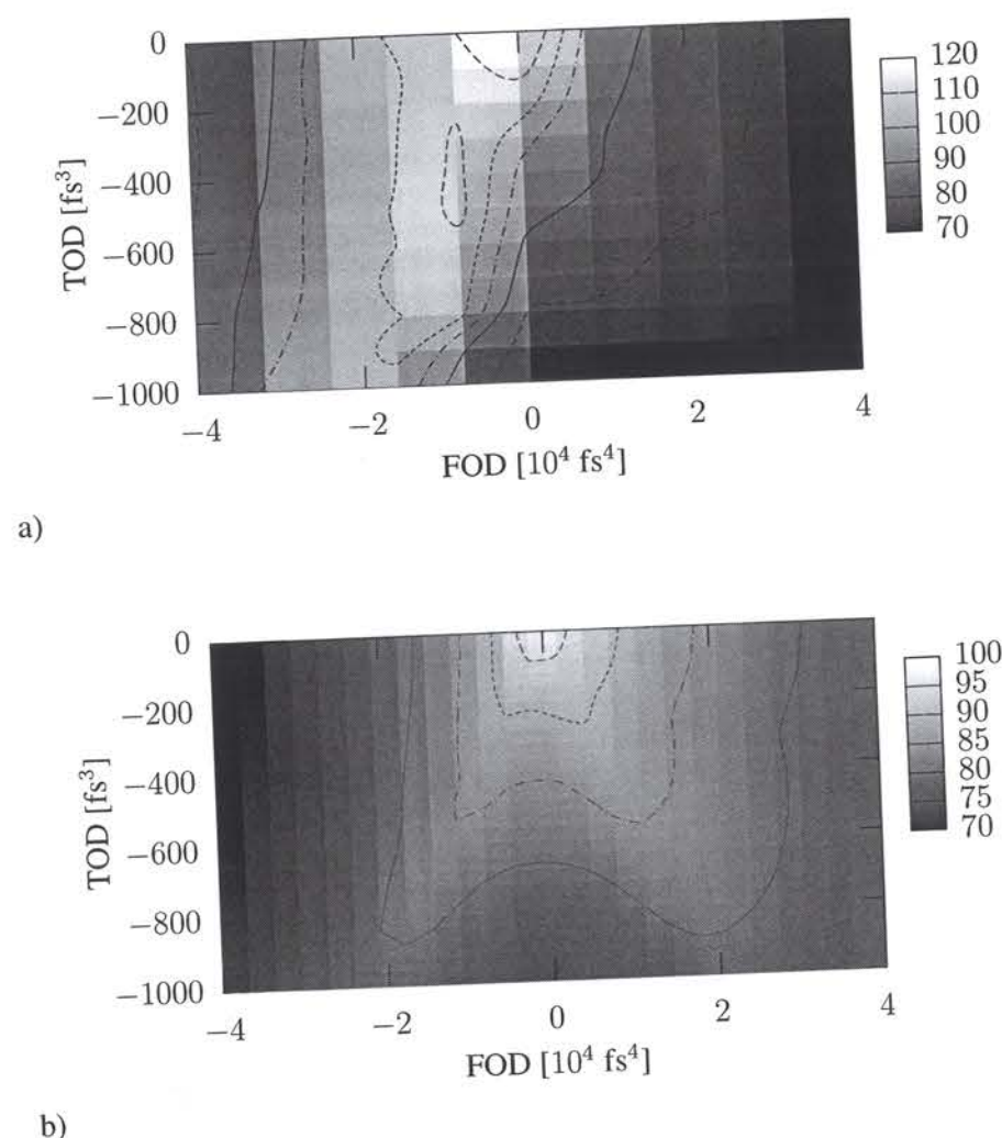
Figure 3.22: Optimized peak powers for the a) nonlinear and b) the linear case. The area including an peak power enhancement factor of 95 or larger, is clearly larger in the nonlinear (dash-dotted contour) than in the linear case (long dashes). Also remarkable is the fact that in the nonlinear case the circulating peak power can be higher than in the linear case.
