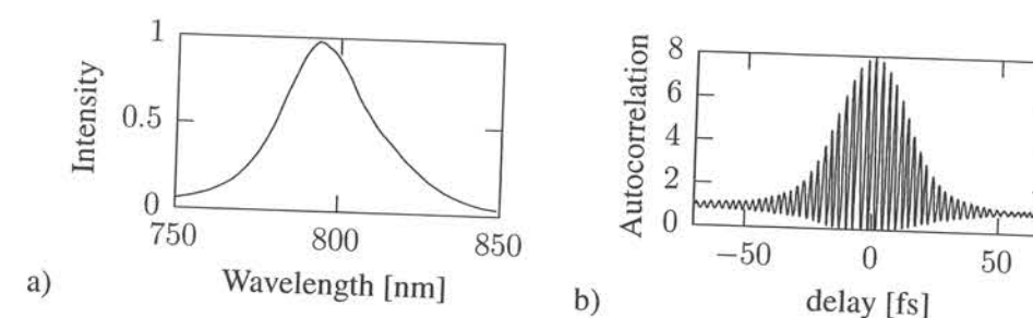
Figure 4.3: a) Typical output spectrum of the laser system with a FWHM width of 30 nm centered at 795 nm. b) Measured interferometric autocorrelation trace corresponding to a pulse duration of about 20 fs.
