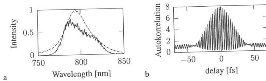
Figure 4.10: a: Locked resonator spectrum (solid) and driving laser spectrum (dashed), b: measured intracavity second-order autocorrelation shows a nearly Fourier limited pulse corresponding to 28 fs pulse duration if a sech pulse shape is assumed.
