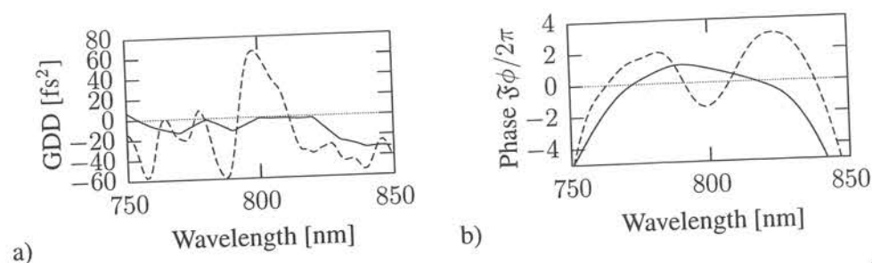
Figure 4.7: Round trip a) GDD and b) phase for the resonator (2.671 m air, 2.3 mm sapphire, one LA3, two LA5, three LA10 and two LA11) that was built during this work. Solid lines show the sum of the design curves and dashed is the sum of measured dispersion properties. The finesse assumed for scaling the phase is \mathcal{F} = 100\pi .
