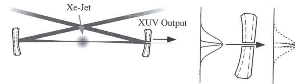
Figure 4.15: Schematic for hole coupling in a resonator. A small aperture at the center of one cavity mirror transmits the narrow XUV beam while most of the wider fundamental is reflected.
