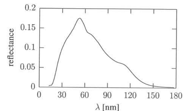
Figure 4.16: Fresnel reflectance of sapphire for p-polarized radiation at an incidence angle of 60.4^\circ (Brewster's angle for 800 nm), determined using tabulated refractive index data from Palik (1991).
