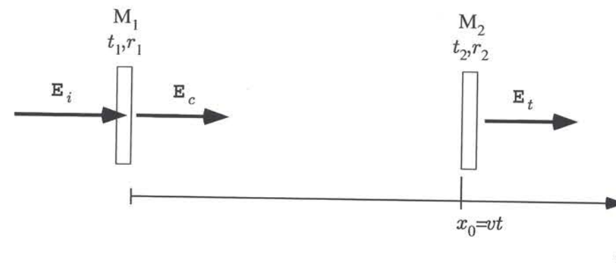
Figure 3.17: Simplified scheme of a scanning Fabry-Perot cavity with incident wave E_i , that gets transmitted through mirror M_1 with transmission t_1 and reflection r_1 , circulating wave E_c that bounces back and forth between the mirrors and gets transmitted through mirror M_2 , which moves at velocity v . E_t : transmitted wave.
