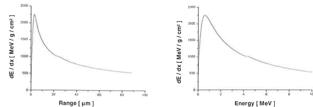
Figure 5.3: Energy loss dE/dx for alpha-particles in CR-39. The highest energy loss occurs at the end of the range at low energies, shortly before the particle is stopped.
