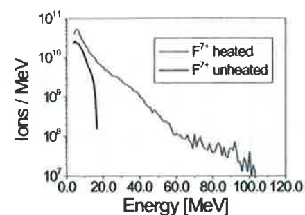
Figure 6. Heavy ion acceleration in the presence (unheated) and without (heated) proton contaminants. More than 100 MeV (5 MeV/nucleon) F^{7+} ions were measured.
