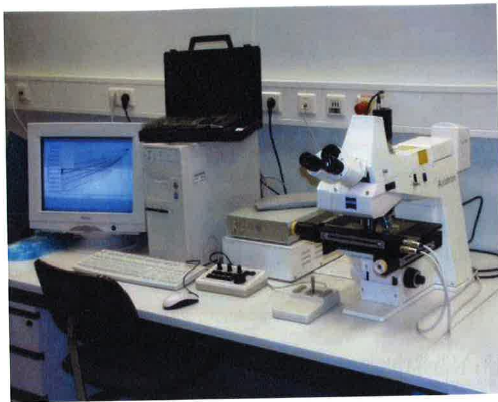
Figure 5.6: Automated scanning and particle counting station: The CR-39 detectors are placed under a computer controlled microscope. A CCD-camera relays the image to the computer where a special pattern recognition software searches for particle tracks. The tracks are counted and analyzed. From the stored data the complete image on the CR-39 can be reconstructed, displayed and further processed.
