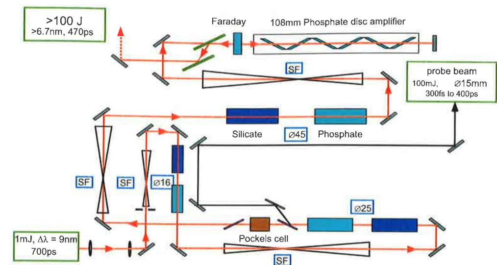
Figure 4.2: The pulses from the front end are amplified in two 16, 25 and 45 mm diameter glass amplifiers, respectively. The rods consist of different glass sorts to widen the gain curve. The final amplification is done in a 108 mm disc amplifier. Between the single amplifier stages are spatial filters (SF) to clean the beam profile.
