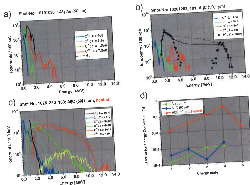
Figure 7.3: (a) Carbon spectra for an unheated 50 μm Au-target: the ion yield is very weak, the high energy cutoff for the highest charge state is around 0.5 MeV/nucleon. (b) Carbon spectra for an unheated Al/C-target (50 μm): the proton signal shows a gap due to detector properties which is optimized for heavier particles. The lines show two fits to bridge the detector gap H + -spectra, but the real spectra has still a high energetic tail which cannot be accounted for from the Thomson parabola -signal. (c) Carbon spectra for a heated Al/C-target (50 μm): The ion signals are strongly enhanced and the high energy cutoff is at higher energies. (d) Conversion efficiencies of laser energy to ions for all three targets: The unheated targets show a similar behavior. The heating increased the energy in the heavy ion signal by two orders of magnitude.
