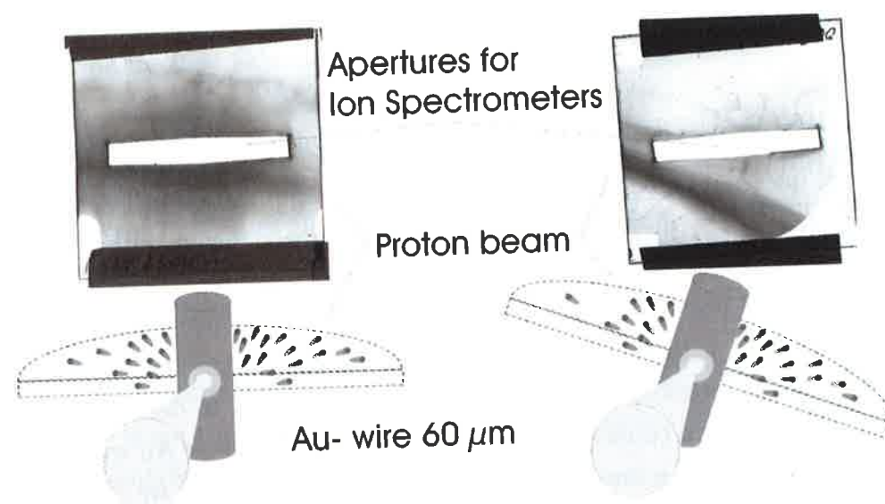
Figure 6.9: Experimental setup and RCF images of experiments with 60 \mu\text{m} gold wires. The convex rear surface constitutes a de-collimating cylinder-lens. Accordingly the proton beam was formed into a line.
