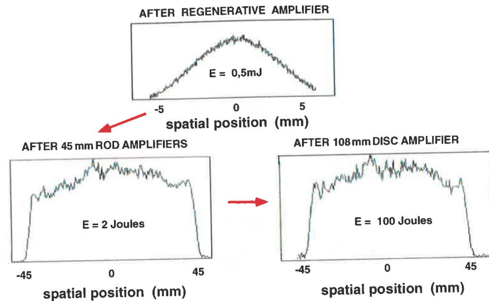
Figure 4.4: The beam profiles evolve gradually in a flat-top profile while passing the different amplifier stages. This reduces the peak intensities on the compressor gratings.
