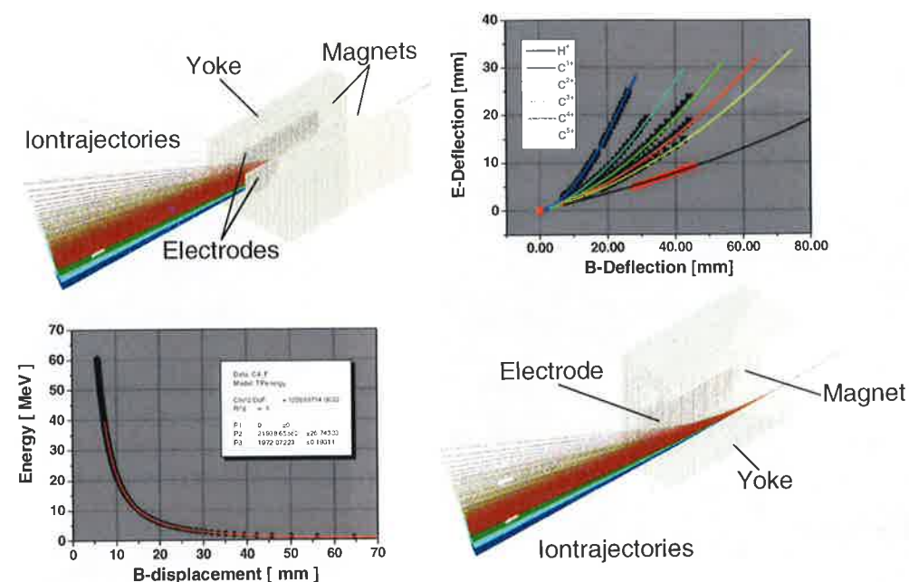
Figure 5.2: Thomson parabola calibration: top left and bottom right: a 3D computer model was needed to treat the fringe fields correctly. Top right: the simulated traces are overlayed with the measured data to identify the charge states. Bottom left: from the simulation an energy dispersion relation for the Thomson parabola can be obtained.
