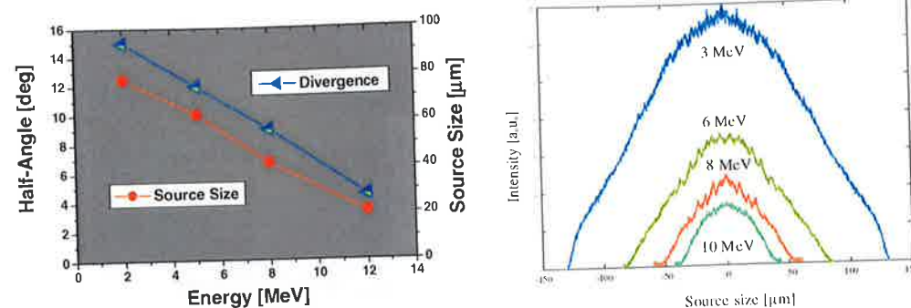
Figure 6.6: Real source size of laser accelerated protons in dependence of their energy. The spot size at the rear surface decreases from 260 \mu\text{m} diameter for 3 MeV protons to 80 \mu\text{m} diameter for 10 MeV.
