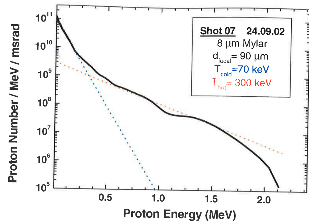
Figure 9.2: Proton spectra for a 8 \mu\text{m} Mylar target irradiated by a 0.6 \text{ J} pulse from the table-top, high rep-rate ( 10 \text{ Hz} ) MPQ ATLAS-10 laser.
