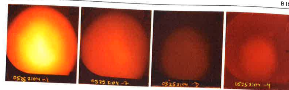
Figure 3. RCF images of the laser accelerated proton beam 5 cm behind the target. The ion energy increases from left to right. The divergence of the homogeneous beam decreases with increasing ion energy.
