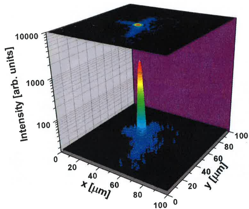
Figure 4.8: Typical focal spot for a LULI laser shot with an energy of \sim 15 J. The plot shows the intensity over the spatial extension of the focus.
