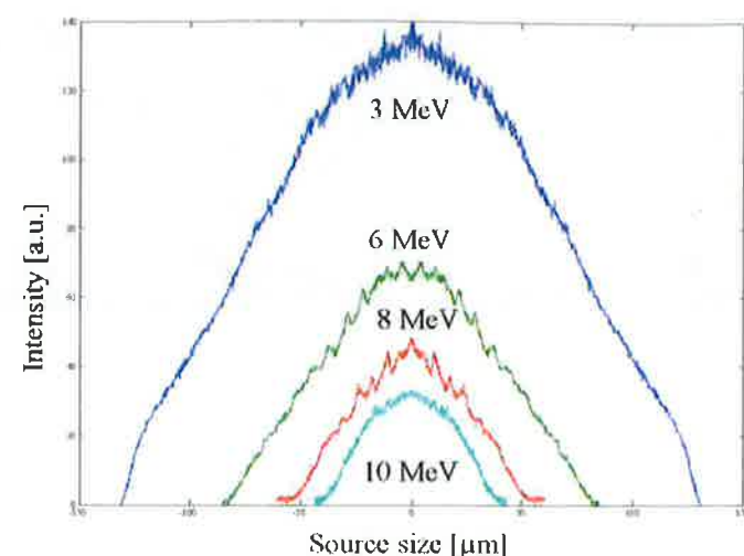
Figure 4. Real source size of the laser accelerated protons for different proton energies. The size at the rear surface decreases from 260 \mu\text{m} for 3 MeV protons to 80 \mu\text{m} for 10 MeV protons.
