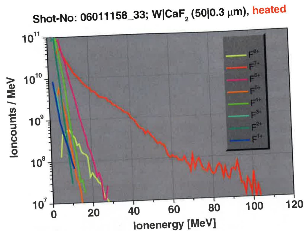
Figure 7.6: Resistively heated W/CaF 2 -target: All protons were removed and F 7+ -spectra is now dominantly accelerated: More than 100 MeV (5 MeV/nucleon) energy and more than 4% conversion efficiency are achieved for F 7+ /ions.
