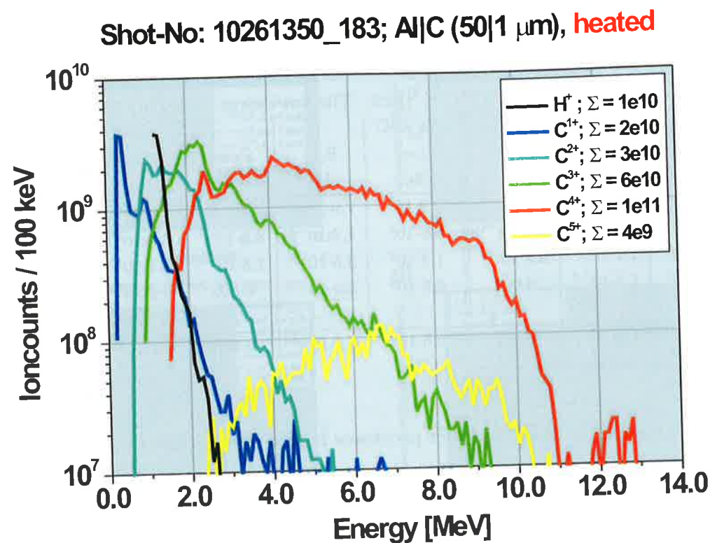
Figure 7.4: Carbon spectra for a heated Al/C-target ( 50 \mu\text{m} ): The ion signals are strongly enhanced and the high energy cutoff occurs at higher energies. The cutoff energies and ion numbers increase with increasing charge state.
