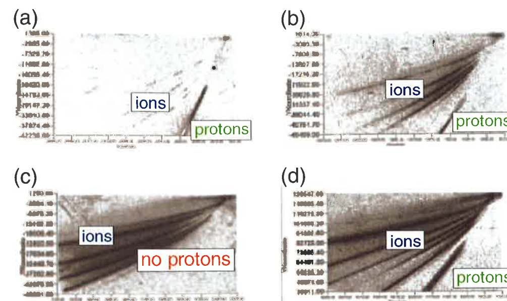
Figure 7.1: (a) Ion traces from an unheated Al/C-target on CR39. A strong proton line which is even too dense for counting at its onset is clearly visible while the ion signal is extraordinarily faint. (b) An Al/C-target resistively heated to \sim 800\ \text{K} shows a strong increase in the ion signal and energy while the proton signal is reduced. (c) By heating W-targets to \sim 1300\ \text{K} all protons can be removed. The ion signal and energy is strongly enhanced by orders of magnitude. (d) Al/ D_2 -target cleaned by laser ablation with a mJ-ns Nd:YAG pulse some 100\ \mu\text{s} before the main pulse. The result is similar to the resistive heating for Al-targets: The ion signal is enhanced but a substantial proton fraction remains.
