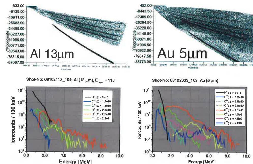
Figure 7.2: Typical Thomsonparabola raw data and spectra for unheated targets. Left: 13 \mu\text{m} Al-target, 11.2 J laser energy, right: 5 \mu\text{m} Au-target, 12 J laser energy. Both cases show strong carbon spectra, however in the case of the thin gold other traces, probably Oxygen, are also present, albeit very weak.
