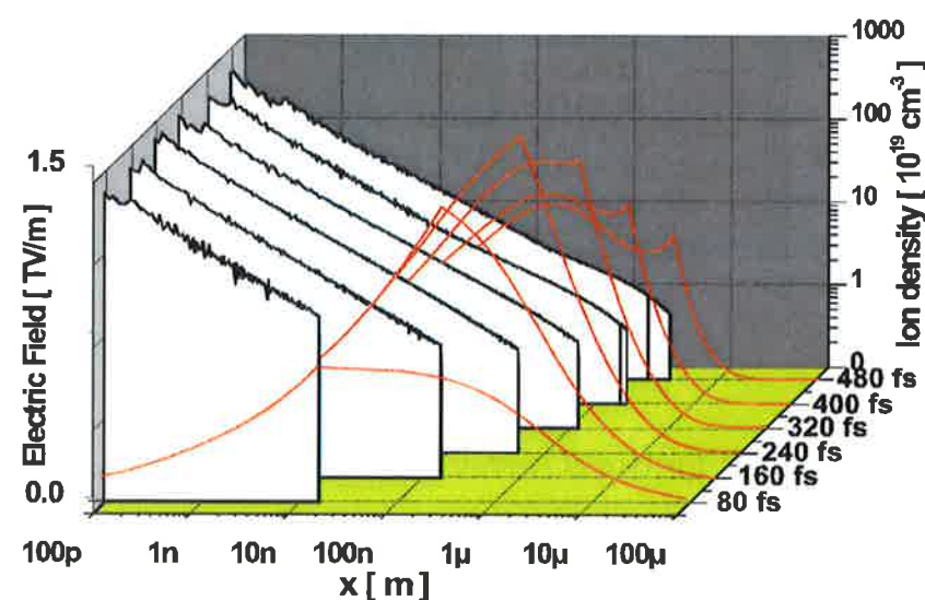
Figure 2: Spatio-temporal evolution of accelerating fields and ion densities.
