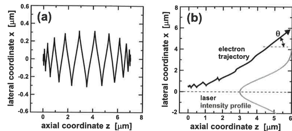
Figure 2.1: Electron trajectories in a strong laser field: (a) laser pulse of duration \Delta\tau = 20 fs, amplitude a_0 = 2.5 ( I = 1.3 \times 10^{19} \text{ W/cm}^2 at \lambda = 800 \text{ nm} ), and large lateral beam size; (b) same laser pulse, but in a tight focus (diameter d_{\text{FWHM}} = 3 \mu\text{m} , the laser lateral intensity profile is also shown). An electron, initially at rest at a distance of x_0 = 0.5 \mu\text{m} from the laser axis, is ejected under an angle of \theta \approx 52^\circ to the axis with an energy of E_{\text{kin}} = 0.64 \text{ MeV} .
