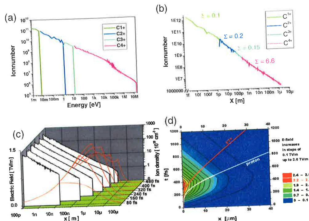
Figure 8.2: C^{4+} -spectrum calculated with 1D-kinetic model. Highest energy and absolute ion numbers are reproduced within an order of magnitude. (c) Time-space history of the accelerating electric fields (red curves) and the ion distribution (white curve): The region of maximum field moves out into the vacuum. Already during the pulse there exists an ion distribution on a \mu\text{m} -scale. (d) F^{7+} -trajectory and corresponding H^+ -trajectory in accelerating quasistatic field. The same field that accelerates F^{7+} to \sim 100 MeV accelerates protons to \sim 23 MeV. This result is in good agreement with the measured data.
