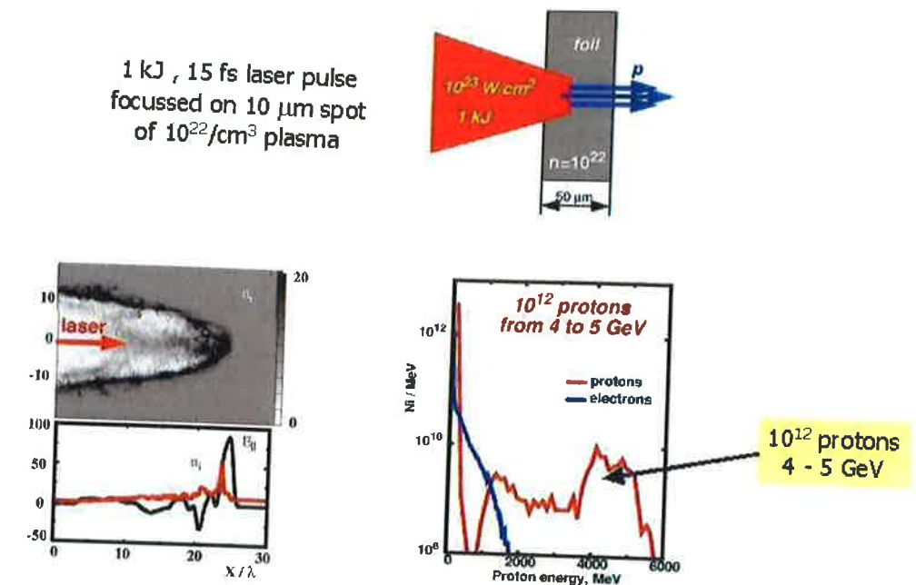
Figure 9.3: Laser-accelerated GeV protons: top: simulation setup and parameters; left: ion density ( n_i ) and longitudinal electric field; right: energy spectra of electrons and protons [101].
