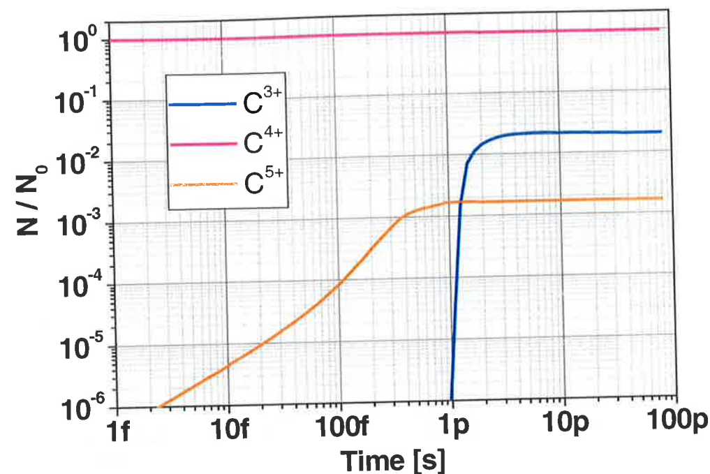
Figure 3.3: Charge transfer due to electrons in a laser accelerated C^{4+} -ion cloud from the time it leaves the target till it reaches the Thomson parabola-spectrometer. The transfer rates are calculated by the FLY-code. Electron and ion densities and temperatures are fully time-dependent.
