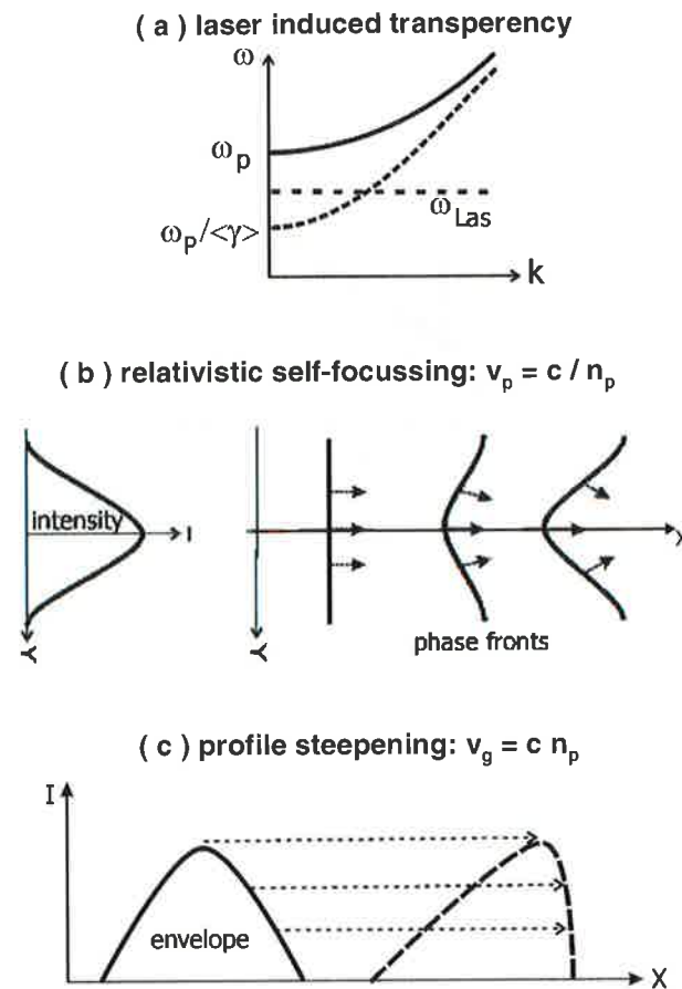
Figure 2.3: Effects of relativistic non-linear optics: (a) Laser Induced Transparency: High intensities producing \gamma \gg 1 reduce the plasma frequency \omega_p . The plasma becomes transparent at its former plasma frequency. (b) Relativistic Self-focussing: A pulse with a transverse intensity profile increases the refractive index of the plasma strongly along its propagation axis, but not as much in the fringe region. The plasma acts as a positive lens. (c) profile steepening: The central pulse regions with higher intensities move with larger group velocity v = n_p c than the head of the pulse, the profile steepens.
