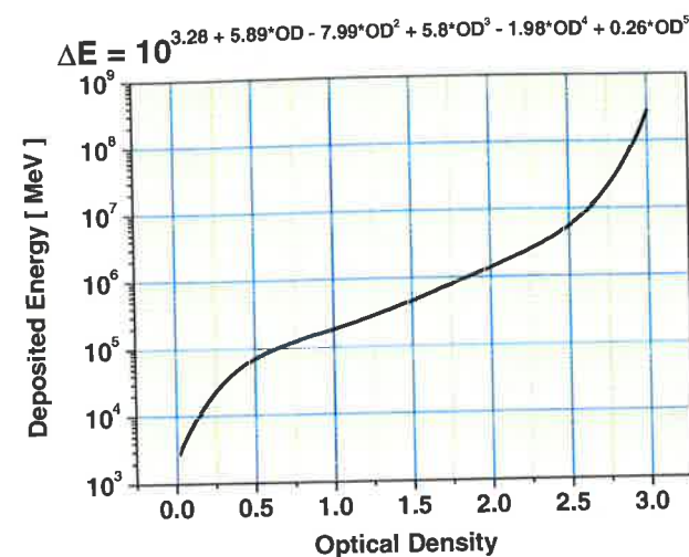
Figure 4.11: Calibration curve for proton energy deposition in RCF (courtesy of A. Blaze-vic).
