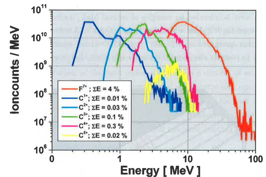
Figure 1: Spectra of laser-accelerated heavy ion-jets.
