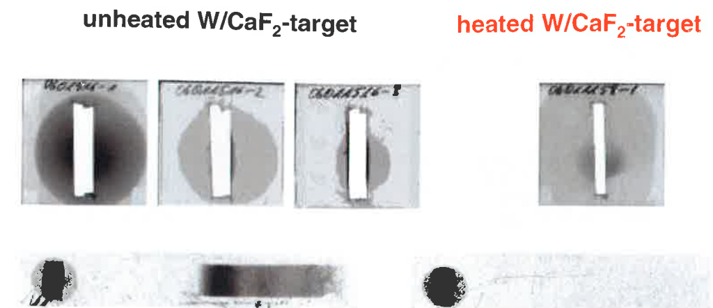
Figure 7.7: RCF and proton spectrometer raw data for shots on cold and heated W/CaF 2 -targets. For non-heated targets the typical proton spectra was measured and the RCF detectors showed the usual beam profile. For the heated targets the proton signal completely vanishes, disproving the existence of high energy protons. The first layer of RCF shows a narrow spot, similar to the deeper layers, i.e. the high energy tail, of measured proton spectra. In the absence of protons this spot has to be caused by heavier ions and corresponds to fluorine ions >4 MeV/nucleon.
