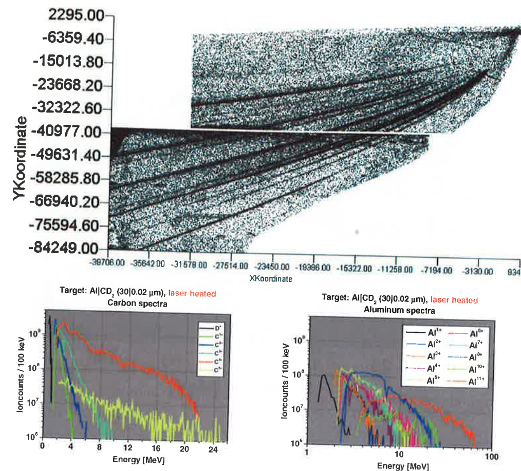
Figure 7.5: Carbon and aluminum spectra for a laser-heated Al/CD 2 -target: The ion signals are strongly enhanced and the high energy cutoff occurs at even higher energies as before. Spectra for all carbon charge states up to \text{C}^{5+} could be identified and nearly all charge states of Al up to 11+. The \text{Al}^{9+} charge state cannot be identified since it coincides with the \text{C}^{4+} charge state. Between \text{Al}^{13} and \text{Al}^{14} is a track that could not be identified.
