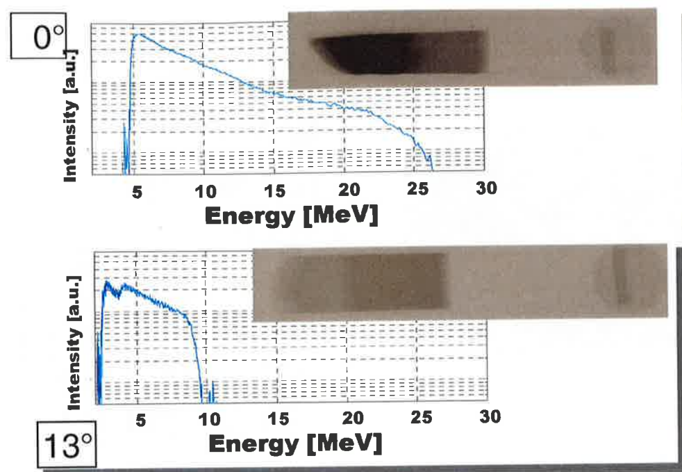
Figure 6.4: Proton spectra at 0^\circ and 13^\circ for a typical Au-target. The high-energy cutoff is strongly reduced at larger angles.
