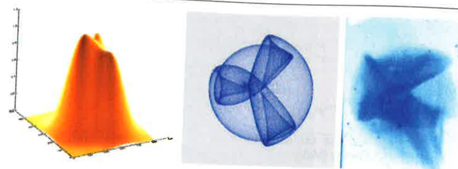
Figure 5. Proton beam filamentation due to electron transport. Simulation of a filamented electron sheath (left) in plastic causes the proton beam to show structure (central part). The experiment (right) shows an excellent agreement with the simulation.
