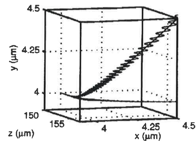
Figure 2.2: 3-dimensional trajectory of an electron accelerated and ejected by a high intensity laser pulse ( a_0 = 0.3 , \tau_{Pulse} = 200 fs). The calculations take into account the field components in laser direction arising from the focussing [16].
