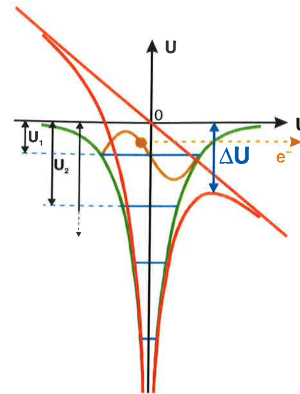
Figure 3.1: Field Ionization by Barrier Suppression: An external electric field disturbs and suppresses the Coulomb barrier of an atom. An electron at the potential U_1 is bound in the unperturbed potential (green). The external field depresses the barrier by the amount \Delta U so that the electron suddenly finds itself at an energy higher than the new disturbed potential (red).
