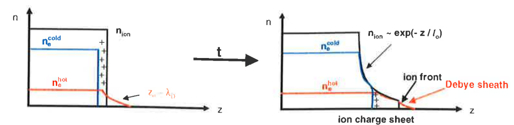
Figure 2.5: Schematics of the TNSA-mechanism
