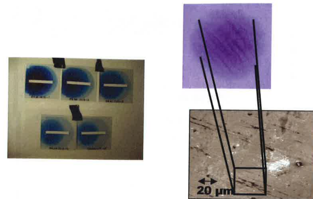
Figure 6.3: For an electroplated Au-target with smooth surface the signal is homogenous through all layers of RCF. For a target made from rolled gold structures appear in the proton signal which correspond to surface structures visible under an electron microscope.
