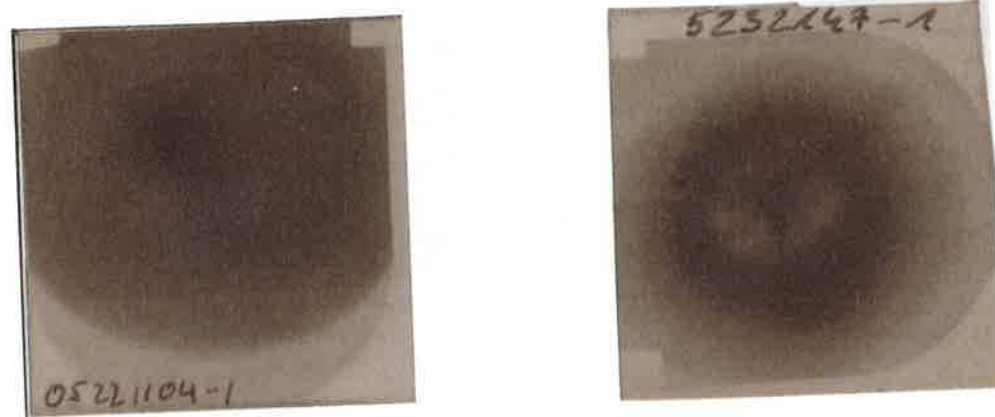
Figure 6.8: Beam imprint for an undamaged (left) and a damaged (right) target front side. A small crater on the front side caused a ring structure in the proton signal.
