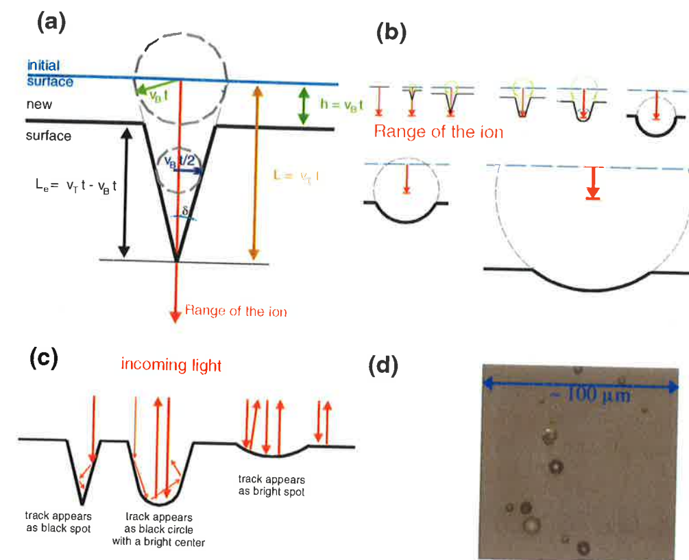
Figure 5.4: Iontracks in CR-39: (a) schematic diagram of track formation. h : thickness of removed surface, L : length of the etched track at time t , v_B : bulk etch velocity, v_T : track etch velocity. (b) development of the track during the etch process. First a cone is etched up until the end of the ion range is reached. Further etching produces a sphere at the end of the cone that gets bigger and finally develops into a bowl shape. (c) different track shapes show different appearances depending on how they reflect the light. (d) microscope image showing exemplary tracks.
