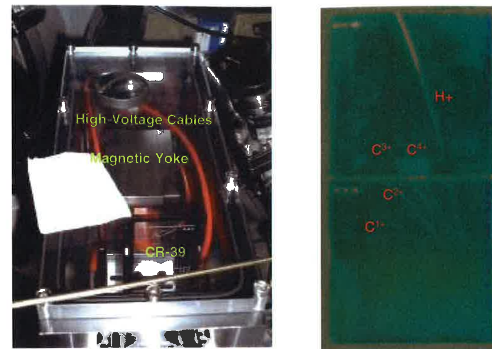
Figure 5.1: eft: Thomsonparabola spectrometer and right: etched CR-39 detector, showing \text{H}^+ and \text{C}^{1+} - \text{C}^{4+} parabolic ion traces.
