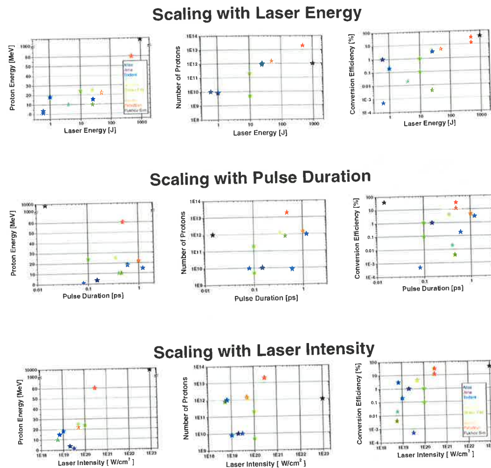
Figure 9.4: Scaling behavior of proton energy, yield and energy conversion efficiency with laser parameters. The top row shows scaling with laser energy, the middle row scaling with pulse duration and the bottom row scaling with laser intensity on target. The experiments together with the references are listed in Tab. 9.1. The colored stars are experimental data, the black star is from a 3D-simulation with VLPL.
