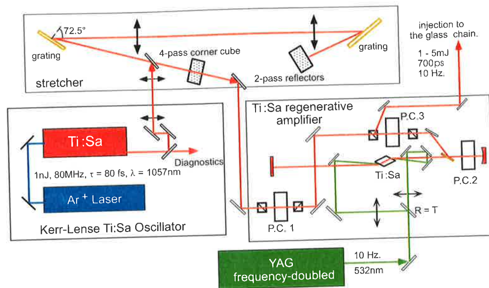
Figure 4.1: The frontend of the LULI 100 TW laser produces 80fs laser pulses. First the pulses are created in a Ti:Sapphire oscillator pumped by an \text{Ar}^+ -laser. These pulses are then stretched to 700 ps by a grating stretcher and amplified in a Nd:YAG pumped Ti:Sapphire regenerative amplifier to a level of \sim 5 mJ.
