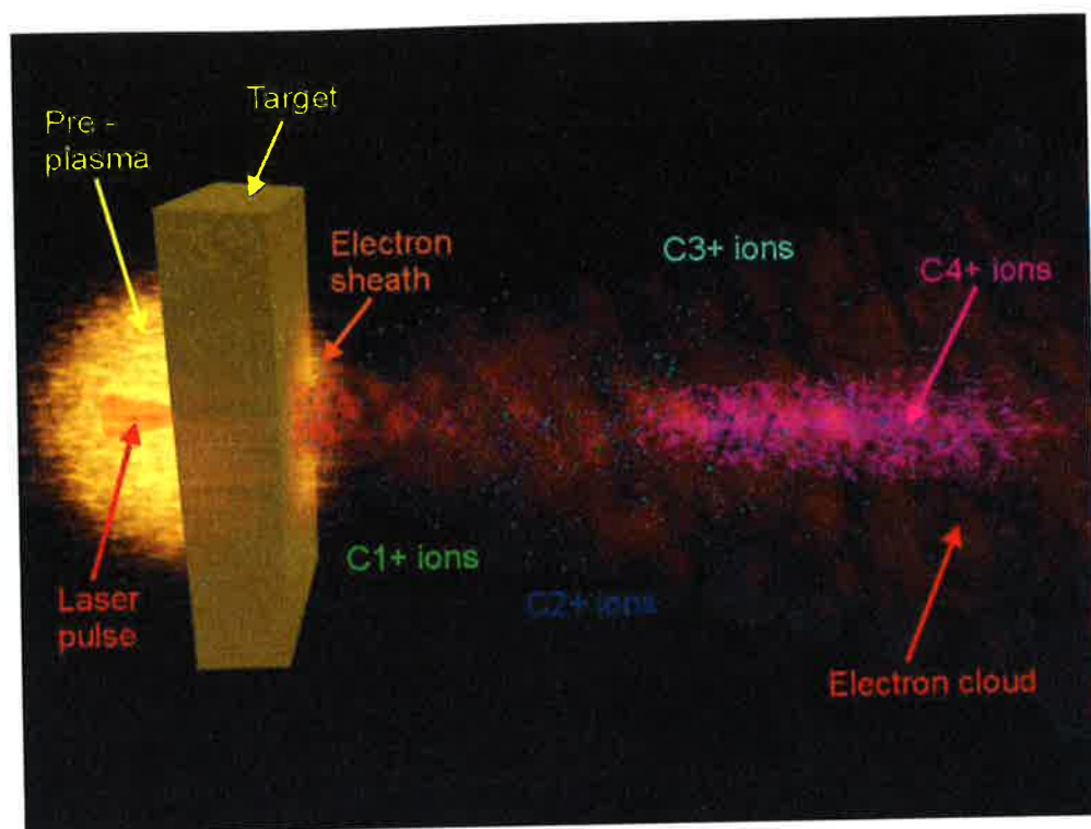
Figure 2.4: Ion acceleration from thin foil targets.
