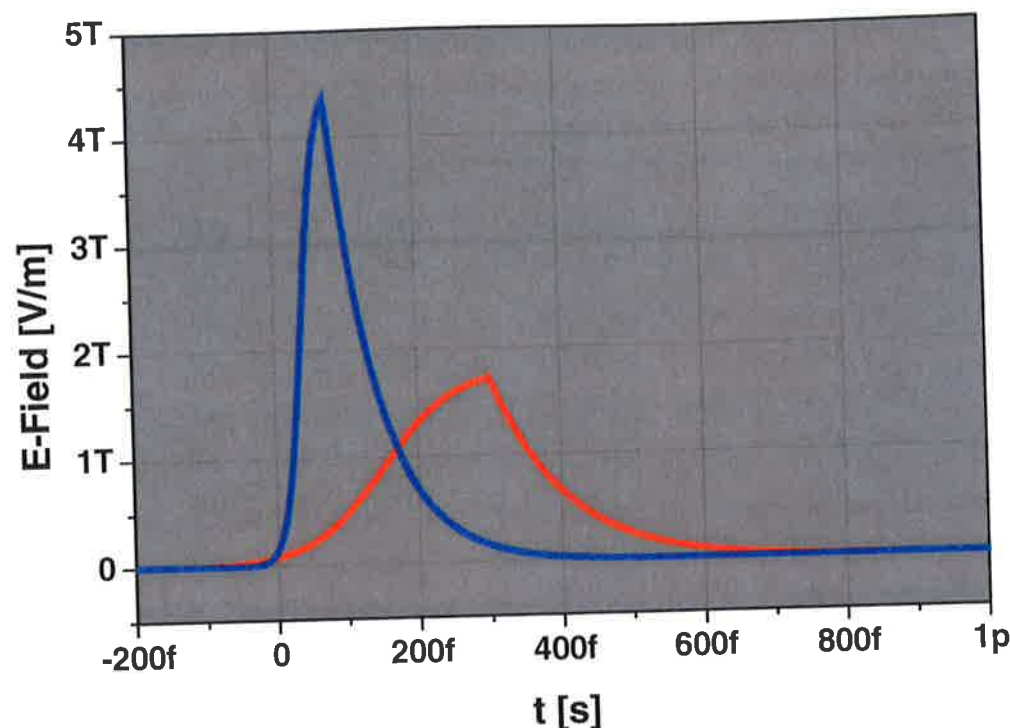
Figure 8.1: Accelerating fields for C^{4+} -ions. In order to achieve the right cutoff energy the field duration and strength are varied. The maximum field is much shorter than the laser pulse. A field of the duration of the laser pulse is in good agreement with TNSA-model predictions with respect to the field strength.
