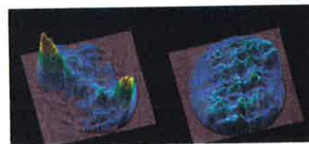
Fig. 2. Fluence patterns in the plane of the first compressor grating. Left, DM1 is replaced with a plane mirror; peak fluence, 300 mJ/cm 2 . The double-peak pattern is due to the coarse two-half structure of the WFAs shown in Fig. 3. Right, DM1 is optimized; peak fluence reduced to 90 mJ/cm 2 . The remaining fluence modulation arises from the fine structure of the WFAs (Fig. 3). The very high spatial frequencies, which carry little energy, are lost on propagation through the spatial filter SF2 (Fig. 1).
