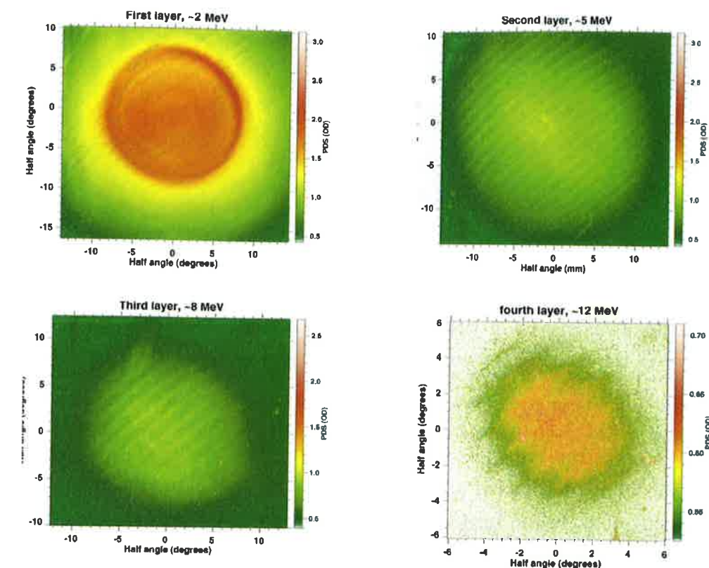
Figure 6.5: Proton signal in RCF from an 18\ \mu\text{m} Al-target with a 0.2\ \mu\text{m} deep and 3\ \mu\text{m} wide grid structure. The laser shot was fired at LANL's Trident Short Pulse Laser and contained 26 J in a \sim 20\ \mu\text{m} diameter focus. The pulse length was about 1.2 ps, making for an Intensity of \sim 7 \times 10^{18}\ \text{W}/\text{cm}^2 on target.
