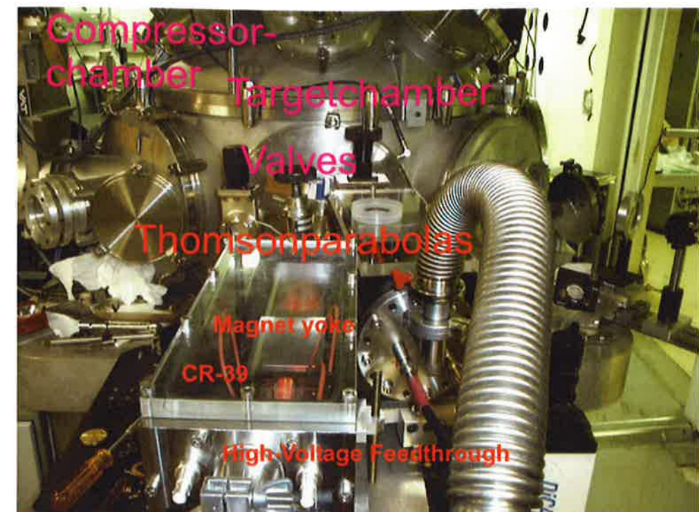
Figure 4.7: The LULI targetchamber has 1.2 m diameter. In the foreground the two Thomson parabolas can be seen which are attached to the chamber via valves to have independent access without breaking the vacuum. In the upper left corner a part of the compressor chamber can be seen.
