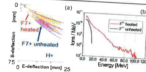
FIG. 2 (color). (a) Overlaid signals of heated (orange) and unheated (blue) W/CaF 2 targets. The proton signal vanishes for heated targets; the fluorine signals (especially \text{F}^{7+} ) go up to much higher energies. (b) Corresponding \text{F}^{7+} spectra: \text{F}^{7+} ions achieve more than 100 MeV (5 MeV/nucleon).
