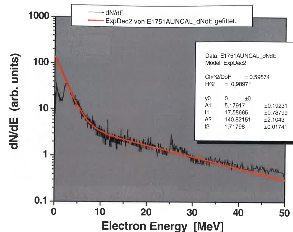
Figure 6.1: Electron spectra for a typical Au-target shot with 24J.
