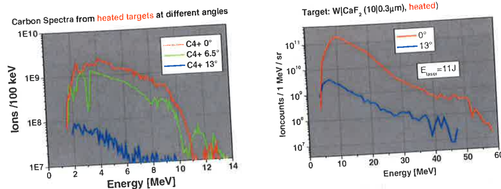
Figure 7.8: (a) C^{4+} spectra at 0, 6.5, and 13° from heated targets. The spectra at 0° and 6.5° were measured on the same shot. Due to the substrate a major proton fraction was still present but the ion acceleration was enhanced. (b) F^{7+} spectra at 0° and 13° from the same shot. The targets were resistively heated and most of the protons could be cleaned of. In both cases the 13° spectra are strongly decreased.
