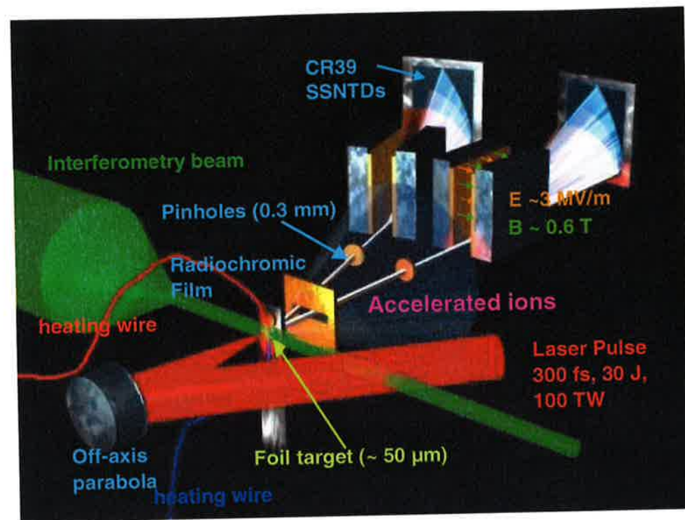
Figure 4.10: Experimental Setup: the target is mounted free standing and can be resistively heated via the two wires, the main laser pulse (red) is focussed optics by an off-axis parabola. The interferometry beam (green) is expanded after the target to obtain a magnified image. Behind the target is the RCF-stack diagnostics and two Thomson parabola-spectrometers with CR-39 detector plates.
