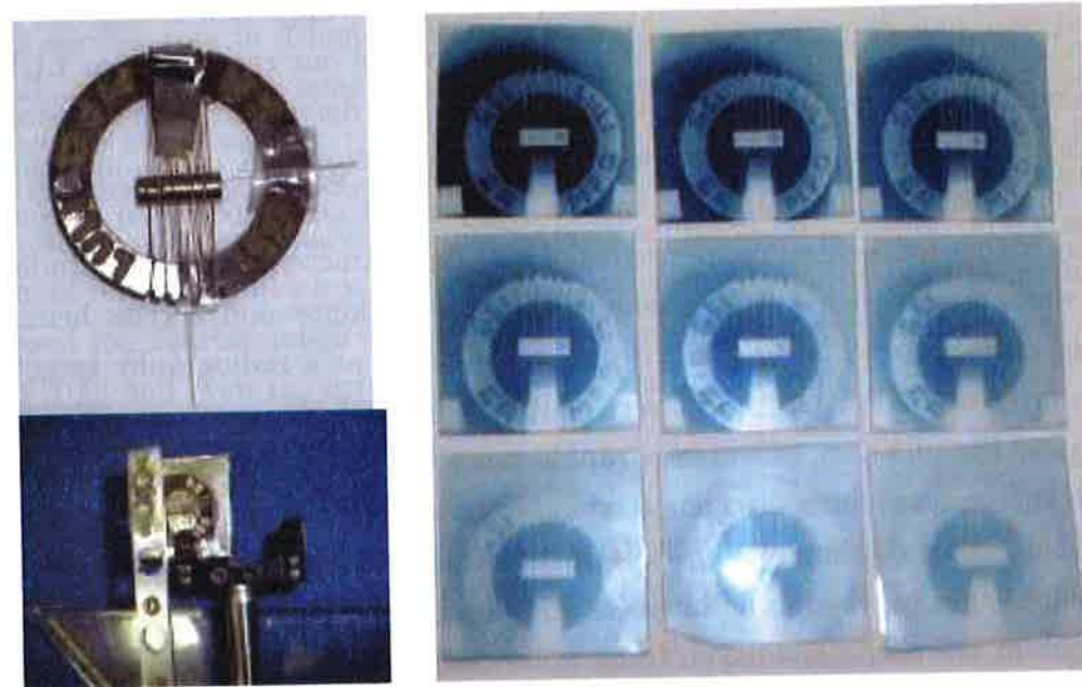
Figure 9.5: Proton radiography of a compound target. Top left: Compound target consisting of an epoxy ring, several wires of varying thicknesses, a steel hohlraum and a glass shell. Bottom left: target mounted \sim 5 cm behind the proton producing target foil. Right: Radiographic images at different proton energies.
