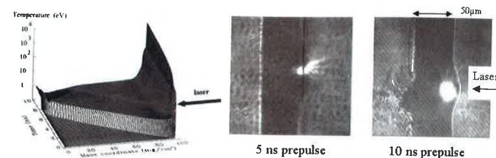
Figure 6.7: left: simulation of the shock wave launched by the prepulse. The shock wave reaches the rear surface at about 7 ns. middle: Interferometric image of the plasma conditions on the front and rear target surface at normal prepulse level at 5 ns before the main pulse. No shock breakout occurred yet, the rear surface is unperturbed. right: The prepulse at 10 ns before the main pulse causes perturbation of the rear surface due to shock wave breakout. No protons were detected.
