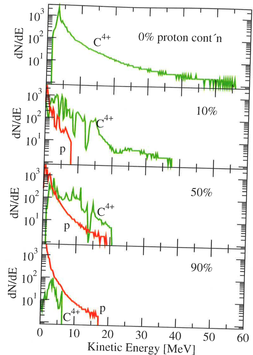
Figure 8.4: Influence of contaminating protons on the carbon spectrum: In the presence of protons the carbon spectrum has lower energies and a cutoff forms.
