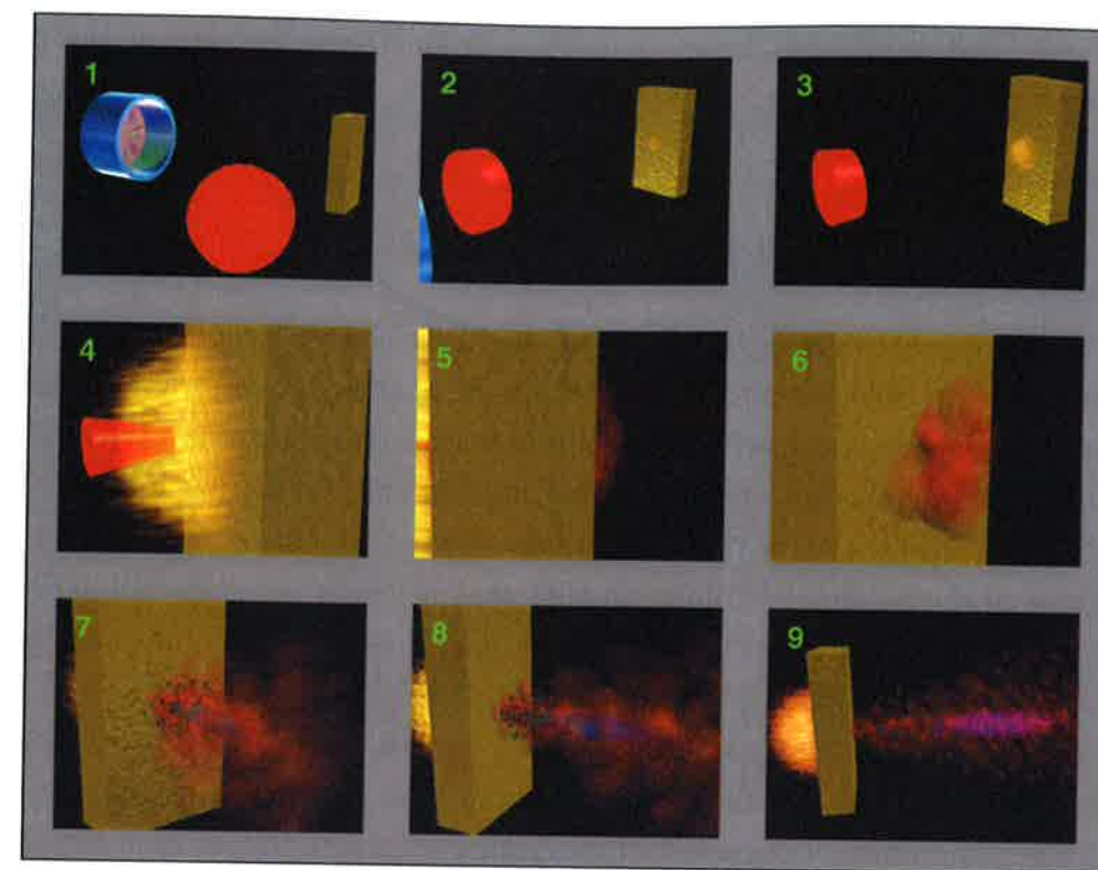
Figure 9.1: Schematics of laser induced ion acceleration: (1,2) A laser pulse is focused by an off-axis parabola on a pure carbon target. (2,3) Prepulses and ASE create a plasma density gradient at the target front side. (4) The main pulse interacts with this preplasma, (5) accelerating relativistic electrons through the target. (6) These electrons set up an ultra-strong (TV/m), quasistatic space charge field at the rear surface. (7) This electric field ionizes the rear surface atoms ( C^{1+} : green). (8) The ionized atoms start moving and are further ionized ( C^{2+} : blue, C^{3+} : cyan, C^{4+} : green; scales: fs, nm). (9) The ions are accelerated to MeV energies, the higher the charge state, the higher the energy and the smaller the divergence.
