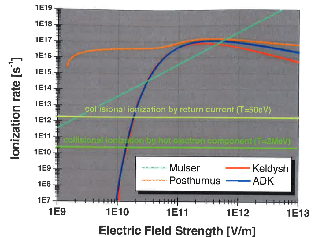
Figure 3.4: Ionization rates for C^{1+} in a strong external electric field according to the numerical model of Mulser (cyan) and the analytical models by Keldysh (red), Posthumus (orange), and ADK (blue). The horizontal lines show the ionization rates due to collisional ionization by the hot (2 MeV) electron component (green) and the cold (50 eV) return current (yellow).
