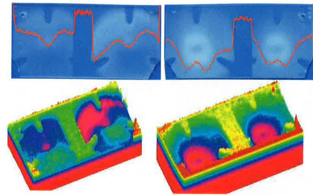
Figure 5.5: A CR-39 plate irradiated at two spots with an alpha source. After etching the plate was scanned at different angles. The change of the angle caused a drastic change in the signal. Top: scanned images, the left shows a bright center of the irradiated spots, the right shows ring structures. The red lines are horizontal line-outs from the middle of the plates. Bottom: False color image of the scanned pictures, the colors represent different brightness values.
