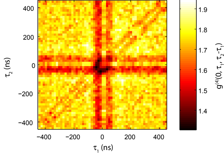
Figure 6.12: Experimental fourth-order intensity correlation function g^{(4)}(0, \tau_1, \tau_2 - \tau_1) . A discussion of the rich temporal structure will be the subject of future investigations.
