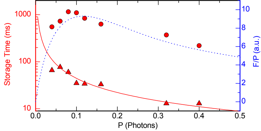
Figure 5.5: Storage time with ( \bullet , left axis) and without ( \blacktriangle , left axis) feedback versus probe power in units of photons in the empty cavity. The error bars are smaller than the symbols. Without feedback, the storage time is mostly limited by radial momentum diffusion as confirmed by the T_{rad} = \frac{a}{P} fit (red line, left axis). With feedback, an increase of the storage time by more than one order of magnitude is observed for a broad range of probe powers. The maximum occurs as a compromise between a low radial heating rate and a good information rate. This is reflected by ratio of fidelity and heating rate, F/P (dashed blue line, right axis), which qualitatively reproduces the power dependence of the storage time.
