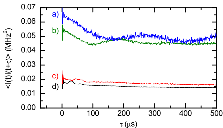
Figure 5.9: Time-dependent intensity-correlation function without feedback in the shallow (a) and deep (b) trap, and with feedback using an integration time of the feedback algorithm of 32 \mu\text{s} (c) and 16 \mu\text{s} (d). Without feedback the radial oscillations cause a characteristic bump at one-half of the oscillation period. This bump disappears when the feedback is enabled.
