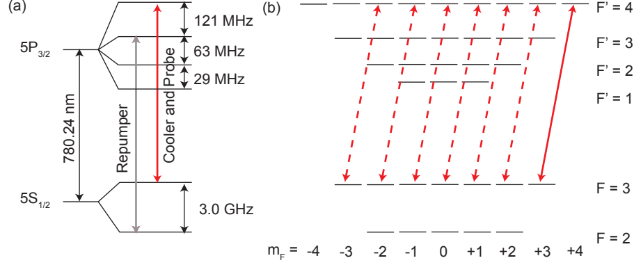
Figure 3.2: (a) Relevant hyperfine transitions of the D2 line of ^{85}\text{Rb} . For the operation of the magneto-optical trap, two lasers, a cooler and a repumper, are needed. (b) In the cavity, the probe laser drives the closed F=3, m_F=+3 to F'=4, m_F=+4 transition justifying the two-level approximation for the atom.
