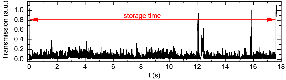
Figure 5.3: Sample transmission trace of a trapped atom. The atom is detected at t=0 by the drop in the transmission. The dipole trap is switched on, and the feedback is activated. The escape time of the atom is determined from the jump in the transmission back to the empty-cavity value.
