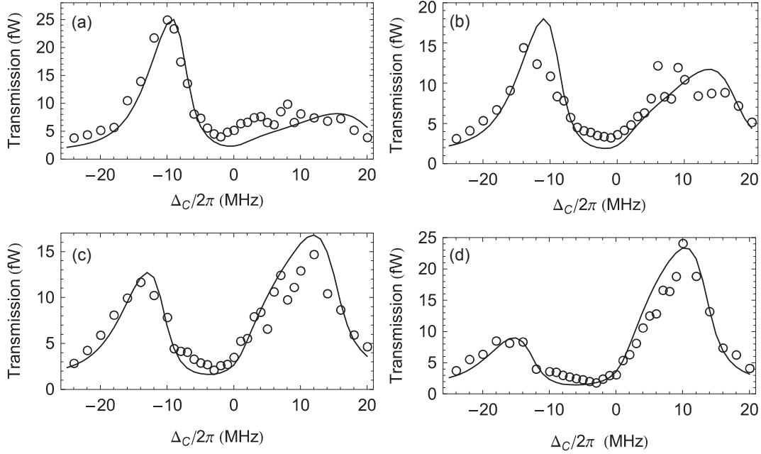
Figure B.1: Experimental (o) and theoretical (solid line) normal-mode spectra for different dipole trap depths. The four spectra corresponding to a transmitted trap power of 340 nW, 310 nW, 280 nW, 250 nW from (a) to (d)). The width of the atomic distribution ( \sigma = 0.35 ), the displacement ( Z_0 = 0.43 ), the AC-Stark shift ( 2U_0/2\pi = 46 MHz), the empty-cavity transmission (260 fW) and the dark count rate (1 fW) for the theoretical curves were adjusted manually for plot (a) and then kept constant. Only the Stark-shift was scaled according to corresponding trap power. We find good agreement without any additional fit parameter.
