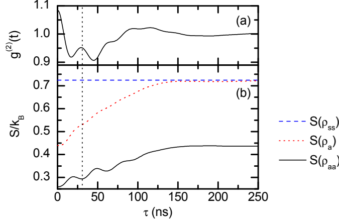
Figure 6.11: (a) Theoretical second-order correlation function for a fixed atom ( g/2\pi = 12 MHz, \Delta_c/2\pi = -12 MHz, \eta = 3.5\kappa ). (b) Entropy of the steady-state density matrix ( S(\rho_s) , dashed blue line), time dependence of the entropy after the detection of a photon ( S(\rho_a(\tau)) , dotted red line) and entropy after two photon detections separated by the time \tau ( S(\rho_{aa}(\tau)) , solid black line). The smaller the entropy, the larger our knowledge about the state of the system. The detection of two photons separated by one period of the vacuum Rabi oscillations (vertical dotted line) provides us with additional knowledge about the state of the system causing a local minimum of S(\rho_{aa}(\tau)) at this time. This explains the interplay of vacuum Rabi oscillations and super Rabi oscillations discussed in the last section.
