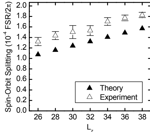
Figure 4.3: The spin-orbit splitting ( \Delta ) is a consequence of a coupling between the intrinsic (polarization, \sigma ) and the orbital angular momentum L_z of the light beam. As predicted by theory (▲), it scales linearly with L_z . However, a systematic discrepancy of about 20 % between theory and experiment is found.
