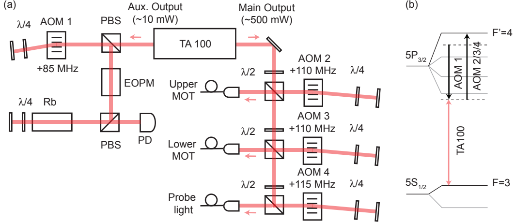
Figure 3.3: (a) Optical setup of the cooling and probe laser. The auxillary output (left part of the figure) of the tapered amplifier laser system (TA100) is used to stabilize the frequency of the laser to a crossover line of a Doppler-free rubidium spectroscopy (cf. text for details). The main output of the tapered amplifier (right-hand side) is divided into three parts. Two parts provide the light for the upper and lower beams of the MOT, whose frequencies can be tuned independently to allow for an atomic fountain. The last part is the probe light that drives the atom-cavity system. All three beams are coupled into optical fibers to deliver the light to the respective parts of the experiment. (b) The laser is locked to a Rb crossover resonance. Because of the detuning of the crossover resonance of 60 MHz and an additional shift of 170 MHz due to the passage through AOM 1 in a double-pass configuration, the output of the laser is red-detuned by 230 MHz with respect to the F=3 to F'=4 transition of the D2 line of ^{85}\text{Rb} . Three AOMs in double-pass configuration (AOM 2, 3, 4) shift the MOT and probe light back on, or close to, resonance.
