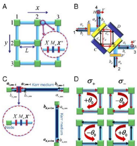
Scheme of the optical network (from the original publication) (Graphic: Theory Division)
