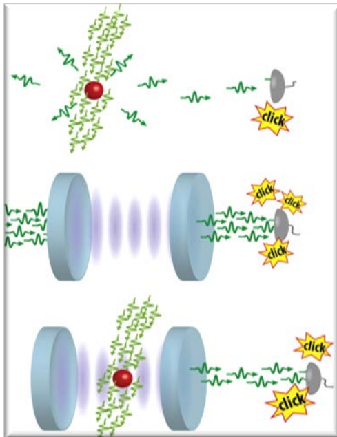
Figure: Illustration of the two-photon blockade.
