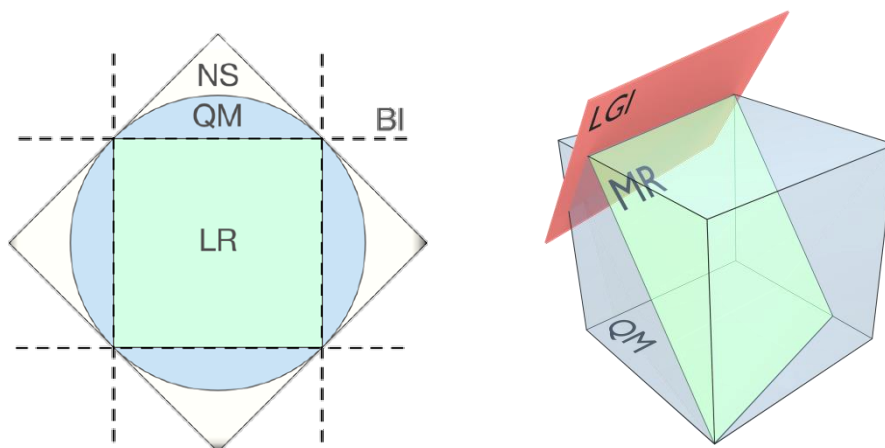
Figure caption: Left: All reasonable physical theories, including quantum mechanics (QM), obey the no-signaling (NS) assumption. Local realism (LR) is tightly delimited by Bell inequalities (BI) which are therefore an optimal tool for experimental tests. NS, QM, and LR all live in a probability space with the same dimension; for simplicity the drawing is in two dimensions. Right: The picture is very different for macroscopic realism (MR). MR and QM live in probability spaces of different dimensions. The Leggett-Garg inequalities (LGI) are cuts through the QM space and do not tightly delimit MR. Hence, LGI are not optimal for experimental tests of MR.
