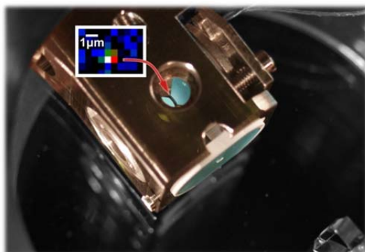
Fig. 1: Central part of the experimental setup: A single atom is trapped in the narrow gap between two highly reflecting mirrors (light blue) that form an optical resonator. Reflection of single photons from the resonator implements a quantum logic operation between the atom and the photons. Graphic: Andreas Reiserer, MPQ, Quantum Dynamics Division.
