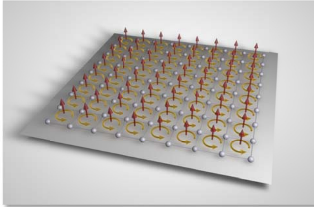
Fig. 1 Cyclotron orbits of atoms exposed to extremely strong effective magnetic fields in specially engineered light crystals. The effective field strengths realized in the experiment correspond to tens of thousands of Tesla magnetic field strength applied to a real material. In the experiment the celebrated Hofstadter-Harper as well as the Quantum Spin Hall Hamiltonian could thereby be implemented.
