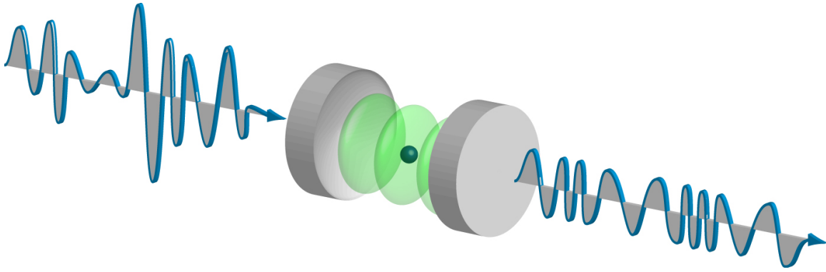
Fig. 1: A single rubidium atom in a cavity squeezes the quantum fluctuations of a weak laser beam, decreasing the fluctuations of the amplitude at the expense of the phase. The effect is exaggerated for clarity.
