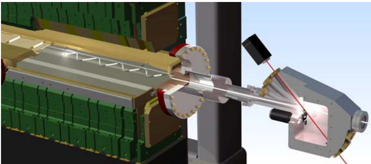
Figure caption: To time-stamp the arrival of each x-ray pulse, researchers use an electro-optic crystal (green) placed next to the electron beam (white) in the linear accelerator just before the beam produces x-rays. A laser (red) probes changes in the crystal to measure the exact time the beam passed by. The image was created by Jean Charles Castagna, SLAC.
