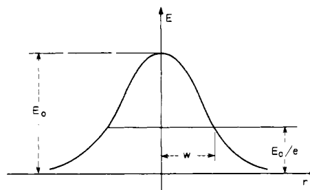
Fig. 5. Amplitude distribution of the fundamental beam.
