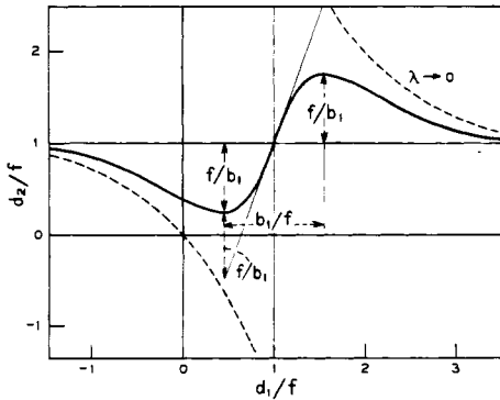
Fig. 13. The waist spacing d_2 as a function of the lens-waist spacing d_1 .
