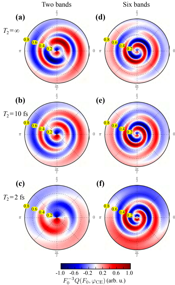
Figure 4.6: The residual current density Q(F_0, \varphi_{CE}) . Similarly to Figure 4.5, the distance to the origin corresponds to the pulse amplitude F_0 , which varies from zero to 0.8 \text{ V/\AA} , while the angle to the horizontal axis encodes the carrier-envelope phase \varphi_{CE} . The color coding of F_0^{-3}Q(F_0, \varphi_{CE}) is individually normalized for each diagram. Panels (a)–(c) show two-band results (1 VB, 1 CB), while panels (d)–(f) display six-band (3 VBs, 3 CBs) calculation results. Each horizontal pair of plots corresponds to a certain value of dephasing time T_2 as indicated by the labels.
