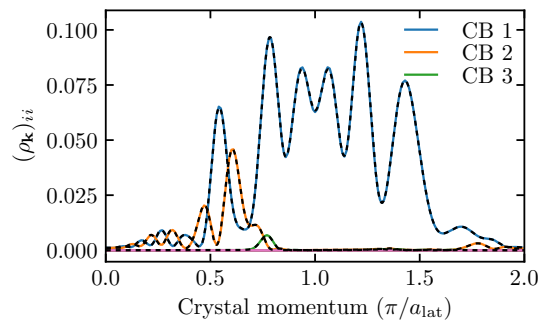
Figure 3.3: Distributions of electrons in the conduction bands (CB) after excitation by a pulse with E_{\max} = 1.5 \text{ V/\AA} according to a velocity gauge calculation (colored, solid lines) and length gauge calculation (black, dashed lines).
