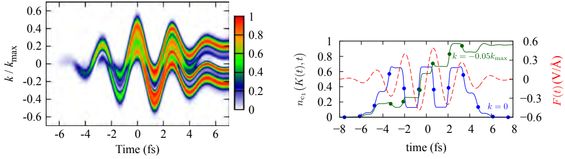
Figure 4.7: (a) Temporal evolution of the conduction-band population in a two-band simulation for F_0 = 0.5 \text{ V/\AA} , \varphi_{\text{CE}} = \pi/2 , T_2 = \infty . (b) Time dependence of the CB population in the two-band simulation (blue and green curves). It is calculated along reciprocal-space pathways K(t) that satisfy the acceleration theorem. The starting point is the \Gamma point ( k = 0 ) for the blue curve and k = -0.05k_{\text{max}} for the green curve. The bold dots on the curves denote moments of passage in the vicinity of the \Gamma point. The dashed red curve shows the electric field of the pulse ( F_0 = 0.5 \text{ V/\AA} , \varphi_{\text{CE}} = \pi/2 ).
