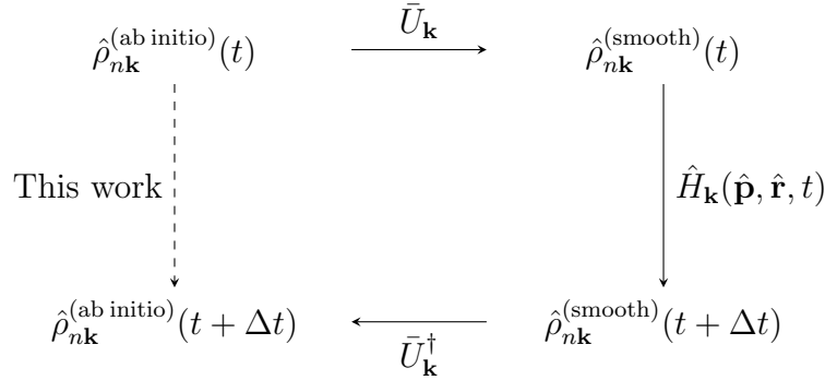
Figure 2.1: The density matrix \hat{\rho}_{n\mathbf{k}}^{(\text{ab initio})} is constructed from a set of wave functions |u_{n\mathbf{k}}^{(\text{ab initio})}\rangle that are not necessarily smooth functions of \mathbf{k} . A unitary, but unknown, matrix \bar{U}_{\mathbf{k}} may be applied at wave functions at every \mathbf{k} in order to transform the wave functions to a gauge where the derivative operator that appears in \hat{H}_{\mathbf{k}}(\hat{\mathbf{p}}, \hat{\mathbf{r}}, t) can be evaluated more easily. In this section, a numerical approach is proposed to evaluate the derivative operator in the ab initio gauge for a mixed system.
