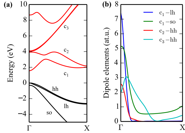
Figure 4.2: (a) The energies of the three highest valence bands (black) and the five lowest conduction bands (red) of GaAs along the line from the \Gamma -point to an X-point. All of the bands are doubly degenerate. (b) Magnitude of the dipole moments |\mathbf{d}_{ij}(\mathbf{k})| for the most important interband transitions.
