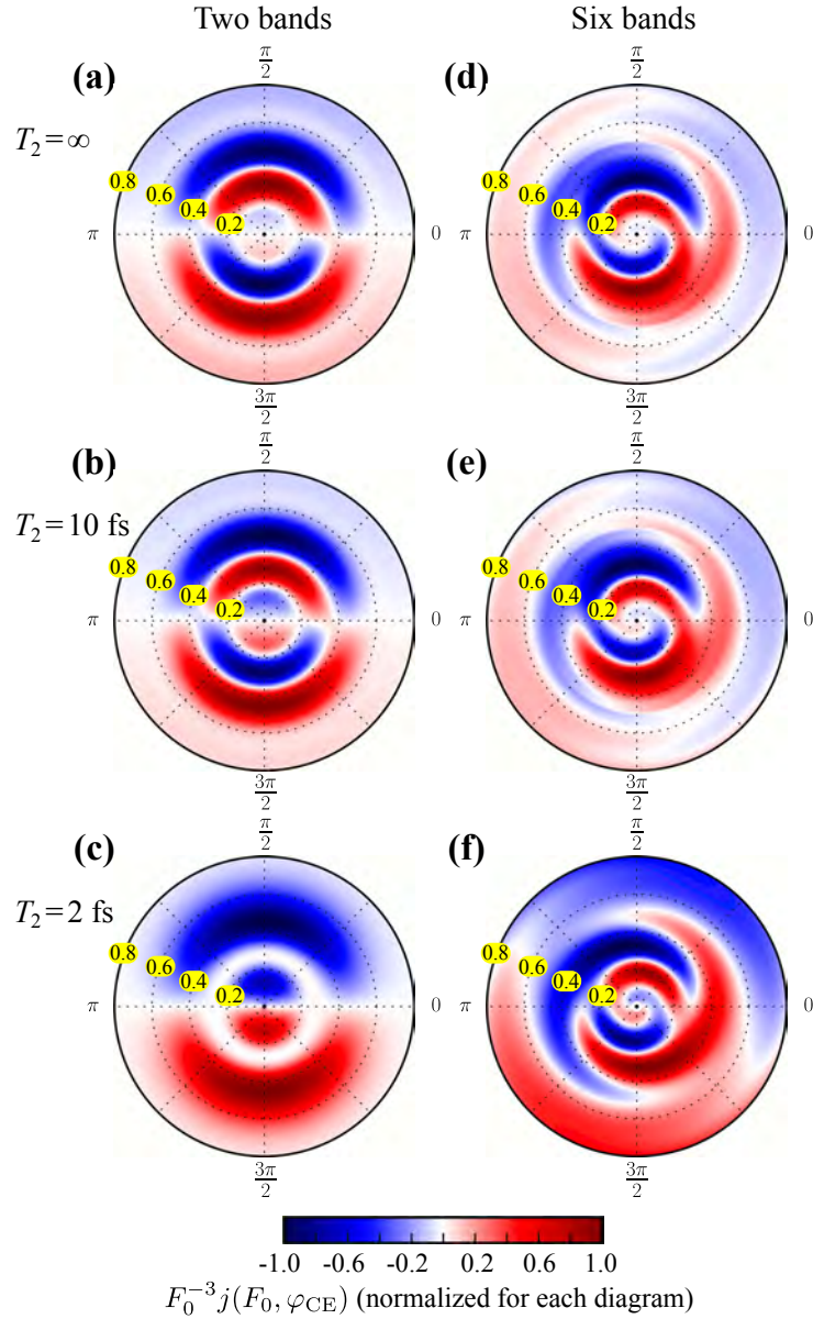
Figure 4.5: The residual current density j(F_0, \varphi_{CE}) . In these diagrams, the distance to the origin corresponds to the pulse amplitude F_0 , which varies from zero to 0.8 \text{ V/\AA} , while the angle to the horizontal axis encodes the carrier-envelope phase \varphi_{CE} . The color coding of F_0^{-3}j(F_0, \varphi_{CE}) is individually normalized for each diagram. Panels (a)–(c) show two-band results (1 VB, 1 CB), while panels (d)–(f) display six-band (3 VBs, 3 CBs) calculation results. Each horizontal pair of plots corresponds to a certain value of dephasing time T_2 as indicated by the labels.
