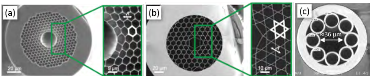
Fig. 3.11. (a) Cross-section of PBG-guiding PCF (taken from ref. 288). (b) Cross-section of Kagomé-type hollow-core photonic crystal fiber (HC-PCF) (taken from ref. 288). (c) Cross-section of anti-resonant guiding HC-PCF with a simplified cladding structure (taken from ref. 289). Images were taken through scanning electron microscopy. The marked pitch \Lambda is not of interest in this context.
