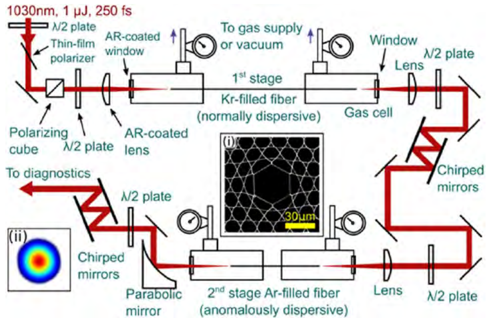
Fig. 3.13. Setup of the double stage Kagomé-type HC-PCF compression which was pumped by the oscillator introduced in section 2.1. Inset (i) shows the cross-section of the fiber with a bore diameter of 36 \mu\text{m} . It was measured in Erlangen with a scanning electron microscope. Inset (ii) shows the measured beam profile of the compressed output which was measured with a CCD camera.
