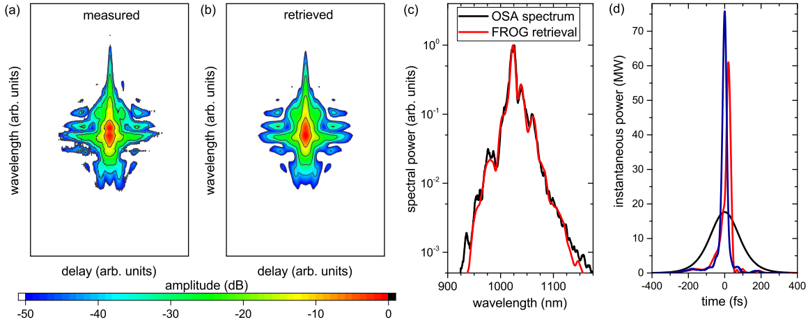
Fig. 3.34. (a) measured and (b) retrieved FROG traces of the compressed pulse after the third broadening stage. The scale is logarithmic. The retrieval grid was 512 \times 512 , the delay spacing 2 fs and the wavelength spacing 0.26 nm. The FROG error of the retrieval was 0.3%. (c) Spectrum measured with an OSA compared to retrieved FROG spectrum of the trace from (b). The scale is also logarithmic. The homogeneity of the beam is evidenced by the excellent agreement between the FROG and OSA spectrum. Since the FROG contains an only 10 \mu\text{m} thick BBO crystal, it behaves like a spatial filter (cf. Fig. 3.23(b)). (d) Instantaneous power of the 90 W average power oscillator output pulses (black line), the 70 W average power compressed pulses after the third stage (red line) and the simulated pulses which were compressed by two bounces off chirped mirrors with tailored GDD (blue line)
