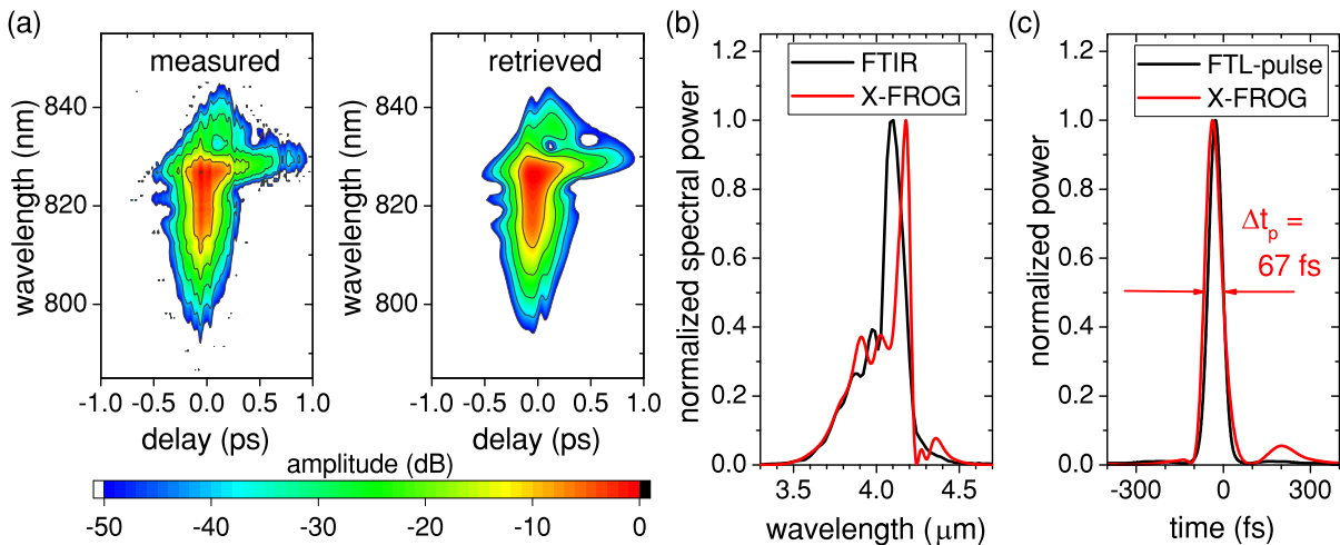
Fig. 4.23. (a) Measured and retrieved FROG traces of the spectrally broadened mid-IR pulses after dispersion compensation. The grid size was 512^2 , the residual FROG error 0.5%. No marginal was enforced for the FROG retrieval. The traces show that the central part of the mid-IR spectrum is not ideally in phase with respect to the broadened parts. That is a typical phenomenon of single-stage bulk compression (cf. section 3.2.1) (b) Comparison between the retrieved FROG spectrum and the spectrum measured with an FTIR (Lasnix L-FTS). The peak of the X-FROG spectrum is red-shifted and the \text{CO}_2 absorptions are more pronounced (due to the longer propagation length to the nonlinear crystal than to the FTIR detector). Otherwise, the agreement is also good and FTLs are nearly identical. (c) Pure material dispersion also led to a good compression of the spectrally broadened pulses which are nearly Fourier limited as the comparison of the red and the black curve shows.
