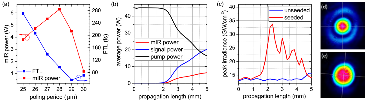
Fig. 4.6. (a) Simulated average powers and FTLs for different poling periods of the PPLN OPA. (b) Evolution of the pump, signal and mid-IR power inside a PPLN crystal with 28 \mu\text{m} poling period. (c) Evolution of the peak irradiance inside a PPLN crystal with 28 \mu\text{m} poling period for a seeded OPA (red solid line) and solely the pump radiation (blue solid line). The results shown in (a)-(c) were obtained with a 5 mm thick PPLN crystal and 45 W of pump power focused to a diameter of 300 \mu\text{m} . (d) Pump beam profile measured with a CCD camera behind the seeded OPA. (e) Pump beam profile if seed was blocked. The profiles shown in (d)-(e) were obtained with a 5 mm thick PPLN crystal and 5 W of pump power focused to a diameter of 120 \mu\text{m} .
