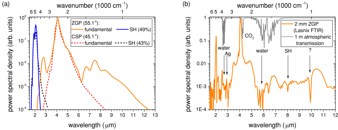
Fig. 4.21. (a) Simulations of continuum generation in ZGP and CSP which motivated the experimental investigation of the approach. The simulations assumed a \text{sech}^2 -shaped 100 nJ, 100 fs pulse centered at 4.1 \mu\text{m} and focused to a peak irradiance of 50 \text{ GW}/\text{cm}^2 . The crystal thickness was chosen to be 3 mm. SHG in ZGP ( d_{\text{eff}} \approx 76.2 \text{ pm}/\text{V} ) is phase-matched at about \theta = 56^\circ (cf. Fig. 4.20(b)) while SHG in CSP is phase-matched at about \theta = 46^\circ ( d_{\text{eff}} \approx 38.8 \text{ pm}/\text{V} ) 428 . Consequently, the shown spectra were predicted for negative effective n_2 at the central wavelength. The simulation results for both crystals exhibit significant spectral broadening, but the ZGP spectrum extends much further into the long-wave infrared. The conversion to the SH is in both cases more than 40% which is a consequence of the need to tune the crystal close to the resonance in order to achieve large effective n_2 values. (b) Experimentally obtained spectra from SCG with the compressed idler output of the OPA and a 2 mm ZGP crystal cut at \theta = 55^\circ . The peak irradiance of the pulse is about 75 \text{ GW}/\text{cm}^2 . A weak supercontinuum can be inferred from the measured spectrum. It is, however, mostly at about -30 dB of the peak power spectral density. Some expected prominent absorption features, which are indicated by the black arrows, can be qualitatively deduced from the spectrum (Ag - reduced reflection of protected silver mirrors, SH - phase-matched SHG in the ZGP crystal at \theta = 55^\circ , cf. Fig. 4.20(a)). In particular, the feature at about 10 \mu\text{m} is, however, unexpected and may result from some measurement error of the FTIR. Generally, the direct SCG with the OPA output was difficult to detect.
