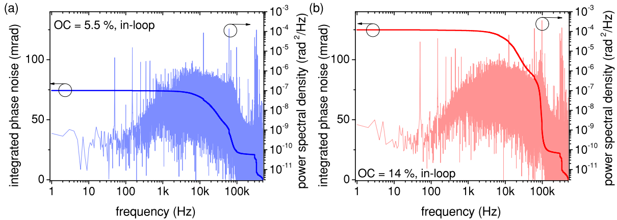
Fig. 2.21. (a) In-loop beat signal stabilization of the KLM TD oscillator with a 5.5% OC and (b) with a 14% OC. Residual phase noise as low as 75 mrad for the lower output coupling and 125 mrad for the higher output coupling were reached in the bandwidth from 1 Hz to 500 kHz. The main difference in phase noise accumulates around 90 kHz. Due to the increasing phase lag of the feedback, the servo loop becomes resonant at this frequency. The noise spike around 330 kHz originated from the DPD electronics. The best corner frequency settings were f_{11} = 20 kHz, f_{12} = 5 kHz or f_{12} = 10 kHz and f_D = 50 kHz.
