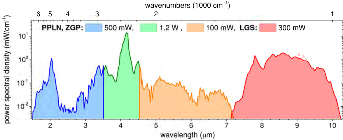
Fig. 4.25. Coverage of the mid-IR spectral region from 1.6 \mu\text{m} - 10.2 \mu\text{m} . Blue, green and orange areas represent a spectrum measurement after SCG in ZGP with a measured total power of 1.8 W. The spectrum was measured about 1.5 m away from the ZGP crystals and partly shows strong attenuation due to atmospheric absorptions. The average powers were measured behind the collimation parabolic mirror. A short pass (blue area) and a long pass (orange area) were used to measure the power of the individual components. The -30 dB width, corresponding to a power spectral density of about 10 \mu\text{W}/\text{cm}^{-1} , ranges from 1.6 \mu\text{m} - 7.1 \mu\text{m} . The red area shows the spectrum generated from an LGS OPA with a measured output power of 300 mW, extending the spectral coverage to 10.2 \mu\text{m} , i.e. over 2.7 octaves in total.
