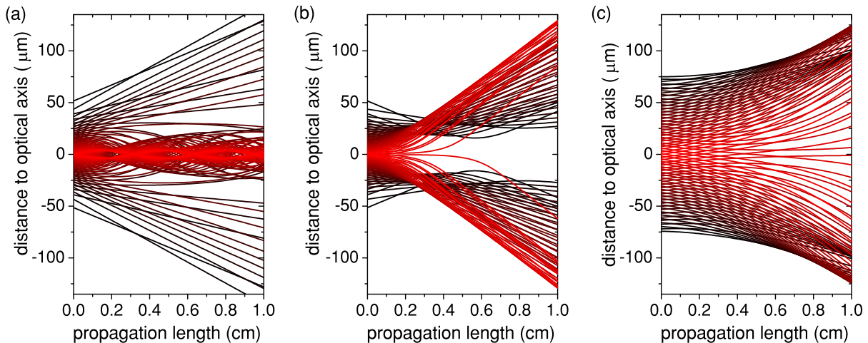
Fig. 3.28. Model for 100 rays describing a Gaussian beam. The darker the rays the larger the initial distance to the optical axis. (a) Self-focusing nonlinearity and beam divergence: The central rays stay close to the optical axis while the outer rays diverge strongly. (b) Self-defocusing nonlinearity and beam convergence: The inner rays are diffracted out of the inner beam region while the outer rays move towards the beam centre. (c) Self-defocusing nonlinearity, no divergence: the mixing of outer and inner rays is clearly reduced in comparison to (b). For all cases, an initial peak irradiance of 200 \text{ GW/cm}^2 was assumed.
