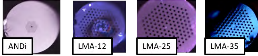
Fig. 3.5. Microscope images of the front fiber facets after damage. While the core of the ANDi and the LMA-12 fibers show severe modifications, the facets of LMA-25 and LMA-35 exhibit no sign of damage.
