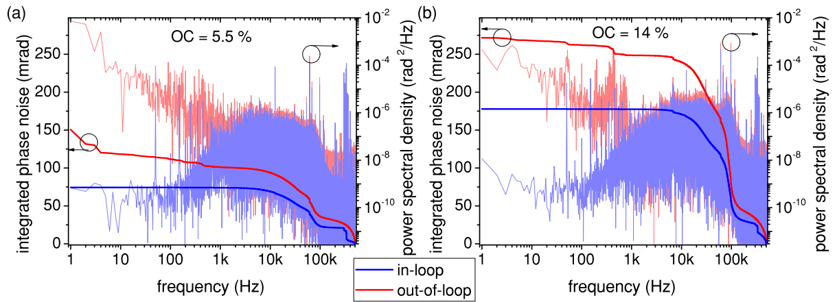
Fig. 2.23. (a) In-loop and out-of-loop beat signal stabilization of the KLM TD oscillator with a 5.5% OC and (b) with a 14% OC. Residual out-of-loop phase noise of 150 mrad for the lower output coupling and 270 mrad for the higher output coupling were reached in the bandwidth from 1 Hz to 500 kHz. The in-loop measurements were done as described before. The out-of-loop phase error was measured with an analog phase detector. It has a lower capture range than the DPD and is also sensitive to amplitude fluctuations but does not show noise spike around 330 kHz.
