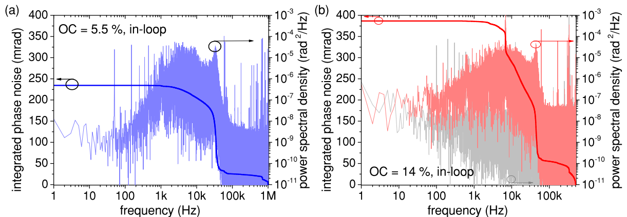
Fig. 3.38. Residual in-loop phase noise for (a) the 5.5% OC and (b) the 14% OC in a bandwidth from 1 Hz to 500 kHz. In (b), the noise floor PSD is displayed in gray. Measurements were taken with a DPD. For (a), the cut-off frequencies of the integral parts were 2 and 10 kHz, and the cut-on of the differential part was 50 kHz. For (b), the cut-off frequencies were 200 Hz and 5 kHz while the cut-on frequency was set to 20 kHz. The same PLF was used in both measurements.
