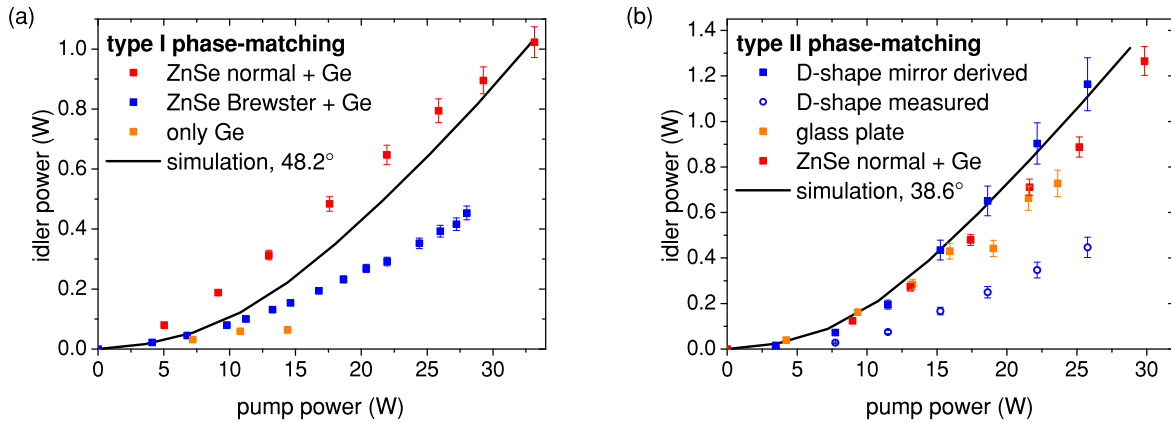
Fig. 4.15. (a) mid-IR generation with type I phase-matched 8 mm thick LGS crystals. The orange dots show a measurement were pump, seed and idler were sent onto a germanium plate to split the near-IR from the mid-IR. At pump powers above 10 W, the germanium plate becomes increasingly opaque for the mid-IR, most probably due to free carriers in the semiconductor. The blue dots were measured with ZnSe plate at BREWSTER's angle which transmitted the pump and reflected about 60 % of signal and idler. These two beams were split with a germanium plate. At low powers, the agreement with the simulation results is good while the experimental values remain behind their expectations at higher pump powers. For the measurement symbolized by the red dots, an AR coated crystal was used, allowing to pump with up to 33 W. In this case, beam splitting was accomplished by a ZnSe wedge with near-0 AOI (yielding about 17 % reflectivity), an AR-coated ZnSe plate for further attenuation of the near-IR and a Ge plate. The idler powers are partly above the expectations of the simulation which might originate from additional seed power due to excellent coupling into the LMA-12. At full pump power, 1 W of mid-IR was generated. The graph corrects for the FRESNEL reflection. An mid-IR transmission of 47 % (infinite number of reflections) was assumed for the Ge plate. (b) mid-IR generation with a type II phase-matched 7 mm thick AR-coated LGS crystal. The red dots have been measured with the same method that yielded 1 W for the type I crystal. In this case, up to 1.3 W could be generated at full pump power. The orange dots were derived from measuring first the total transmitted power and then the transmitted near-IR power while the mid-IR was blocked by a 5 mm thick FS plate. Its power was derived from the difference of both measurements. A maximal pump power of 24 W could be used due to the detection limit of the thermal power meter. The blue dots were derived from spatially splitting near-IR and mid-IR beams with a D-shape mirror. Due to the at least seven times larger diffraction of the mid-IR, parts of it passed the D-shape mirror which completely reflected the near-IR. The measurement was calibrated at low pump powers by inserting an additional Ge plate and comparing the measured idler power with and without the D-shape mirror. All solid dots symbolize the derived generated idler power. The blue hollow dots show actual power measurements, yielding 450 mW. The error bars refer to the uncertainties of the measurement method, not to a statistical analysis of a measurement set. The dark power (arising e.g. from heating the Ge plate) was subtracted from the shown idler powers. It was measured when pump and seed were delayed such that they were not mixed anymore. Phase-matching was adjusted for maximal output power.
