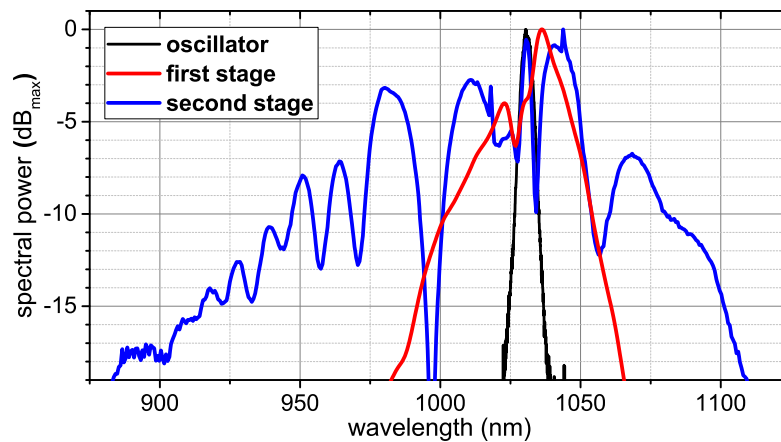
Fig. 3.22. Double stage spectral broadening. The FTL is reduced from 250 fs to 15 fs after the second stage and an intermediate compression by means of chirped mirrors.
