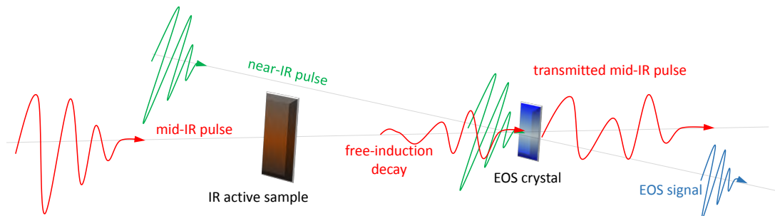
Fig. 5.2. Generic setup of field-resolved spectroscopy. A short mid-IR pulse passes the sample under test and is reshaped through dispersion and absorption. The free-induction decay of the vibrationally excited sample follows. It is up-converted via sum-frequency generation with an ultrashort (known) near-IR pulse. The up-converted signal generates together with the (filtered) near-IR pulse the EOS signal. By varying the delay between mid-IR and near-IR pulses, the full electric field of the free-induction decay is recovered.
