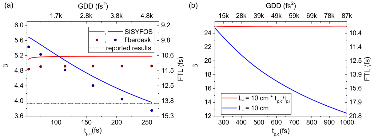
Fig. 3.7. (a) Simulated broadening factors for the data provided in ref. 206 for a fixed fiber length of L_f = 3 cm (stated in the publication, blue line and dots) and for L_f = 3 \text{ cm} \cdot t_{p,c}/55 fs. Two simulation packages were used: 50 data points were simulated with SISYFOS and 6 data points with fiberdesk V. 2.0. The results qualitatively agree well, just differ < 10\% in \beta . SISYFOS used 4 times the temporal grid points (8192) and the full Sellmeier equation of FS which may explain the slight differences. For comparison, the reported results from GANZ et al. are shown. (b) SISYFOS simulations for the LMA-35 experiments of section 2.2.1, predicting the possibility of increasing the pulse energy inversely proportional to the pulse duration. The FTLs were determined by dividing the initial pulse duration by the broadening factor. Hence, they may not be fully accurate as they refer to FWHM and the broadening factors to the RMS spectral widths in the presented plots. The top x-axes show the GDDs which are needed to achieve the pulse duration on the lower x-axes.
