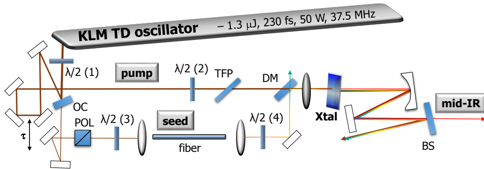
Fig. 4.1. The KLM TD oscillator delivers 1.3 \mu\text{J} pulses of 230 fs duration with a 37.5 MHz repetition rate. A dielectric mirror (OC) splits either 3% or 15% of the oscillator power. The reflected light can be attenuated by a half-wave plate ( \lambda/2 ), thin-film polarizer (TFP) sequence and is directly used to pump the nonlinear crystal (xtal). Either PPLN or lithium gallium sulfide, \text{LiGaS}_2 (LGS) was used. The seed generation is accomplished in either a polarization maintaining ANDi or an LMA-12 fiber. To suppress cross-phase modulation, the polarization is cleaned in front of the fiber with a polarizer (POL). Aspheric lenses were used for coupling and collimation. The long wavelengths of the continuum and the pump are overlapped in space with a dichroic mirror (DM) and in time with a translation stage in the pump arm ( \tau ). The polarizations of seed and pump are optimized for maximal conversion to the mid-IR. After the nonlinear crystal, the beams are collimated. The mid-IR is separated by means of a beam splitter (BS) which was coated in-house. The mirrors in the pump arm and in front of the fiber were dielectric, the others metallic.
