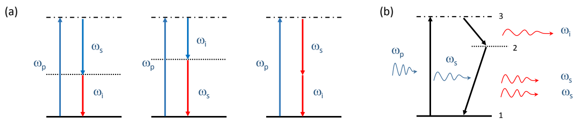
Fig. 1.10. (a) Difference frequency generation schemes. The first two graphs are taken from ref. 183. The leftmost scheme illustrates the generation of an idler photon ( \omega_i ), from a pump photon ( \omega_p ). The process is seeded by a signal photon ( \omega_s ). Vice versa, the middle graph shows the generation of a signal photon seeded by an idler photon. The rightmost graph illustrates the spontaneous decay of a high energy pump photon into lower energy signal and idler photons. In this case, energy conservation is obvious. In the other graphs, the two outgoing seed photons are not explicitly shown. This stimulated process becomes clearer in (b) where the analogy to a laser gain medium is drawn. The pump photon excites the virtual laser level 3 which instantaneously relaxes to the virtual level 2 under the emission of an idler photon. At the same time, a seed photon causes the emission of a second identical (in phase and energy) signal photon.
