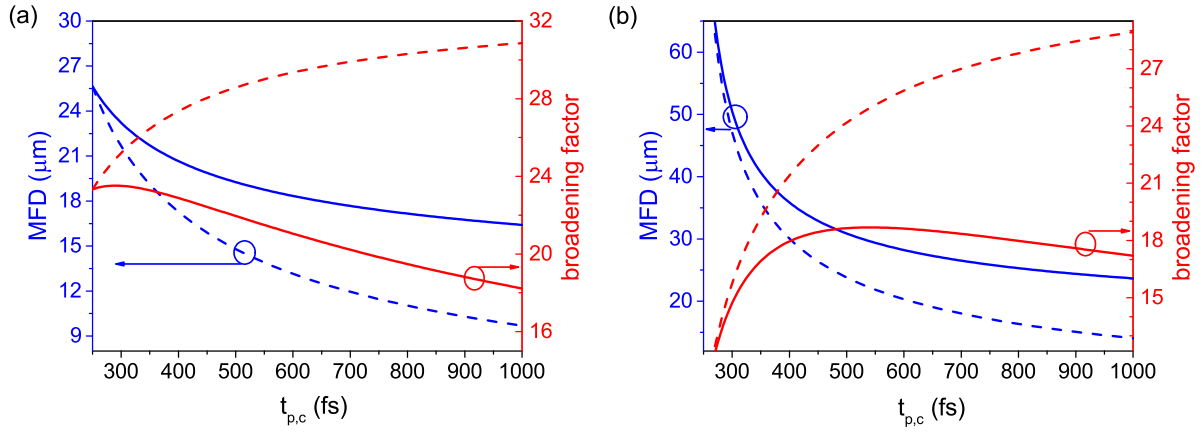
Fig. 3.9. MFDs and broadening factors for various input pulse durations t_{p,c} derived from Eqs. (3.1) and (3.6) where t_{p,i} = 250 fs, \text{GVD} = 19 \text{ fs}^2/\text{mm} , \lambda = 1030 nm, n_2 = 2.8 \cdot 10^{-16} \text{ cm}^2/\text{W} and P_{cr} = 4 MW. (a) An initial peak power of P_{p,i} = 2 MW is set. The solid lines show the predicted results. The dashed lines compare these results to a pulse duration- independent damage threshold. The MFDs are different due to the different damage irradiances. Prechirping hardly increases the maximum broadening factor if the damage irradiance scales \propto t_p^{-3/4} . (b) An initial peak power of P_{p,i} \approx 4 MW is set, being close to the critical power. In this case, an optimal chirp and MFD can be derived, indicating possible applicability of CPSB. Solid lines again represent the pulse duration-dependent damage threshold while dashed lines represent the pulse duration- independent one.
