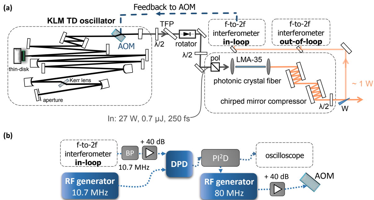
Fig. 2.20. (a) CEP stabilization setup. Oscillator and fiber compression stage are almost as before (cf. Fig. 2.7, \lambda/2 - half-wave plate, TFP - thin-film polarizer, pol - polarizing beam splitting cube), just an AOM was inserted into the oscillator next to the output coupler. It was placed at BREWSTER'S angle. For initial experiments the 5.5% OC was used, otherwise the 14% OC. In the former case, the pulses emerging from the compression stage were about 40 fs long. This was still short enough to the generated a coherent supercontinuum in the highly nonlinear PCFs. The power sent into the interferometers was adjusted by a half-wave plate and a wedge (W) with 45^\circ to 55^\circ AOI. Two f-to-2f interferometers were set up. The in-loop interferometer provided feedback to the AOM while the out-of-loop interferometer analyzed the residual CEP noise. The dashed line indicating the electronic feedback is explained in more detail in (b). The beat signal was electronically band-passed (central frequency 10.7 MHz, bandwidth 2 MHz) to suppress the signal originating from the laser repetition rate. The beat signal was amplified afterwards and compared to a reference stemming from a RF generator by a digital phase detector (DPD) in the in-loop interferometer and a analog phase-detector in the out-of-loop interferometer. The error signal originating from the phase-difference was sent to a PI 2 D controller and monitored in parallel. The signal of the servo controller modulated the 80 MHz RF signal that drove the AOM.
