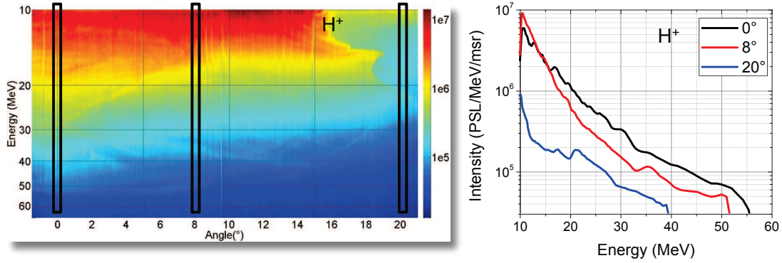
Figure 3.22: a) Angularly resolved proton spectrum measured with the iWASP. The 3 black rectangles represent typical angles of TP measurements. b) averaged spectra obtained from these 3 rectangles as they would have been seen by TP-spectrometers at these angles, showing significant differences in the spectral shape and cutoff energy.
