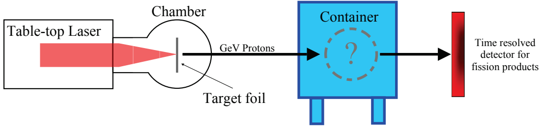
Figure 1.3: Schematic depiction of a laser-driven active interrogation, where the high energy proton beam is used to probe an container for fissile material.
