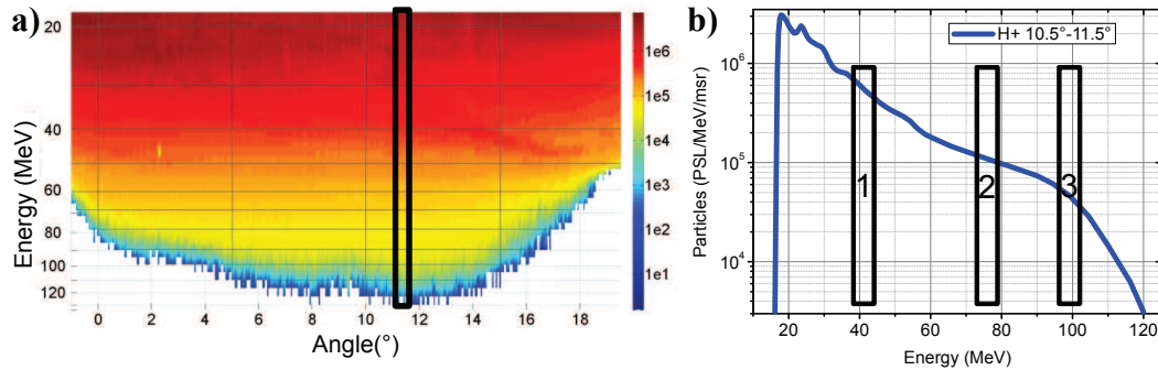
Figure 4.24: a) Angularly resolved proton spectrum measured at Trident from a CH 2 target measured with the iWASP (see text for details). b) averaged spectrum between 10.5° and 11.5° with a cutoff energy exceeding 100 MeV.
