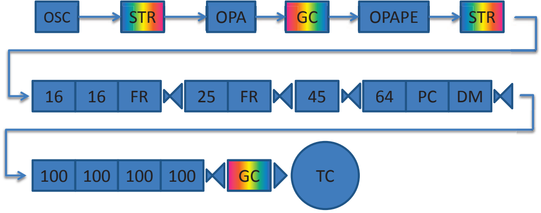
Figure 3.2: Trident laser schematics with “OSC” the seed oscillator, “STR” and “GC” the stretcher and compressor, respectively; with “OPA” and “OPAPE” the optical parametric amplifier and cleaner stage, “DM” the deformable mirror, “FR” a Faraday rotator and “TC” the target chamber. The numbered boxes are amplifier rods/discs of the same size.
