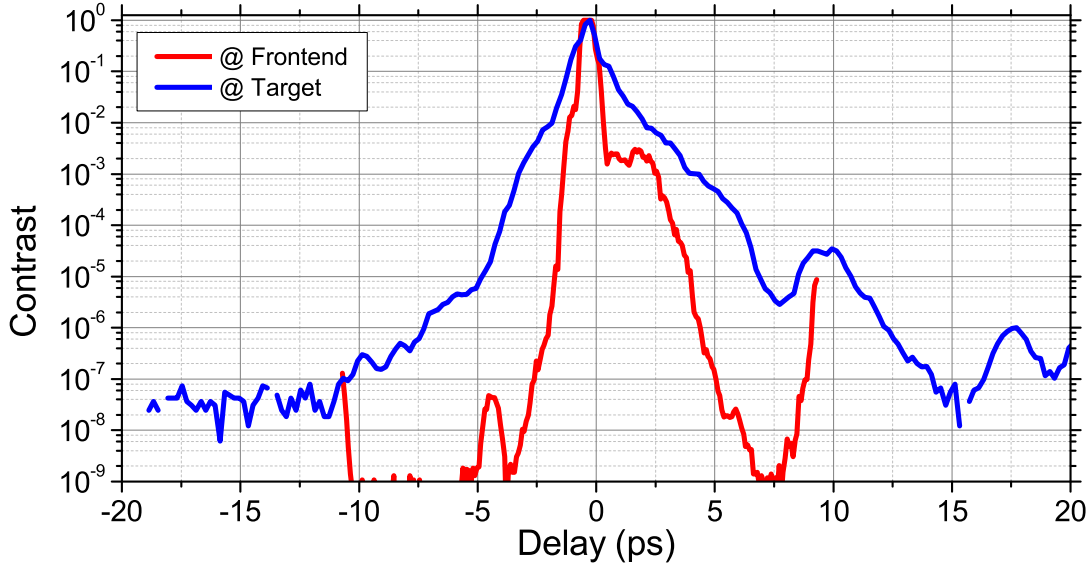
Figure 3.6: Typical contrast of the Trident laser as measured by a scanning-autocorrelator at the front-end (red solid line) and at the target chamber without charging the amplifiers (blue solid line). The decreased contrast at the target side results most likely from imperfect recompression in the final grating compressor.
