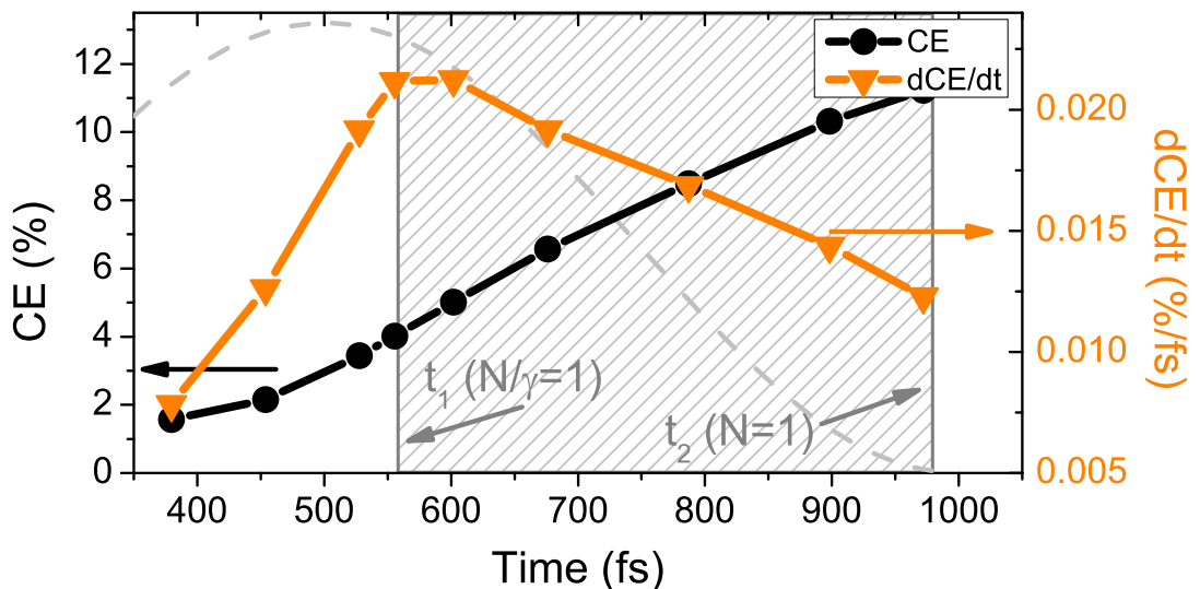
Figure 4.19: Time dependent CE as obtained from 2D-VPIC simulation for a 120 nm target, with the conversion efficiency over t (black circles) and dCE/dt over t (orange triangles). The grayed area (550 fs to 990 fs) indicates the time of relativistic transparency during the simulation. The simulation domain is 20 \mu\text{m} \times 25 \mu\text{m} in the (x, z) plane, the laser pulse has a time-varying intensity I(t) = I_0 \sin^2(t\pi/\tau) with I_0 = 2.0 \times 10^{20} \text{ W/cm}^2 and \tau/2 is the FWHM (500 fs, \lambda=1054 \text{ nm} ) and propagates along x . The laser pulse is Gaussian-shaped with best focus at the target surface with E_y, E_z \sim \exp(-z^2/w^2) with w = 6.8 \mu\text{m} . The targets ( \text{C}^{6+} with 5% protons in number density) are of solid density N = 821 ( 2.8 \text{ g/cm}^3 ) with a step-function density profile at the beginning of the simulation. The cell size is \Delta x = 0.3\lambda_D^0 (0.3 nm) and \Delta z = 1.7\lambda_D^0 ; 500 electrons per cell are used ( T_e = 18 \text{ keV} and T_i = 10 \text{ eV} for carbon ions and protons, initially). (Figure and caption adapted from Jung, et. al. [166])
