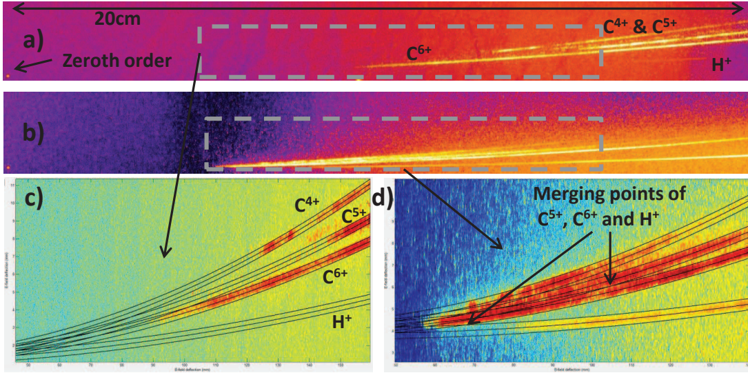
Figure 3.17: Comparison of ion spectra with identical high energy cut-off for C^{6+} (280MeV) and C^{5+} (120MeV) obtained using the novel high resolution and high separation TP with different drift and electric field to demonstrate influence on merging of traces: a) spectrum obtained using appropriate parameters (25 kV/2cm over 20 cm and 50 cm drift) to resolve different traces as shown in c); b) spectrum obtained with too low dispersion (15 kV/2 cm over 20 cm and 30 cm drift) resulting in premature merging of traces as shown in d); low to high energy from right to left side of each image, black lines in c) and d) are predicted traces with upper and lower boundaries. (Figure and caption adapted from Jung, et al. [150])
