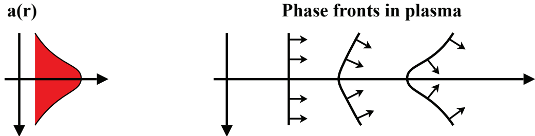
Figure 2.3: Self-focusing in a relativistic plasma due to a transverse gradient in the refractive index causing slower group velocity v_p on-axis than off-axis (Adaption of Ref. [65])
