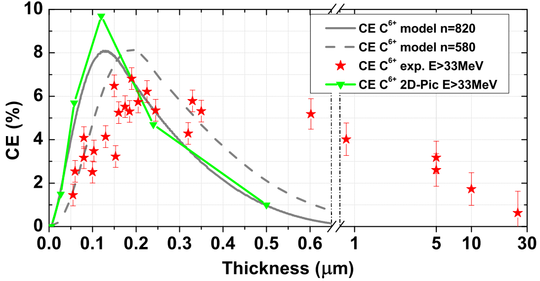
Figure 4.20: Thickness scaling of the CE as obtained from the experiment with ion energies greater than 33 MeV (red stars) in comparison with 2D-PIC simulation (green triangles with E > 33 MeV) and the model using an initial normalized critical density of 820 (gray solid line) and 580 (gray dashed line) to account for expansion of the target under the laser pedestal. Note, that the model loses its applicability in the TNSA dominated regime ( d > \sim 700 nm for Trident parameters). (Figure and caption adapted from Jung, et. al. [166])
