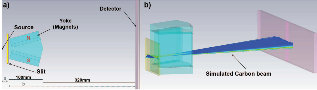
Figure 3.19: a) Top view of the ion wide angle spectrometer (iWASP), with from left to right, the source, the slit, the yoke and the detector. b) Side view showing a simulated trace of carbon C^{6+} ions calculated with CST[158]. (Figure and caption adapted from Jung, et al. [157])
