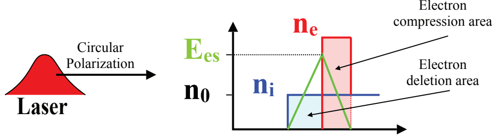
Figure 2.5: Schematic picture of the RPA. Due to the CP laser light, electron heating mechanisms are suppressed and electrons are pushed into the target until the charge separation field balances the radiation pressure. This forms an electron depletion area and an electron compression area. Ions from the latter are accelerated into a mono-energetic spectrum by successive propagation through the target and cycling in the charge separation field E_s . (Adaption of [14])
