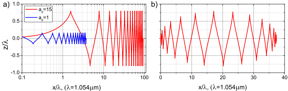
Figure 2.1: a) Electron motion in an infinite plane wave with LP and an a_0 = 1 (blue) and a_0 = 15 (red), where the highly relativistic laser amplitude of 15 strongly bents the electron motion into the laser propagation direction; b) Electron motion in a finite plane wave with a Gaussian envelope and an a_0 = 15 , showing that there is no net energy transfer to the electron (in the case of a single electron in vacuum).
