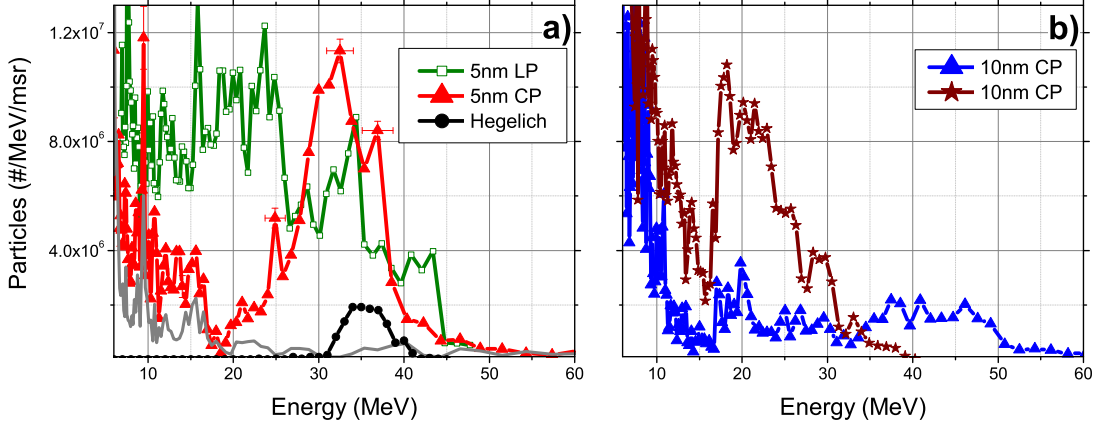
Figure 4.28: a) Carbon C^{6+} spectra measured with CP (spectrum with red triangles, signal noise with gray solid line) and LP (green squares) from a 5 nm DLC foil target and the carbon spectrum obtained from a 10\ \mu\text{m} Ti target as published in Hegelich et al. [26]; b) Carbon C^{6+} spectra measured with CP from two different shots on 10 nm DLC showing deterioration of the monoenergetic structure at increased target thickness as BOA-soliton conditions are not met anymore. (Figure and caption from Jung, et al. [34])
