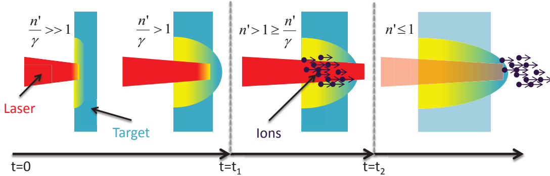
Figure 2.7: Sketch of the Break-out Afterburner: In the time between t = 0 and t = t_1 the target is volumetrically heated and all electrons are subsequently promoted to hot electrons. At t = t_1 the plasma density has dropped to n' > 1 > n'/\gamma and the target turns relativistically transparent to the laser light. It follows a period of rapid and extreme ion acceleration, where the electrons energy is continuously replenished by the laser light. The acceleration ceases when the target turns classically underdense at t = t_2 due to the strong expansion of the plasma with N < 1 .
