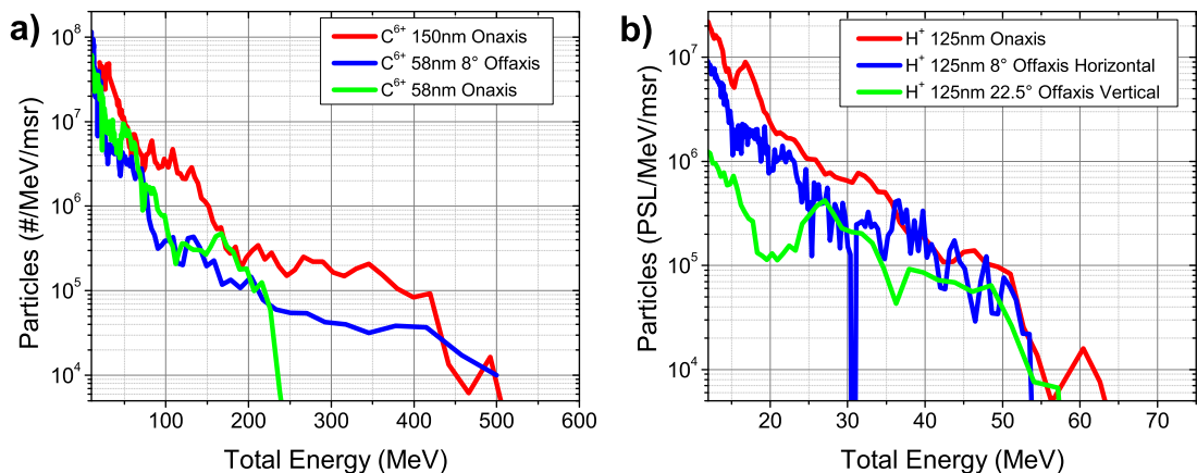
Figure 4.2: Particle spectra measured by TPs at different angles for shots that yielded peak energies a) for carbon C^{6+} ions and b) for protons.
