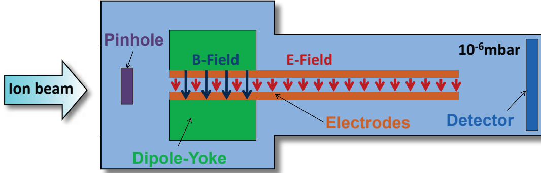
Figure 3.14: Sketch of a standard Thomson parabola, where the parallel magnetic and electric fields are perpendicular to the ion propagation direction. Ions are detected at the detector plane on parabolically shaped lines. (Figure and caption adapted from Jung, et al. [150])
