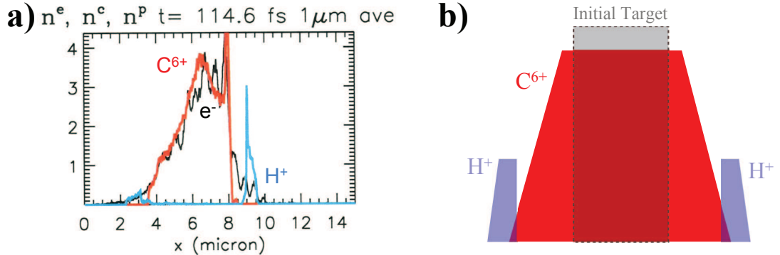
Figure 4.9: a) Snapshot of a 2D VPIC simulation showing the electron (black solid line), carbon C^{6+} (red solid line) and proton (blue solid line) density during the BOA acceleration. The depletion of protons in the target is caused by self-cleaning of the target due to the high charge to mass ratio and low inertia of protons. The self cleaning is sketched in b) and results in different acceleration dynamics for the protons (see text for details).
