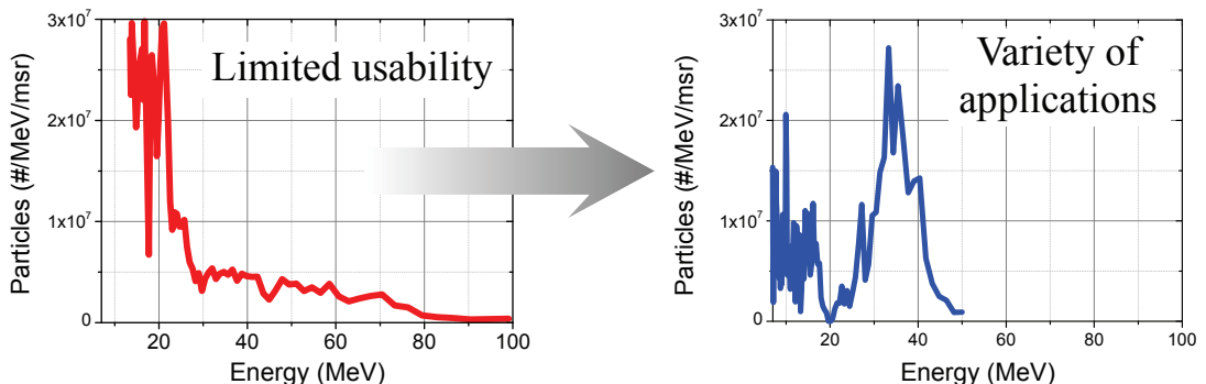
Figure 4.25: a) exponentially decaying (see Sect. 4.2 to Sect. 4.3 for details) and b) mono-energetic ion spectra obtained at Trident (see Sect. 4.4.1 for details), where the latter is preferred for most applications using proton/ion beams.
