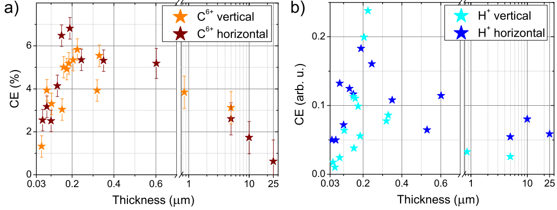
Figure 4.16: Conversion efficiencies for a) carbon C^{6+} (absolute) and b) protons (in arb. u.) for thickness from 30 nm to 25 \mu\text{m} . The conversion efficiency peaks for both species at the optimum BOA thickness d_{\text{opt}} = 200 nm, with almost 7% for C^{6+} and a 5-fold increase for protons as compared with thicknesses larger than 1 \mu\text{m} .
