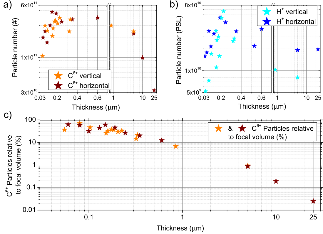
Figure 4.18: Thickness dependency of particle numbers for carbon C^{6+} a) and protons b) for thicknesses ranging from 30 nm up to 25 \mu\text{m} . The peak at 200 nm corresponds to the optimum BOA target thickness for Trident parameters. For thicknesses > 1 \mu\text{m} acceleration turns over to TNSA. Note that particle numbers for protons are given in PSL due to missing absolute calibration of the IP.
