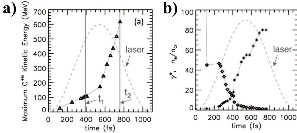
Figure 2.6: VPIC simulation results for Trident laser parameters and a 58 nm diamond like carbon target. In a) the maximum carbon C 6+ vs time (solid line with triangles) and the laser intensity envelope in arbitrary units (dashed line); between the times t_1 and t_2 90% of the energy gains occurs. In b) the related normalized electron densities (diamonds) and the electron Lorentz factor (pluses) are plotted and show that the target is relativistically transparent between the times t_1 and t_2 . (Figure adapted from Ref. [106])
