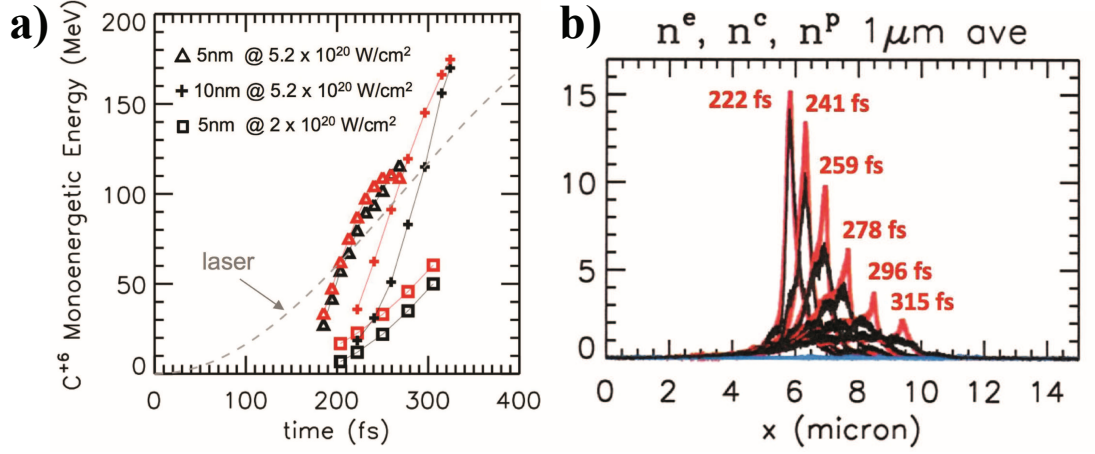
Figure 4.30: a) Results from 2D simulations for the BOA-soliton acceleration at higher laser intensities: using a 5 nm and 10 nm-thick carbon target at n'_0 = 821 and a \sin^2 square CP laser with peak intensity 5.2 \times 10^{20} \text{ W/cm}^2 (triangles and crosses), in comparison with a 5 nm thick carbon target at peak intensity 2 \times 10^{20} \text{ W/cm}^2 representing Trident parameters (squares). The soliton “energies” ( 1/2m_i v_s^2 ) are red and the ion energies black. b) Temporal evolution of the ion density spike for the 10 nm case with 5.2 \times 10^{20} \text{ W/cm}^2 with the carbon density (red) and electron density (black). (Figure from Ref. [35])
