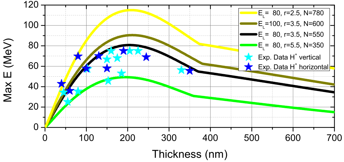
Figure 4.8: Thickness scan for protons (blue stars) measured with the iWASP covering an angle of 22^\circ in the direction parallel (light blue, marked as “vertical”) and perpendicular (blue, marked as “horizontal”) to the laser polarization axis with a solid angle of \sim 0.1 msr. The solid lines are predictions by the analytical model for different combinations of the laser energy and focus to account for variations in the laser and the target alignment. The initial target density has been adjusted to keep the optimum thickness at 200 nm (see text for details).
