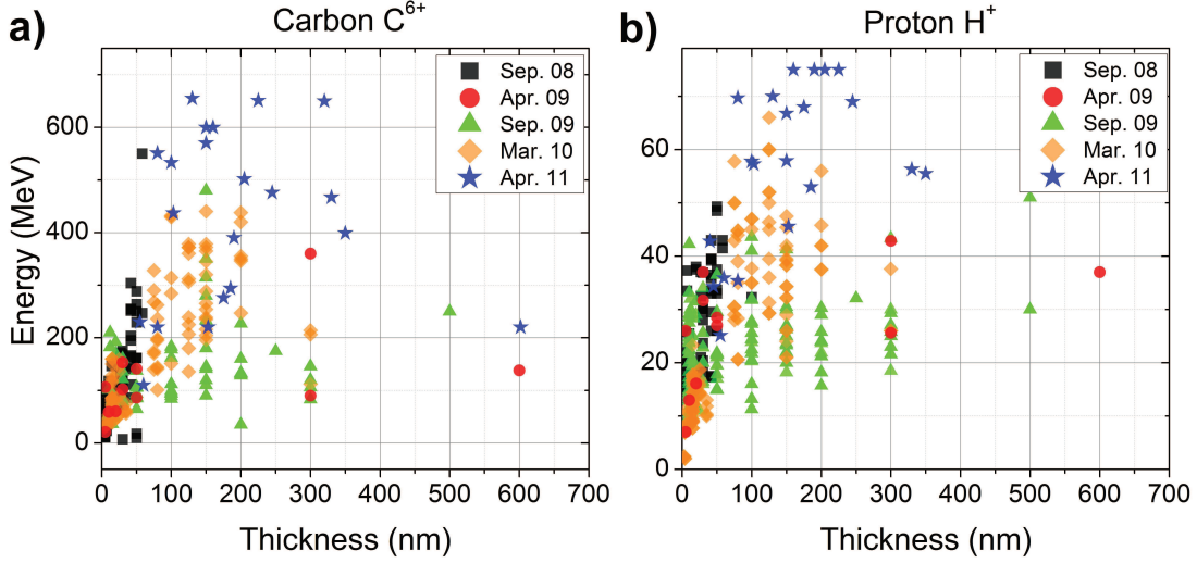
Figure 4.3: Experimental data of 5 of the 6 campaigns showing the efforts in improving repeatability and accuracy of the measured maximum carbon C^{6+} ion a) and proton b) energies. The campaigns from Apr.08 through Mar.10 were done in the TP-setup, the last one in the iWASP-setup that covers a much larger solid angle of the ion beam. Campaigns from Mar.10 on also used the improved target and focusing system as described in Chap. 3.3.
