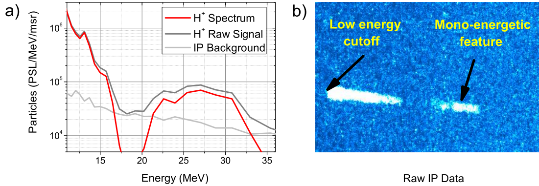
Figure 4.26: a) Mono-energetic spectrum measured at Trident with CP from a 42 nm DLC foil. The red solid line shows the raw signal (dark gray solid line) subtracted from the background (light gray solid line). The raw data measured with a TP is shown in b) with increasing energy from left to right.
