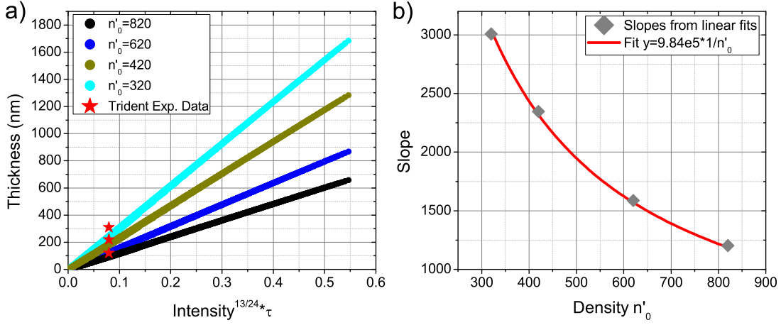
Figure 4.7: a) Results of a parametric scan of the analytical model for the BOA acceleration with different initial densities n'_0 ; maximum C^{6+} ion energies for different thicknesses are displayed as red stars, as shown in Fig. 4.6; b) Allometric fit of the slopes from a) (see text for details).
