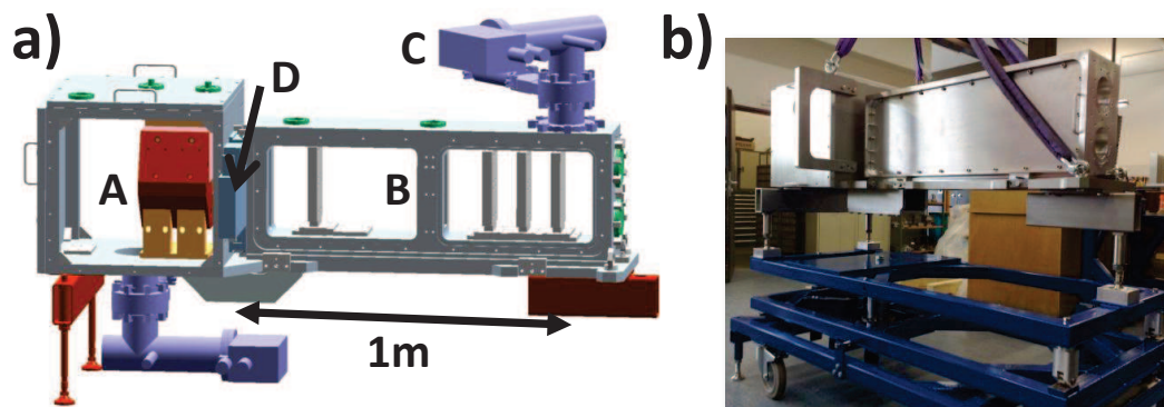
Figure 3.16: a) Schematics of the new Thomson parabola with A the core part containing the magnets and electrodes and B the drift and detector part and space for an additional pair of electrodes. Both parts are separated by a vacuum valve D and pumped by their own cryo pump C ; b) photograph of the new TP, including its 6axis support. (Figure and caption adapted from Jung, et al. [150])
