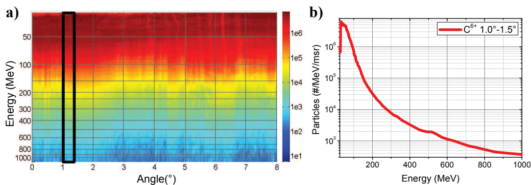
Figure 4.23: a) Angularly resolved carbon C^{6+} ions measured at Trident from a heated target measured with the iWASP. b) averaged spectrum between 1^\circ and 1.5^\circ with a cutoff energy exceeding 1 GeV.
