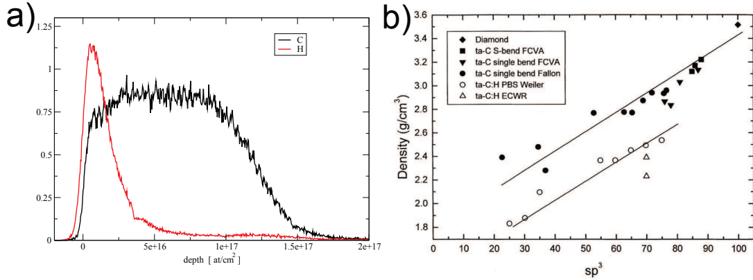
Figure 3.11: a) Preliminary ERDA measurement done at the Tandem accelerator of the Technical University of Munich (TUM) by A. Bergmaier and W. Assmann; b) graph taken from Ref. [139] showing density dependency of the sp^3 content for various DLC foils, where ta-C is hydrogen free and ta-C:H is hydrogen contaminated DLC.
