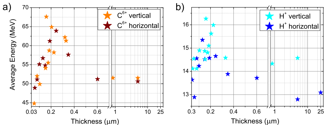
Figure 4.17: Thickness dependency of the average particle energy for carbon \text{C}^{6+} a) and protons b) for thicknesses ranging from 30 nm up to 25 \mu\text{m} . The low energy detection limit for the carbons is 33 MeV and 11 MeV for the protons. The peak at 200 nm corresponds to the optimum BOA target thickness for Trident parameters. The error for the mean ion energy is expected to be close to the instrument's energy resolution (6% for protons and 10% for carbon ions at 50 MeV/amu).
