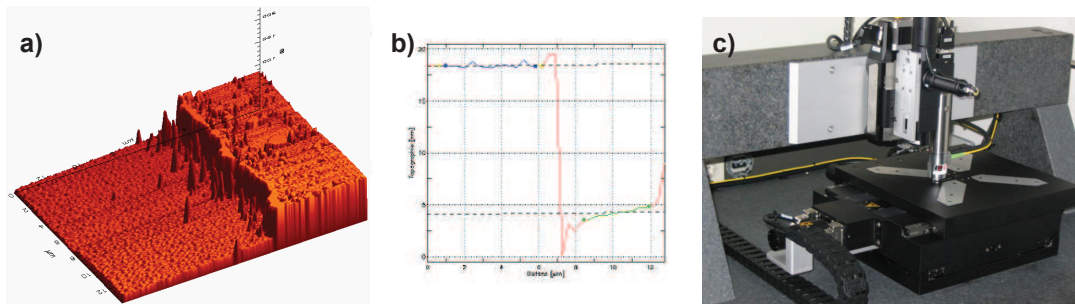
Figure 3.10: a) Topographic scan of a DLC foil at the edge of the coating and b) a lineout showing the thickness of the foil measured with c) an commercial atomic force microscope (AFM)
