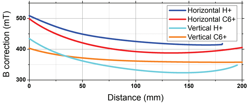
Figure 3.21: Calibration curves for the iWASP for different iWASP setups; the calibration lines have been obtained from the low energy cutoff lines of either the protons or the carbon C^{6+} ions (see Fig. 3.20).
