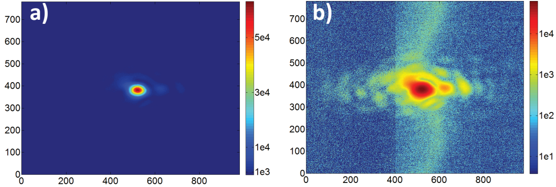
Figure 3.3: Raw image taken with the focus diagnostic camera a) with linear z -scale and b) with log z -scale. Axes are in original pixel values, where one pixel is \sim 0.086\mu\text{m} . Note, that the waved haze above and under the focus visible in image b) is an artifact, most likely resulting from working near saturation of the camera.
