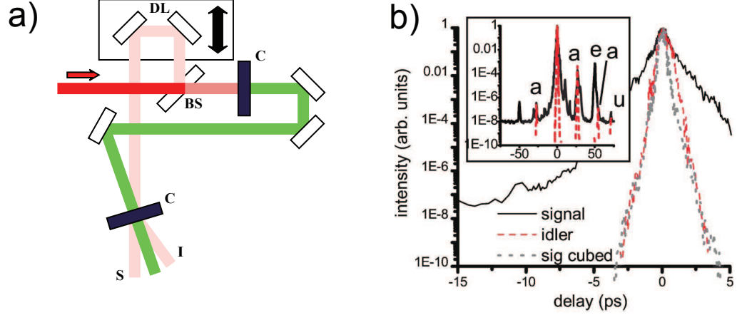
Figure 3.5: Sketch of the OPAPE cleaning technique used at Trident to improve the contrast; b) temporal contrast measurement of the signal (black solid line), the cubed signal (gray dashed line) and the idler (red dashed line). The inset shows a larger time window with some artifacts “a”, a reference pulse “e” and an unknown peak “u” (see text for details, adaption of Ref. [115]).
