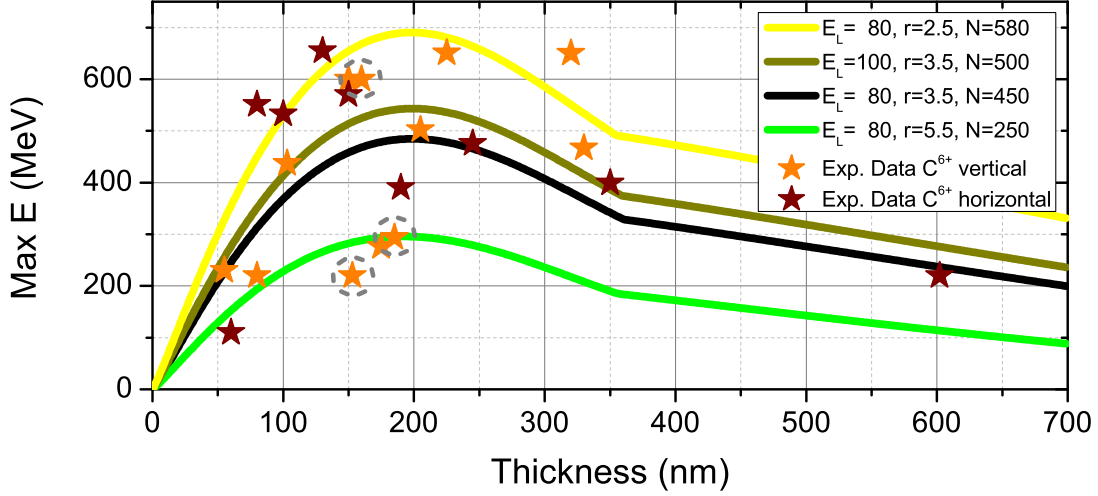
Figure 4.4: Thickness scan for carbon C^{6+} ions (red stars) measured with the iWASP covering an angle of 22^\circ in the direction parallel (orange, marked as “vertical”) and perpendicular (dark red, marked as “horizontal”) to the laser polarization axis with a solid angle of \sim 0.1 msr. The solid lines are predictions by the analytical model for different combinations of the laser energy and focus to account for variations in the laser and the target alignment. The initial target density has been adjusted to keep the optimum thickness at 200 nm (see text for details). For the three data points marked with a gray dashed circle the on-shot laser contrast is shown in Fig. 4.5 b).
