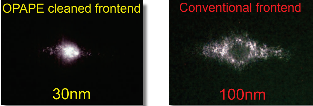
Figure 5.1: 3\omega backscatter from a 30 nm target with the OPAPE cleaned frontend (left frame) and from a 100 nm target with the old low contrast frontend. With the OPAPE cleaning the contrast is good enough, so that the main pulse still interacts with a overcritical target generating third harmonic radiation over the whole focal spot, which is measured in the backscatter diagnostic
