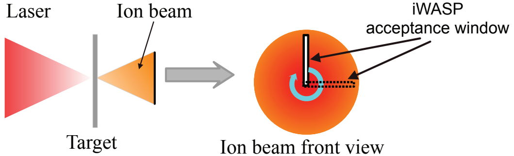
Figure 4.15: Estimating the conversion efficiency from the measurements: the conversion efficiency is calculated for the solid angle captured by the iWASP, where measurements have been done parallel and perpendicular to the polarization axis. The conversion efficiency is then “rotated” by 360^\circ assuming azimuthal symmetry of the beam (see text for details).
