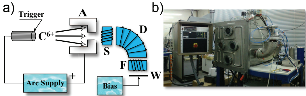
Figure 3.8: a) Sketch of the cathodic arc deposition process and b) picture of the actual setup used to fabricate diamond like carbon targets at the University of Munich.
