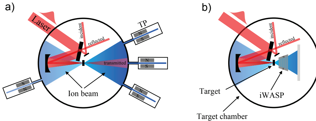
Figure 4.1: Experimental setup with a) the TP-setup, where a number of different TPs analyzes the particle beam at different positions around the target. A variety of secondary diagnostics can be employed, such as electron spectrometers and laser pulse diagnostics; b) the iWASP-setup, where the iWASP measures the ion spectra angularly resolved; due setup constraints, no other diagnostic can be used in this configuration. In both setups is the laser (CP and LP) focused by an F/3 (F/8) off-axis parabolic mirror on a nanometer-scaled diamond like target.
