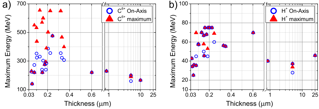
Figure 4.12: Overall maximum energies (red triangles) and cutoff energies seen on-axis at 0^\circ (blue circles) for carbon \text{C}^{6+} ions a) and protons b). For protons maximum energies are emitted on-axis regardless of the target thickness, whereas maximum carbon ion energies are emitted off-axis in the BOA regime ( \ll 1 \mu\text{m} ) and on-axis in the TNSA regime ( > 1 \mu\text{m} ).
