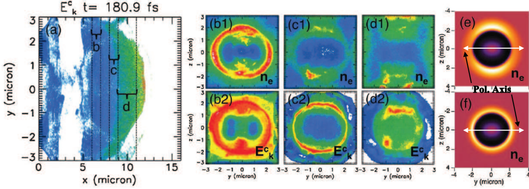
Figure 4.14: a) - d) 3D VPIC simulation results of the BOA at time t = 180.9 fs during the relativistic transparency. Panel a) shows E_k^c and depicts regions over which the data are averaged in panels b) ( x = 6 - 7 \mu\text{m} ), c) ( 8 - 9 \mu\text{m} ), and d) ( 9 - 11 \mu\text{m} ); b1) to d1) show averages of n_e and in b2) to d2) is E_k^c displayed. e) and f) shows n_e from 2D hydromodeling without and with electrostatic forces from the ions on the expelled electrons, respectively (shown after 3 fs) (Figure and caption from Ref. [164]).
