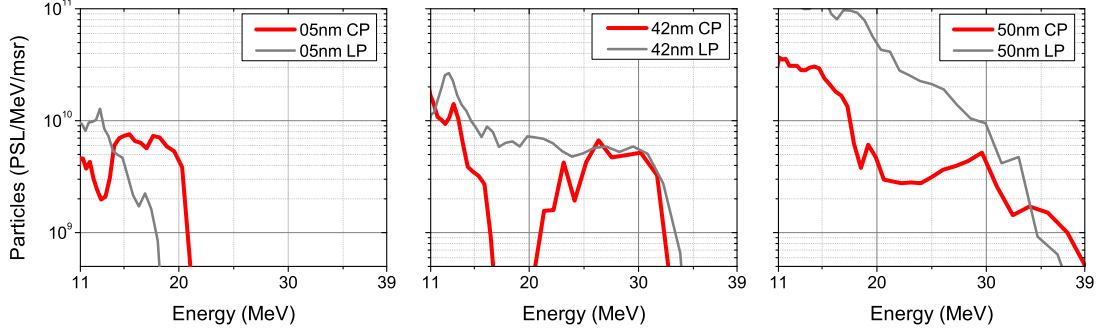
Figure 4.27: Mono-energetic spectra measured at Trident with CP (red solid line) and LP (gray solid line) from a) 5 nm, b) 42 nm and c) 50 nm DLC foil targets.
