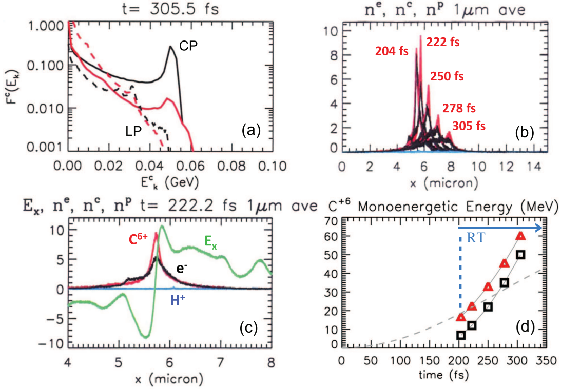
Figure 4.29: Results from a 2D simulation: (a) carbon C^{6+} spectra at 305 fs (end of the acceleration phase) for CP (solid) and LP (dashed) laser obtained along a 1-micrometer average over z centered at z = 0 (black) and from the whole simulation domain (red); (b) time evolution of carbon ion (red curves) and electron density (black), both normalized to n_{cr} , during the transparency phase (the blue trace is the proton density); (c) bipolar electric field structure in E_x (green) co-moving with the solitary carbon density spike (red); (d) monoenergetic ion energy (black squares) obtained from ion spectrum vs. time during the acceleration phase as compared with the soliton “energy” \frac{1}{2}m_i v_p^2 (red triangles) estimated from the soliton speed v_p (the laser intensity profile is indicated in arbitrary units as gray dashed line). (Figure and caption from Jung, et al. [34])
