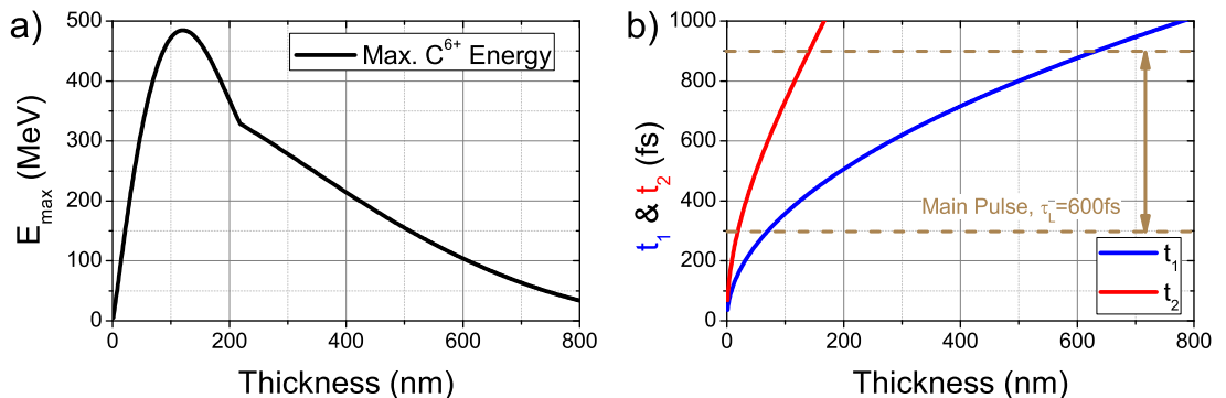
Figure 2.8: Model prediction a) of the maximum carbon C^{6+} energy vs. Thickness for Trident parameters with \tau_\lambda = 600 fs, E_L = 80 J, n'_0 = 660 , q_i = 6 for carbon C^{6+} and a(t) = a_0 \sin^2(\pi t/2\tau_\lambda) , with a_0 = 16.8 ; b) BOA acceleration times t_1 and t_2 for the same parameters
