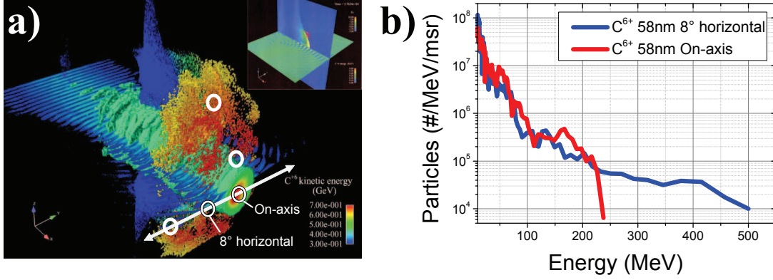
Figure 4.11: a) Snapshot of BOA acceleration in a 3D VPIC simulation, where the white line indicates the laser polarization axis and the white circles positions of TP-spectrometers in the TP-setup. The iWASP analyzed the particle beam along and perpendicular to the polarization axis. b) Typical TP-spectra measured on- and off-axis exhibiting significantly different high energy cutoffs.
