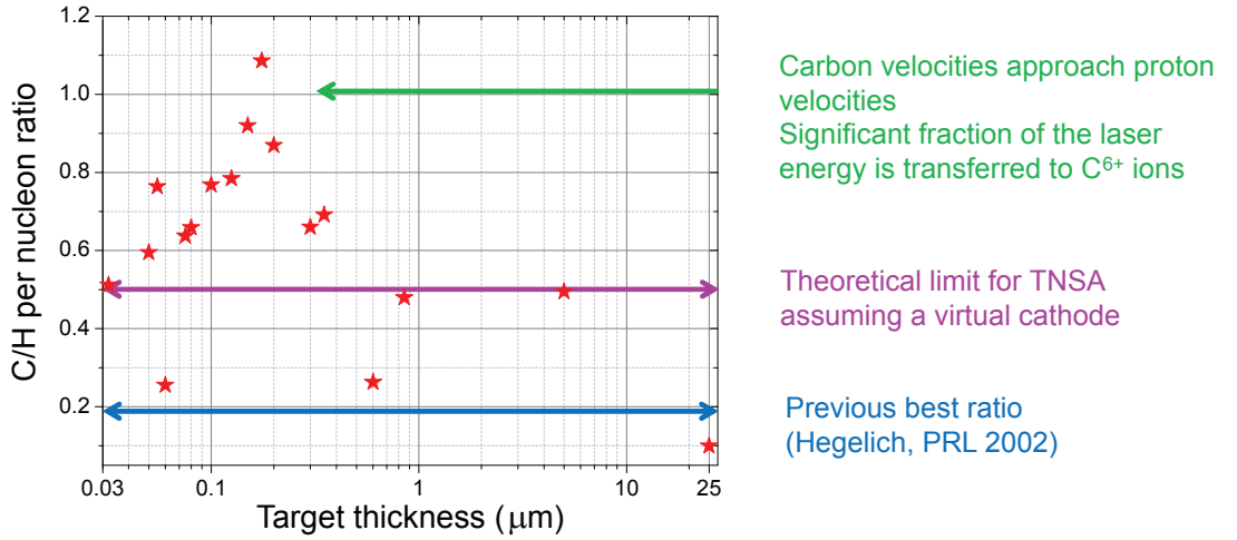
Figure 4.10: Ratios of the per nucleon energy for carbon and proton maximum energies. The ratio goes up to 1.1 at the optimum thickness, where carbon ions have a slightly higher velocity than the protons. The theoretical limit in a TNSA dominated acceleration by a virtual cathode is 0.5 and the highest experimentally measured value for TNSA is 0.2.
