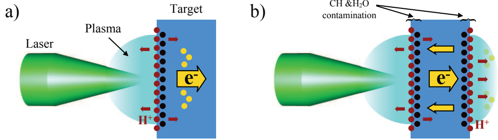
Figure 2.4: Schematic depiction of the Target Normal Sheath Acceleration (TNSA). The obliquely incident laser heats electrons on the front side of the target. The electrons penetrate the target, that is several micron thick and opaque to the laser light. A charge separation field is created by these hot electrons on the back side of the target due to subsequent field ionization of the target surface. Protons (and ions) are accelerated in this virtual cathode target normal to the back surface (see text for details).
