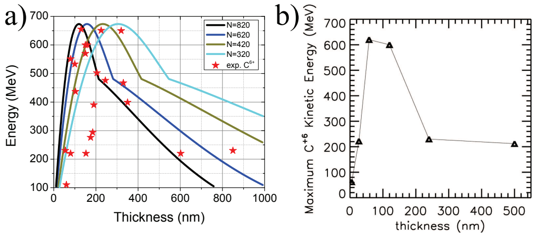
Figure 4.6: a) Maximum carbon C^{6+} ion energies measured with the iWASP (red stars) and predictions by the analytical model with optimum Trident parameters and varying initial target density to account for variations in the laser contrast and hence the pre-mature expansion of the target. b) Thickness scan as obtained from the VPIC simulations for Trident parameters and an initial density of n'_0 = 660 (left frame adapted from Ref. [106]).
