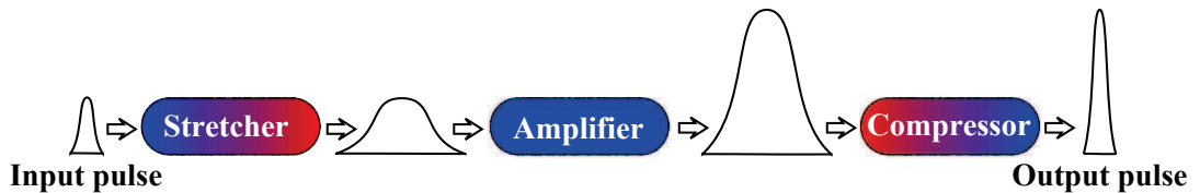
Figure 3.1: Schematic depiction of a CPA stage, where the pulse is first stretched in time, then amplified and finally recompressed.
