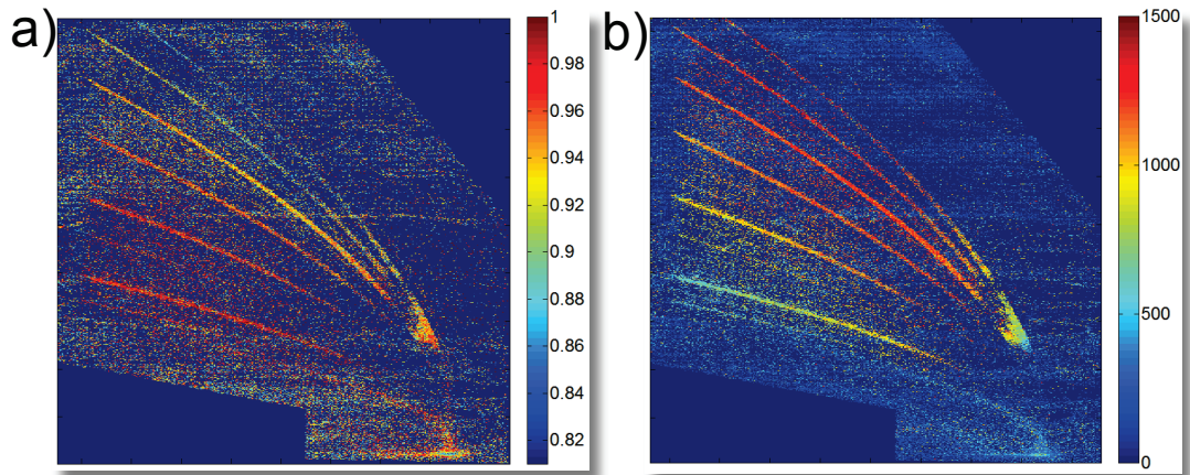
Figure 3.13: Image of an scanned CR39, showing parabolic particle tracks obtained from a Thomson parabola (see Sect. 3.4.2 for details), where in a) eccentricity is color coded in the z-axis and in b) the enclosed area of the pits (in arbitrary units).
