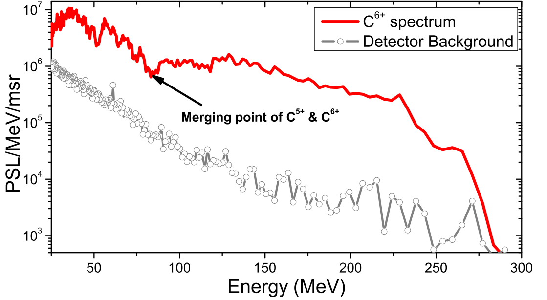
Figure 3.18: Carbon C^{6+} spectrum (red solid line) extracted from Fig. 3.17b including detector background (gray with circles) showing corruption of the spectrum after the merging of C^{5+} into C^{6+} at 80 MeV. (Figure and caption adapted from Jung, et al. [150])
