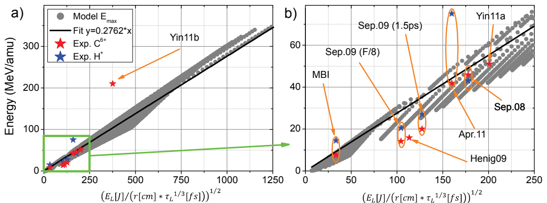
Figure 4.22: a) Parametric scan of the analytical BOA model (gray circles) plotted as maximum ion energy vs. \sqrt{E_L / (r_L \tau_L^{1/3})} . The black solid line is a linear fit of the parametric study with a slope of 0.2762. The red and blue stars are experimental results for carbon C^{6+} and proton maximum energies. The data point marked as “MBI” was obtained from measurements at the MBI in Berlin [87], “Henig09” at Trident with double plasma mirrors [30], the remaining points represent data from the six campaigns fielded at Trident (with optimal parameters or an F/8 OAP or a longer pulse duration of 1.5 ps). The points “Yin11a” and “Yin11b” represent simulation results with Trident laser parameters using a F/3 and a F/1 OAP, respectively. The latter represents a planned follow-up experiment at Trident to test the predictive capabilities of the model and the simulations. b) zoomed in view of the brown rectangle in a) showing parameters accessible with Trident
