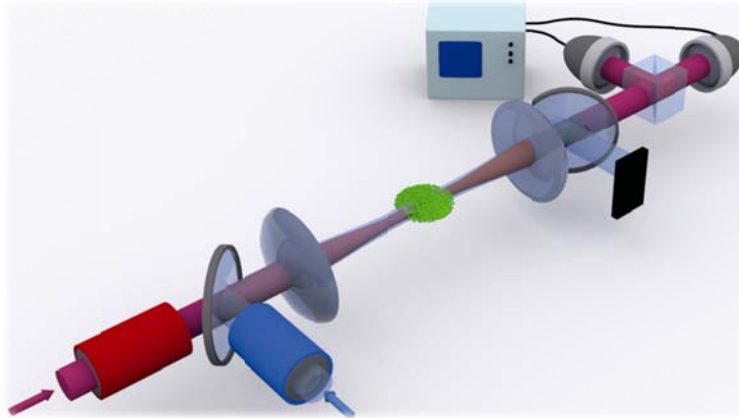
Fig. 1: Illustration of the experimental set-up: an atomic cloud (green) is held in an optical dipole trap and irradiated with light pulses from a control (blue) and a signal beam (red). Graphic: MPQ, Quantum Dynamics Division.
